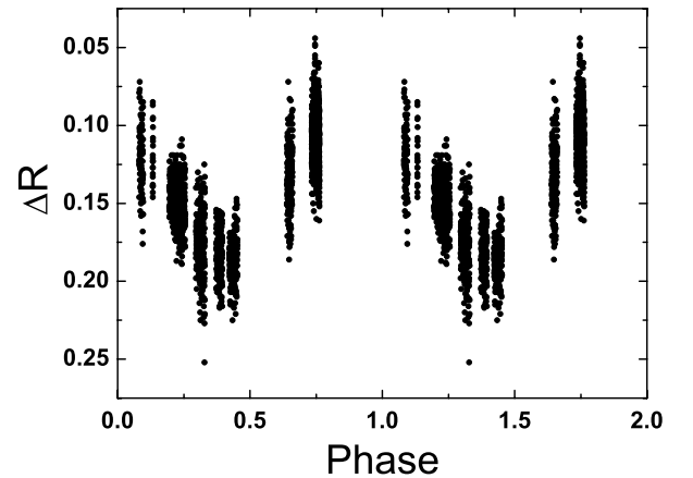
Fig. 4. Light curve of BD+20 1790 based on Terskol photometry and folded with rotational period.
