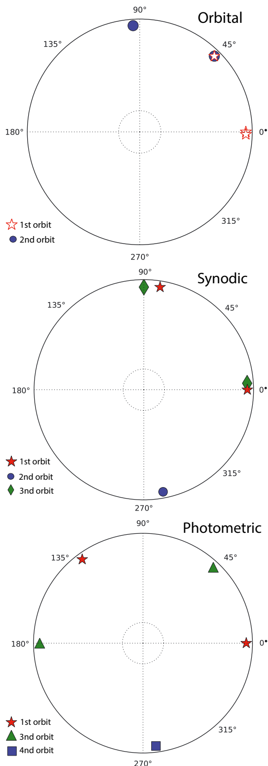
Fig. 17. Flare events for the Foces08B run. Top: phase folded orbital period. Middle: phase folded synodic period. Bottom: phase folded photometric period. The number of orbits for every period are marked with different symbols and colours, that are explained at each figure.
