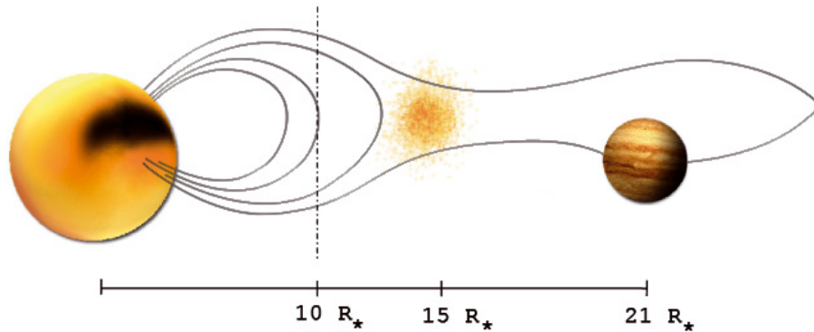
Fig. 18. Artistic impression (M. Hernán-Obispo and S. Recuero) for the BD+20 1790 system, discussed in text. The co-rotation radius is about 10 R_{\odot} , whereas the estimated height for the prominence-like structures is up to 15 R_{\odot} . The planet semi-major axis is about 21 R_{\odot} .
