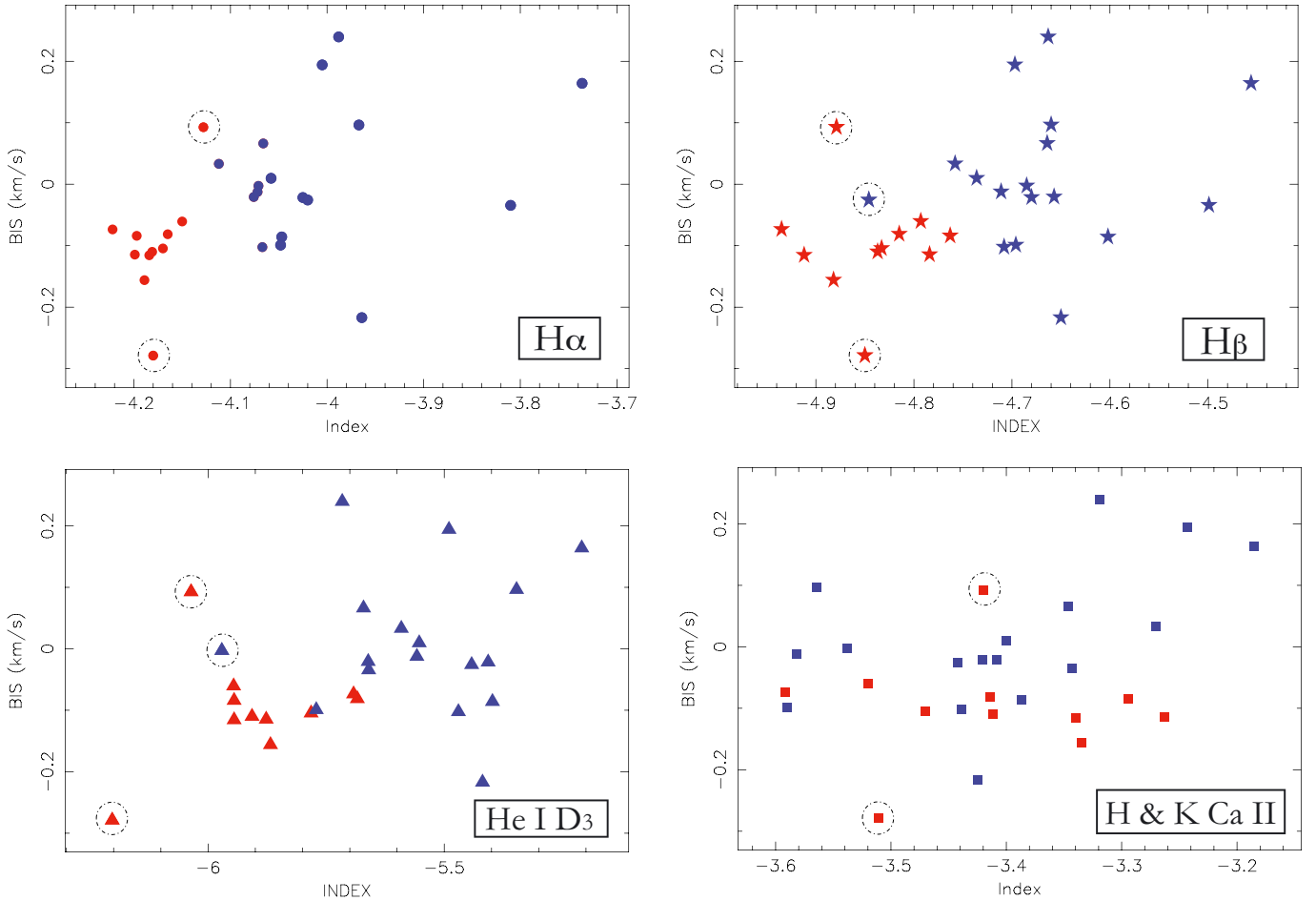
Fig. 7. Activity index vs. BIS for CORALIE data. Blue symbols represent flare affected indices. Red symbols represent the data without flare activity. Circles are for H \alpha , stars for H \beta , triangles for He I D _3 , squares for Ca II H & K. It can be seen that the scatter for the BIS is higher when a flare event occurs. Points that are marked with a dashed circle present a peculiar behaviour that is discussed in the text. Error bars for indices are about 0.001 and for BIS about 0.0001 km s ^{-1} .
