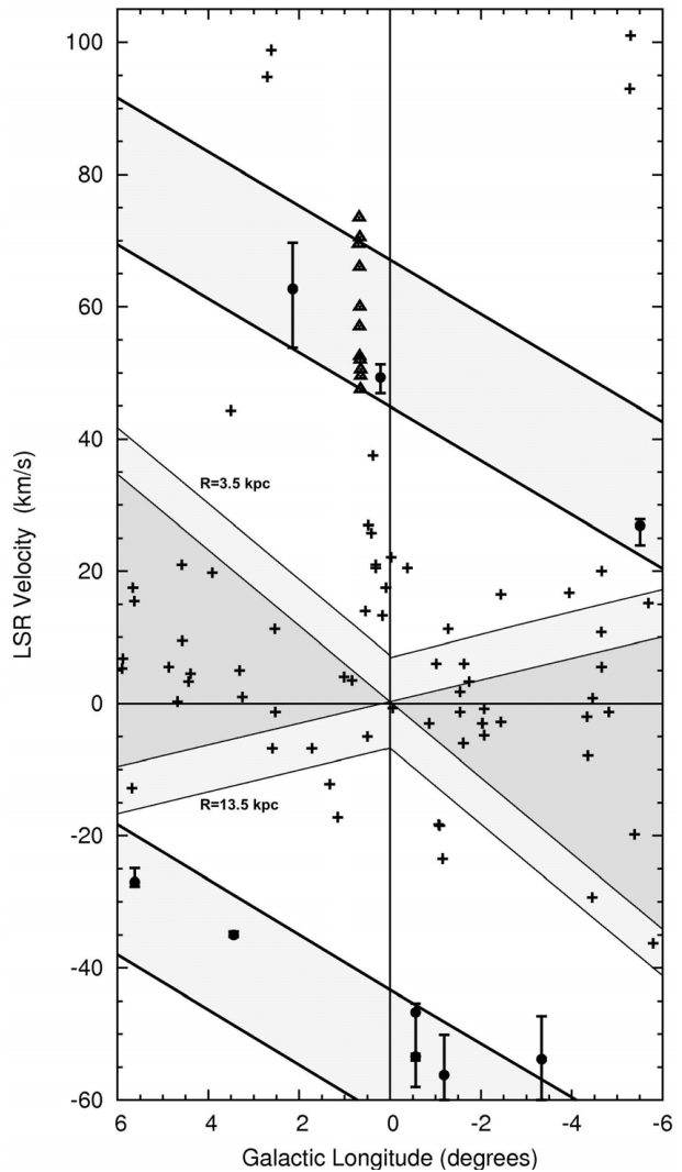
Figure 5. Longitude-Velocity plot for masers within 6 degrees of the Galactic Centre direction. Maser site symbols are crosses except for those within Sgr B2 (triangles) and nine sites attributed to the 3-kpc arm (filled circles with velocity range bars). The central wedge-shaped shaded areas are the l - v domains for sites with Galactocentric radii between 3.5 and 13.5 kpc, bounded by lighter shading to allow for small deviations from circular rotation (see text). The wide lightly-shaded parallel sloping bands near the bottom and top are the domains of the near and far sides of the 3-kpc arm. Sites within the remaining white domain are believed to lie within 3 kpc of the Galactic Centre, as discussed in the text.
