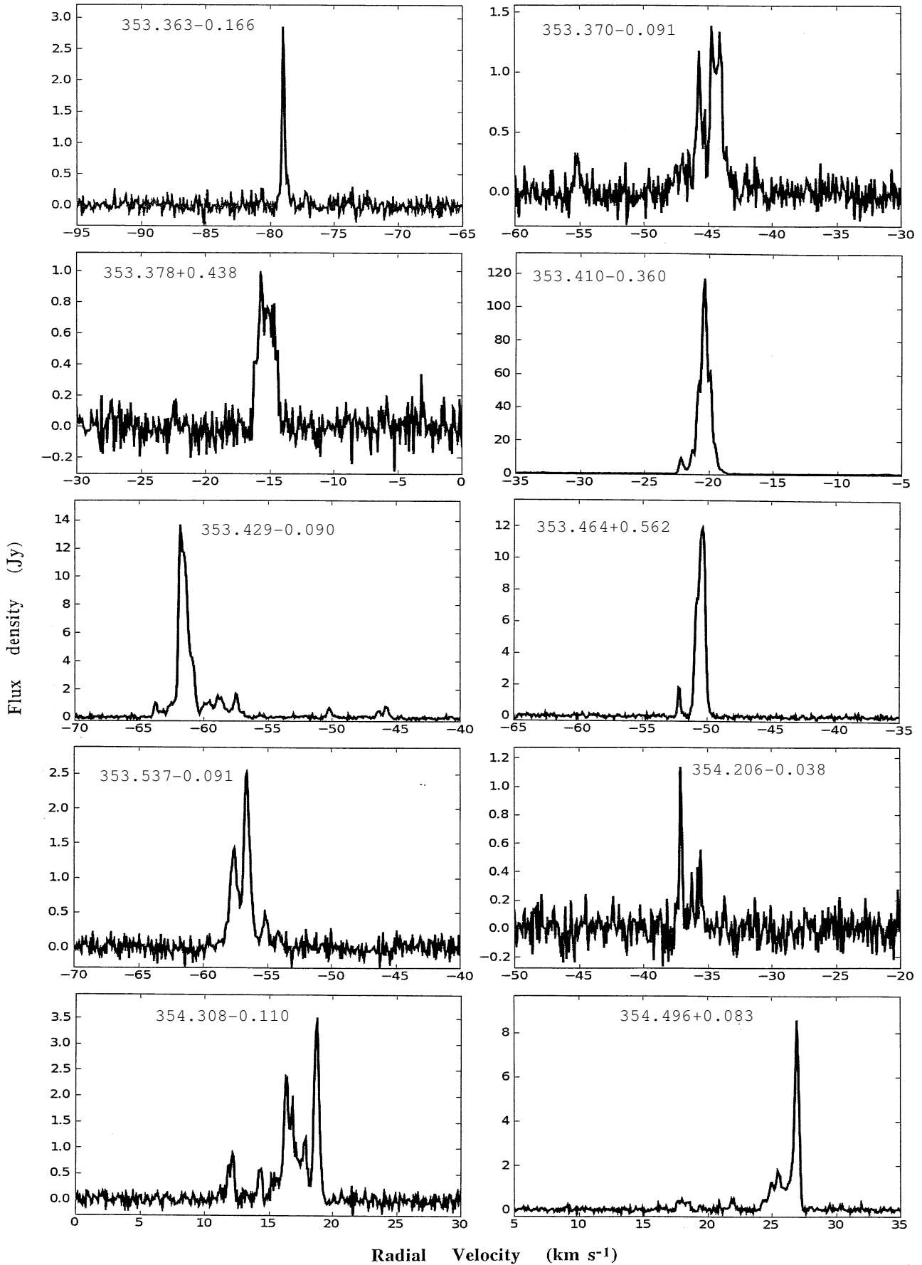
Figure 1. - continued p9 of 16
