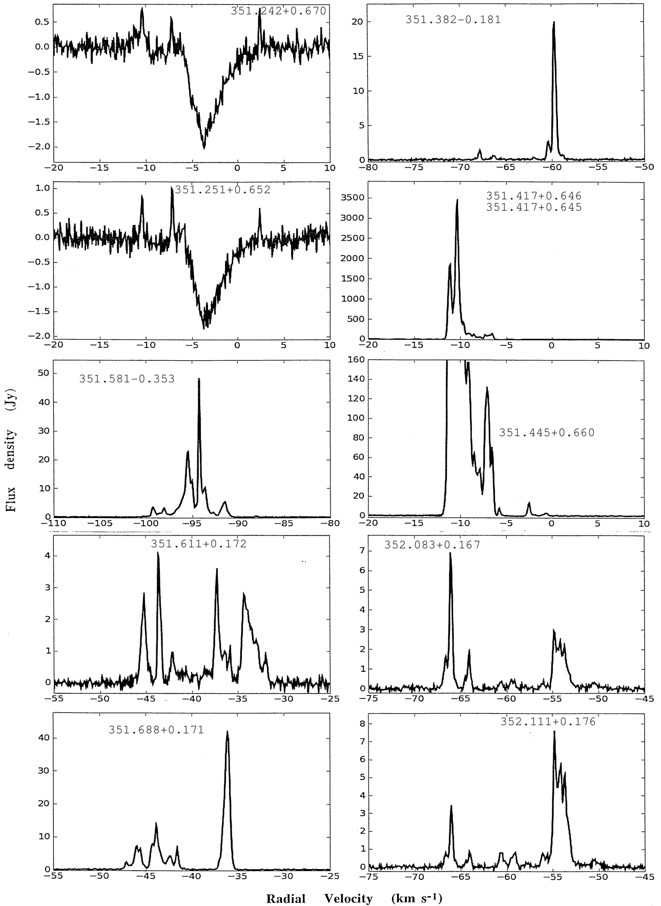
Figure 1. Spectra of 6.6-GHz methanol masers.
