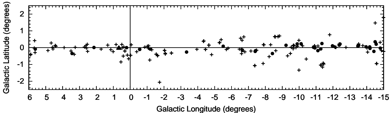
Figure 2. Distribution of the 183 methanol masers in the present survey region. Sources in the Sgr B2 complex are denoted by triangles, those believed to lie within the 3-kpc arm by circles, and the remainder by crosses.
