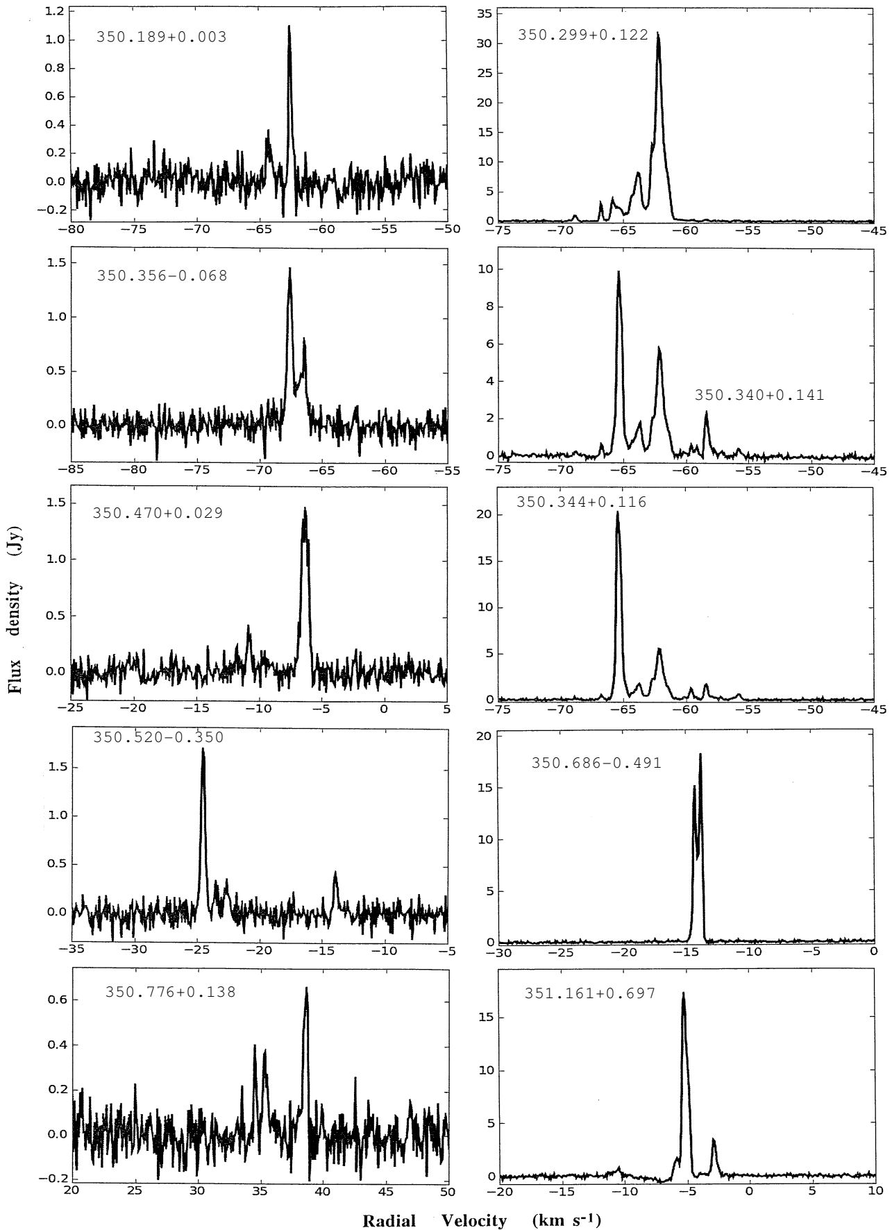
Figure 1. - continued p6 of 16
