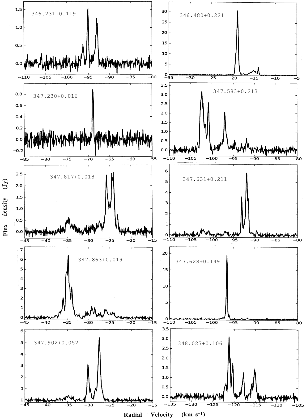
Figure 1. - continued p3 of 16
