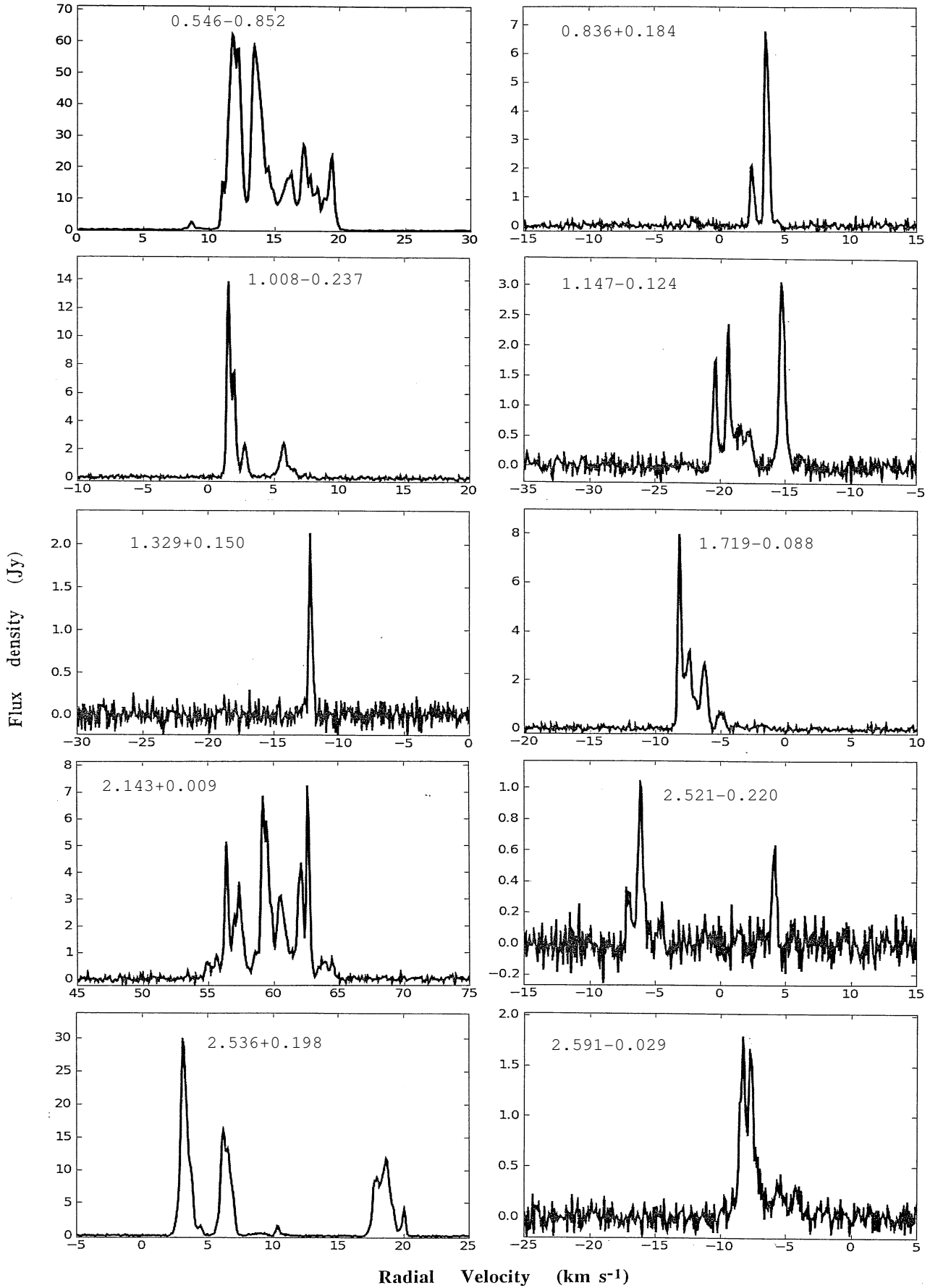
Figure 1. - continued p14 of 16
