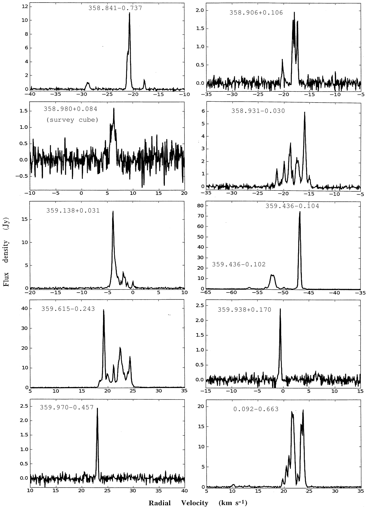
Figure 1. - continued p12 of 16
