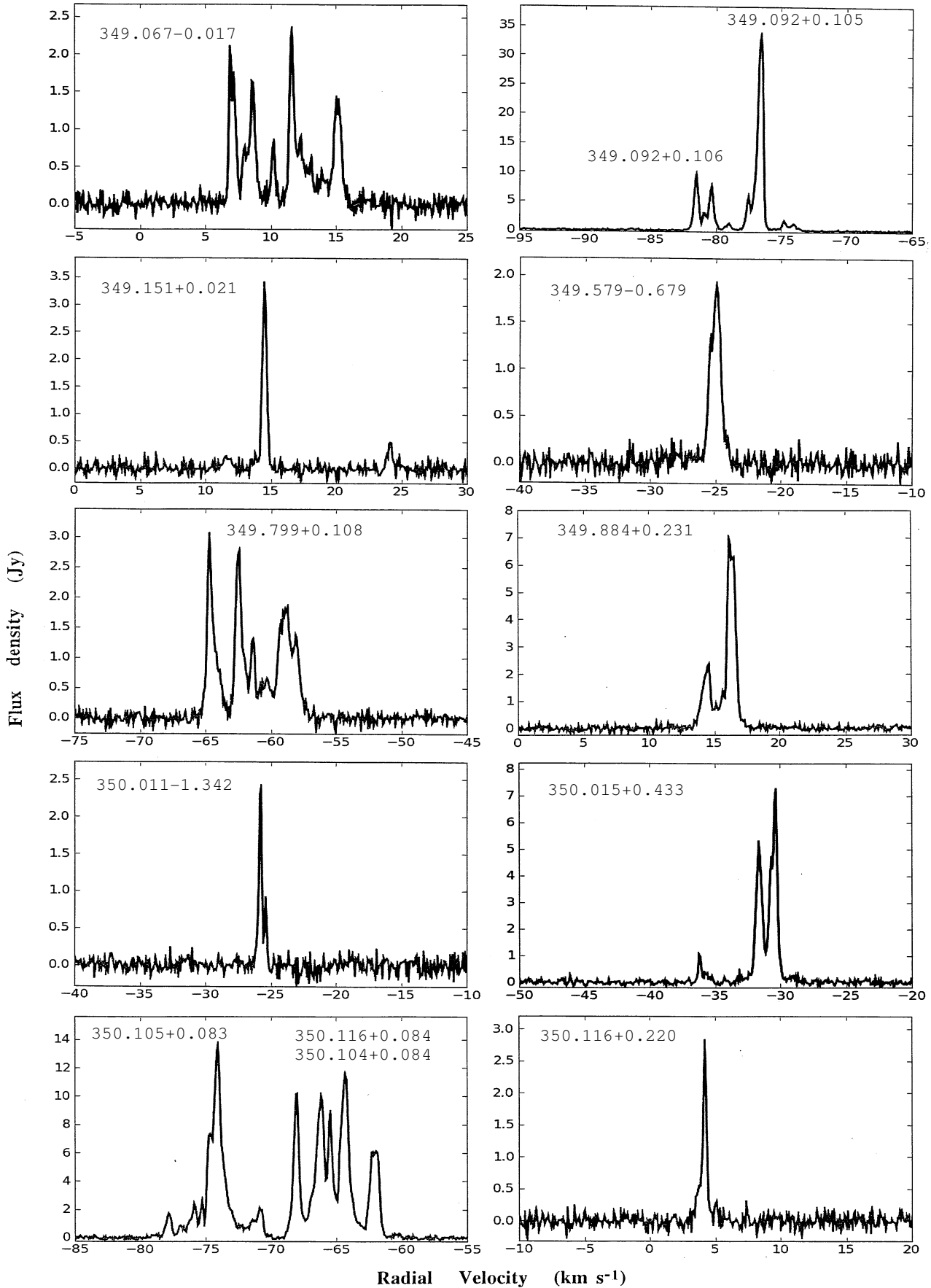
Figure 1. - continued p5 of 16
