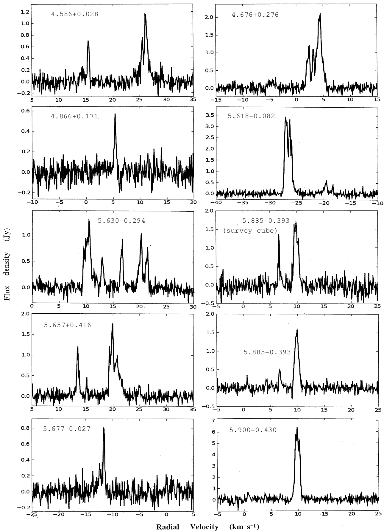
Figure 1. - continued p16 of 16
