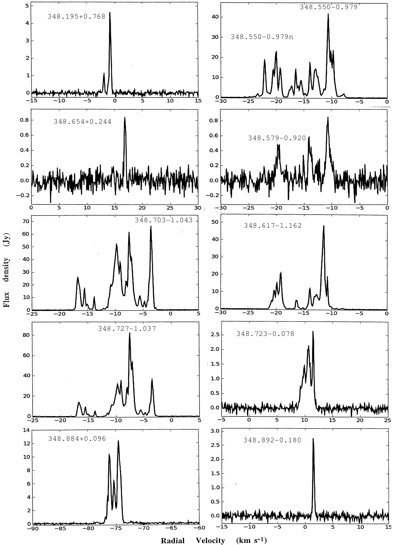
Figure 1 continued n. of 16
