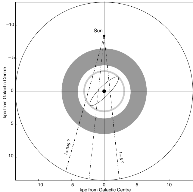
Figure 4. Plan view of the Galaxy extending to the outer boundary of detected methanol masers (Galactocentric radius 13.5 kpc). A central dot, radius 0.25 kpc, denotes the Galactic Centre Zone, a lightly shaded annulus the 3-kpc expanding arm and a shaded annulus from radius 4 to 6.5 kpc shows where high mass star formation is concentrated. An ellipse depicts the likely location of a Galactic bar. Labelled longitudes 345^\circ and 6^\circ mark the limits of the Galactic sector covered in the present survey.
