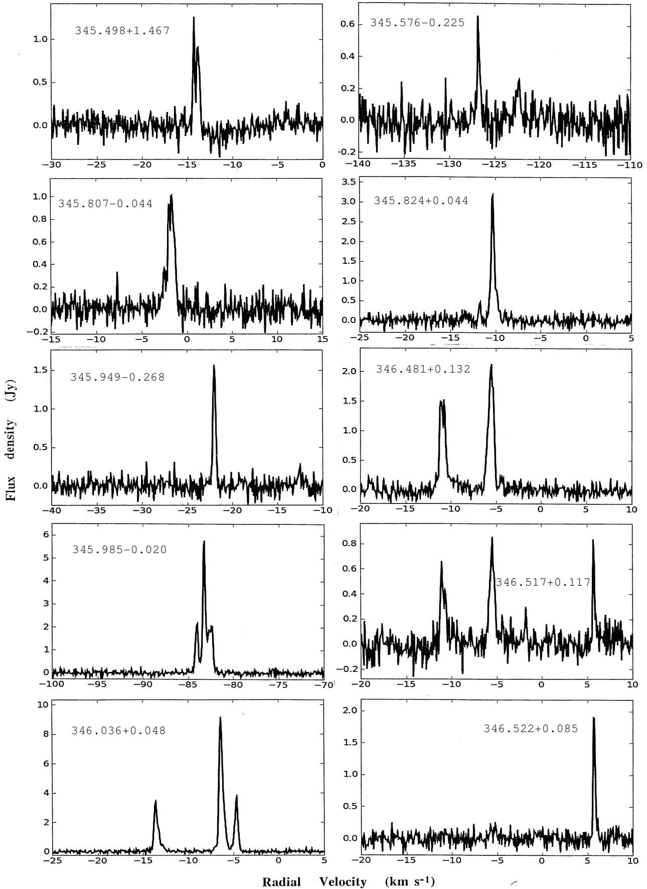
Figure 1. - continued p2 of 16
