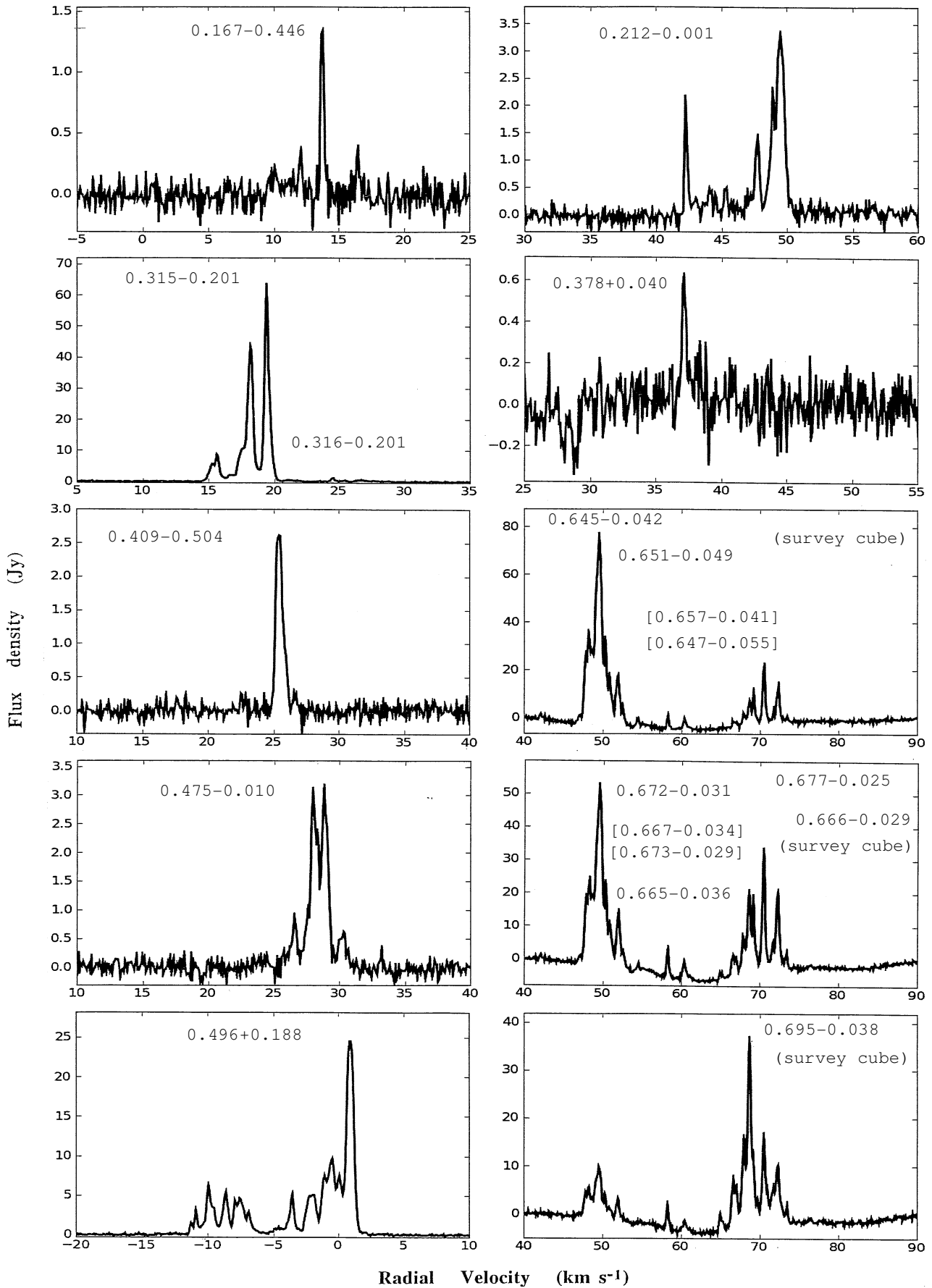
Figure 1. - continued p13 of 16
