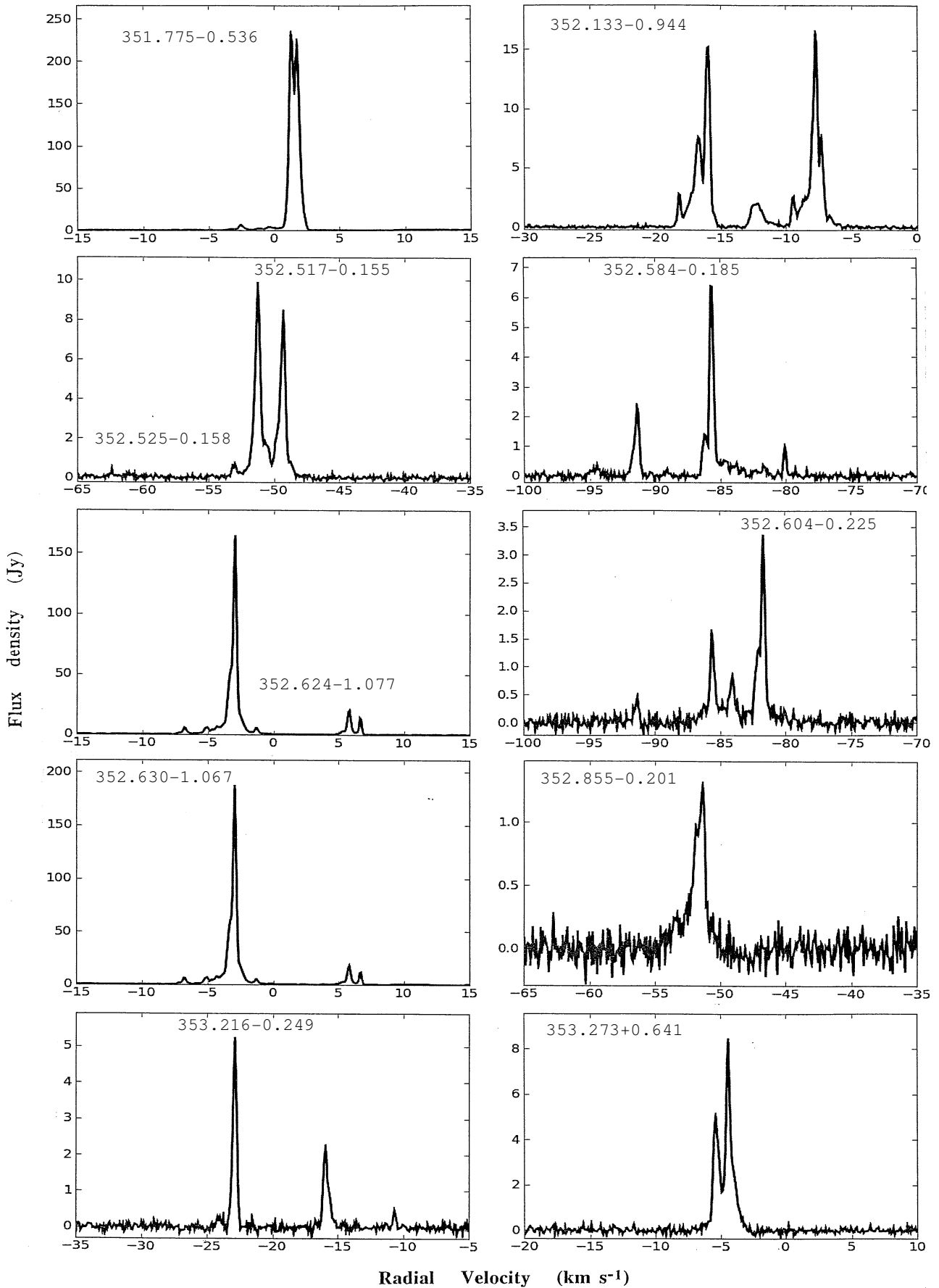
Figure 1. - continued p8 of 16
