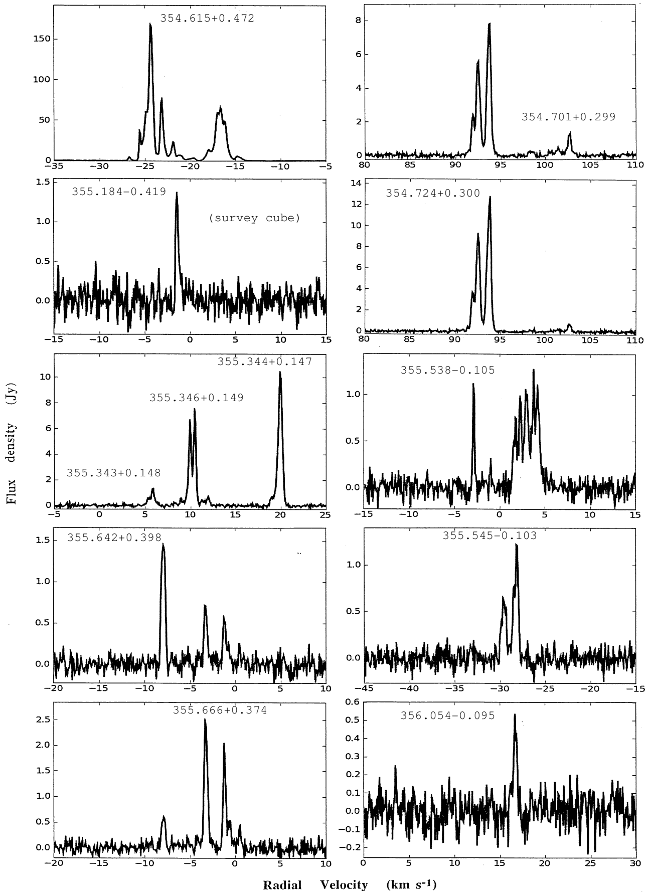
Figure 1. - continued p10 of 16
