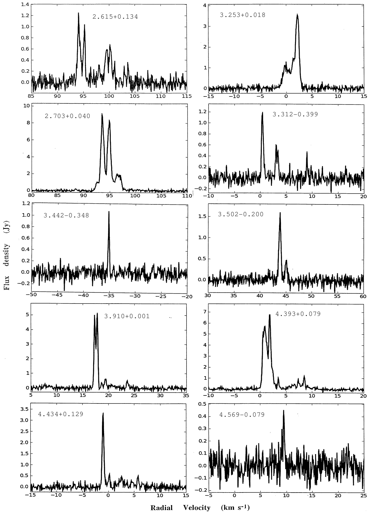
Figure 1. - continued p15 of 16
