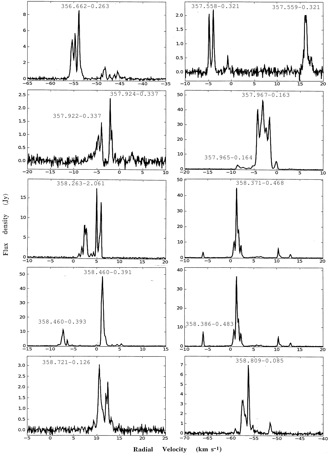
Figure 1. - continued p11 of 16
