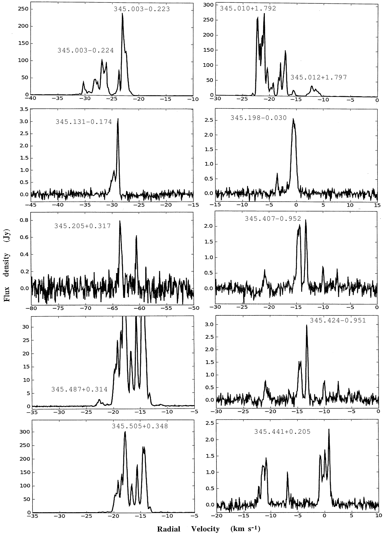
Figure 1. Spectra of 6.6-GHz methanol masers. The combined emission from nearby sites is seen in some spectra and requires reference
