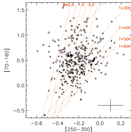
Fig. 1. Two-color diagram [70–160] vs [250–350] for the Stage 3a sources cataloged in the two investigated fields (crosses for \ell = 30^\circ , and diamonds for \ell = 59^\circ , respectively). Red dotted lines represent the loci of greybodies for various constant values of temperature and emissivity law exponent. In the bottom right corner the average error bar is reported.
