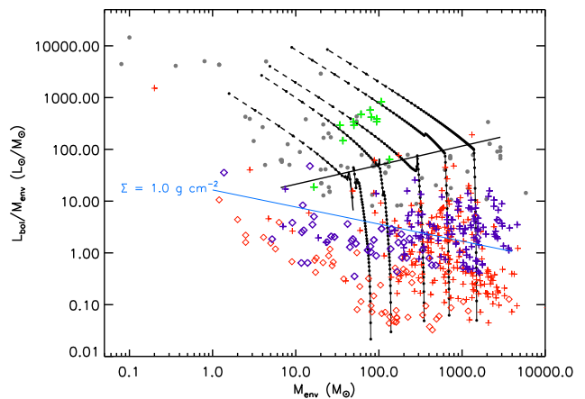
Fig. 3. L_{\text{bol}}/M_{\text{env}} vs M_{\text{env}} plot for fitted SEDs in the two investigated fields (crosses for \ell = 30^\circ , and diamonds for \ell = 59^\circ , respectively). The blue and red colors refer to fits obtained using the Robitaille et al. (2006) method (except the green points identifying models compatible with a central ZAMS star) and the greybody, respectively. The remaining grey filled circles represent the sources studied in Molinari et al. (2008) (see their Fig. 9) and are plotted for comparison. Black lines represent the models (see text); dots mark 10^4 yr intervals. The colored line represents the L/M threshold from Krumholz & McKee (2008)
