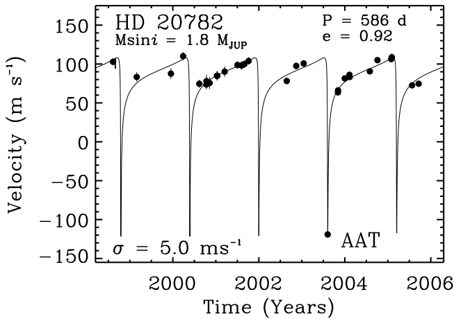
Figure 4. Doppler velocities obtained for HD 20782 from 1998 August to 2005 September. The solid line is a best fit Keplerian with the parameters shown in Table 4. The RMS of the velocities about the fit is 5.0 \text{ m s}^{-1} . Based on a primary mass of 0.95 M_{\odot} , the minimum ( M \sin i ) mass of the companion is 1.77 M_{\text{JUP}} and the semimajor axis is 1.36 \text{ au} .
