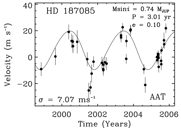
Figure 3. Doppler velocities obtained for HD 187085 from 1998 August to 2005 October. The top plot shows the best fit eccentricity, the bottom plot shows a similar quality fit for a fixed eccentricity of 0.1. In both cases the solid lines indicate the best fit Keplerian with the parameters shown.
