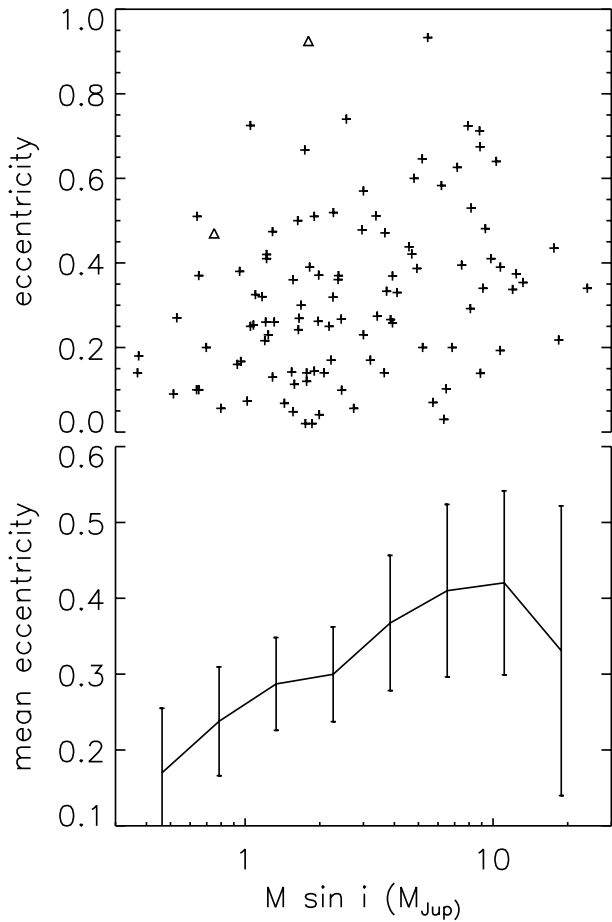
Figure 7. The upper plot shows a scatter plot for eccentricities against M \sin i / M_{\text{Jup}} for exoplanets within 200 pc with semimajor axes 0.5–10 au and masses less than 20 M_{\text{Jup}} as given by table 2 of Butler et al. (2006). The values for the exoplanets presented here are shown as triangles. The error bars are \sqrt{(\text{number})} statistics and are only indicative. The plots show results from many surveys and are thus drawn from an inhomogeneous sample.
