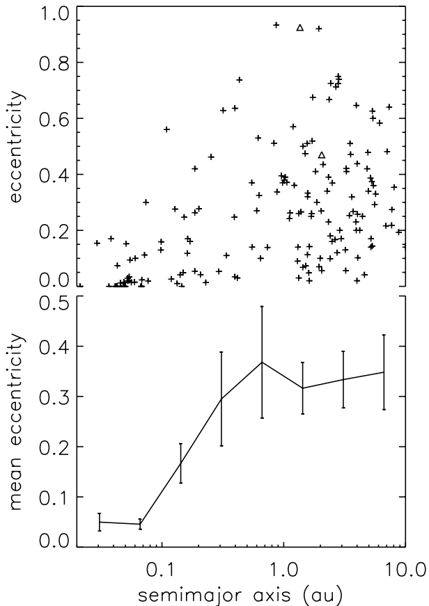
Figure 5. The upper plot shows a scatter plot for eccentricities against semimajor axis for exoplanets, within 200 pc, with semimajor axes <10 au and masses less than 20 M_{\text{Jup}} as given by table 2 of Butler et al. (2006). The values for the candidate exoplanets presented here are shown as triangles. The lower plot shows mean eccentricities plotted against semimajor axis for exoplanets. Tidal circularisation dominates the close-in planets with eccentricities reaching a plateau by around 0.2 au. The error bars are from \sqrt{(\text{number})} statistics and are only indicative. The plots show results from many surveys and are thus drawn from an inhomogeneous sample.
