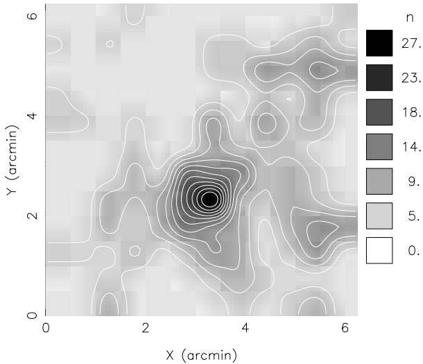
Fig. 2. Number density ( n = \text{number/square arcmin} ) of cluster galaxies selected either by (U - R)_{AB} > 3 or redshift.
