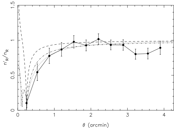
Fig. 7. Number of counts as a ratio of expected counts versus radial distance from cluster centre in the R band. Error bars account for the error in n_R and shot noise. Superimposed are the isothermal (dashes, r_{\text{crit}} = 15'' ), power-law (dot-dashes, \kappa_0 = 1.52 , \xi = 0.61 , r_{\text{core}} = 11'' ) and NFW (dots, r_s = 1.75' , \kappa_s = 0.23 ) models fit to the first 9 points.
