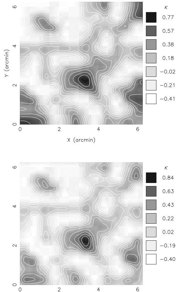
Fig. 8. Mass reconstruction from the R band data. Top : estimated \kappa from parabolic estimator. Bottom : iterated self-consistent \kappa . Contours in both plots are separated by intervals of \delta\kappa = 0.1 . North is up, East is left.
