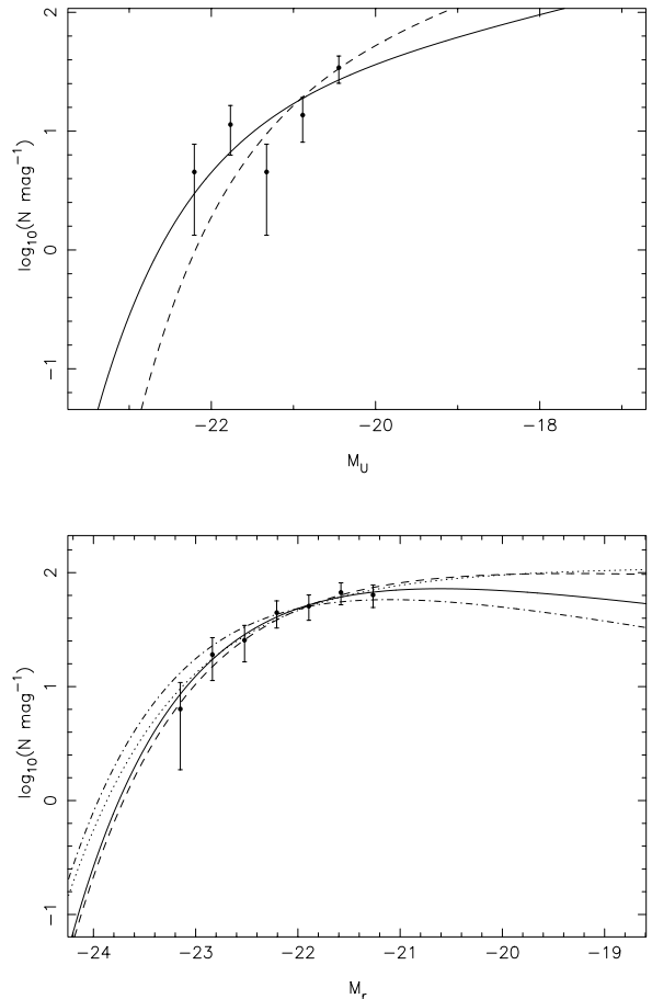
Fig. 5. Luminosity functions of CL0024+1654 galaxies. Top: U band Schechter LF from Beijersbergen et al. (2001) for the Coma cluster (dashes) and the best fit LF determined in this work (solid). Bottom: r band CCLFs for rich clusters from Paolillo et al. (2001, dots), Piranomonte et al. (2000, dashes), Garilli et al. (1999, dot-dashes) and the best fit from this work (solid).
