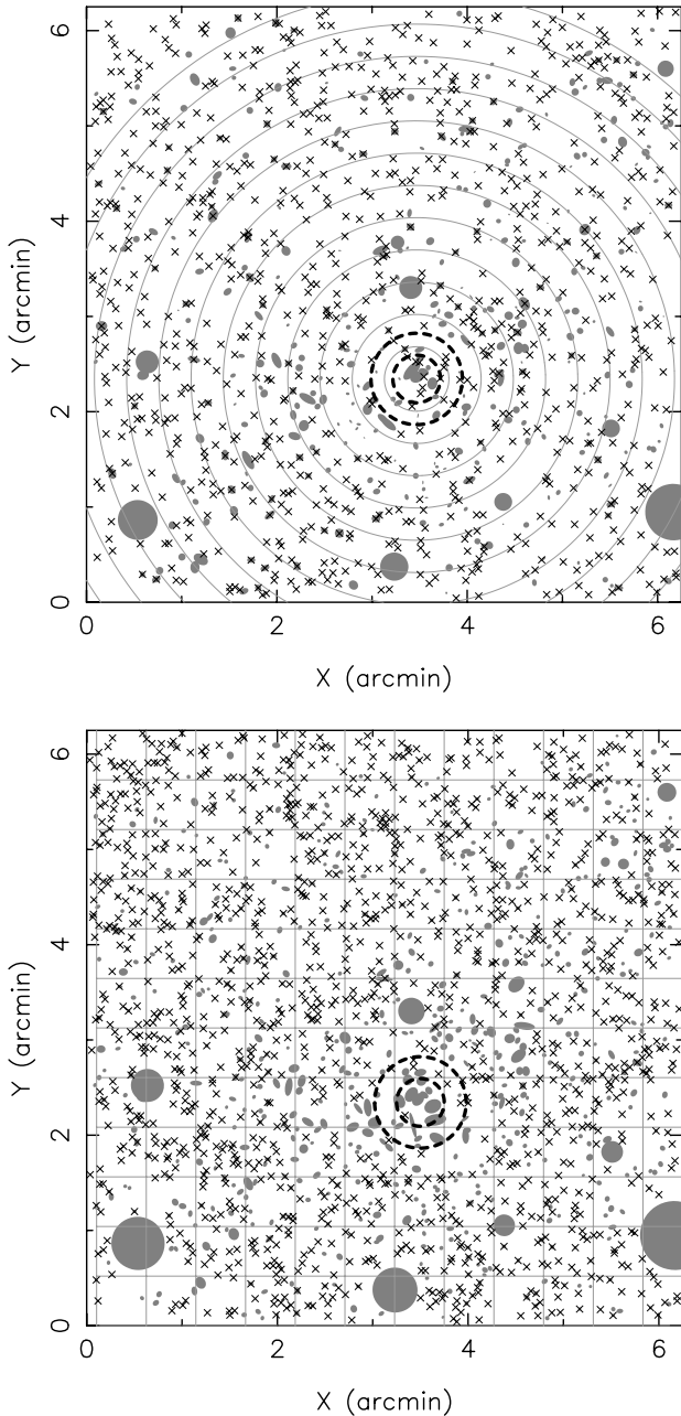
Fig. 6. Top: U band mask (grey ellipses) with source positions (black crosses) and annular bins used in Sects. 4.3 and 6. Bottom: corresponding R band mask with grid used for 2D maps in Sect. 5.1. Observed arcs lie along the outer heavy dashed circle in both plots. The inner dashed circle shows the critical line determined from the isothermal sphere model fit to the R band number counts (see Sect. 4.3).
