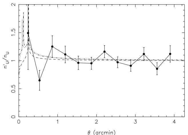
Fig. 12. Radial number count profile in the U band. Superimposed are the best fit isothermal (dashed line), power-law (dot-dashed line) and NFW (dotted line) models using the number count slope \beta_U = 1.07 . Error bars account for the error in n_U and shot noise.
