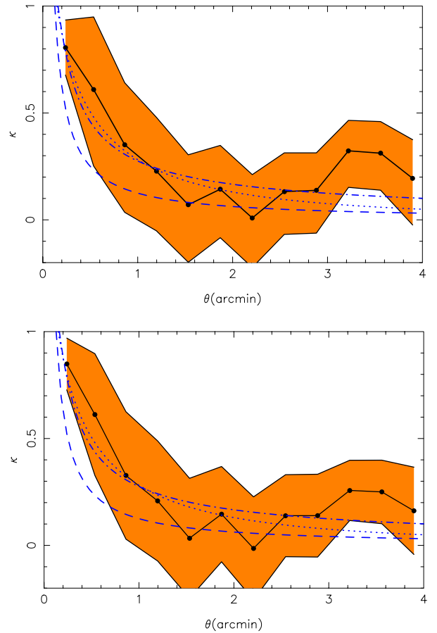
Fig. 9. Top: locally estimated radial mass profile for R band sources binned using annuli shown in Fig. 6. The shaded region shows the 1\sigma uncertainty which allows for shot noise, source clustering, uncertainty in background count normalisation and 19% cluster contamination. Bottom: axi-symmetric solution for the R band. Both plots show the isothermal (dashes), power-law (dot-dashes) and NFW (dots) models fitted to the first 9 data points (see Sect. 4.3).
