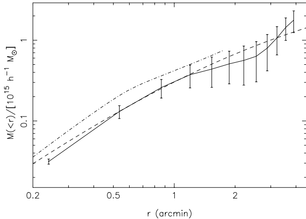
Fig. 10. Cumulative projected mass calculated by normalising to the amount of mass enclosed within the circle traced by the observed arcs. Also plotted is the NFW model of Sect. 4.3 (dashes) and the B band results of van Kampen (1998) (dot-dashes).
