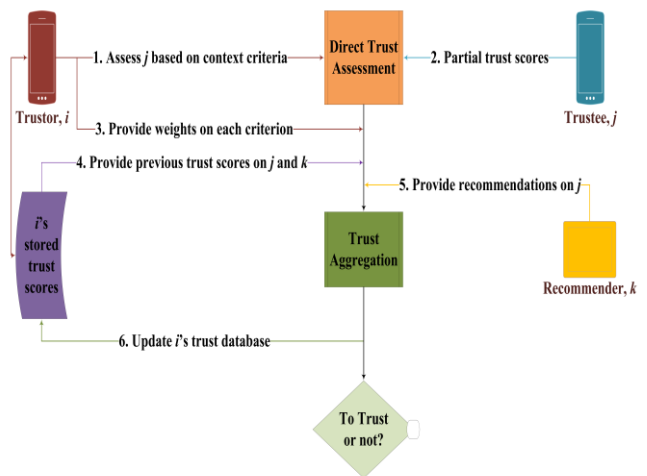
Fig. 2. Flow diagram illustrating the basic steps involved in trust computation in the CTRUST model.
