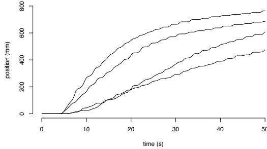
Figure 5: Progression of the robot toward the box for four values of sensitivity, (250, 500, 1000 and 2000) for curves from top to bottom respectively.
