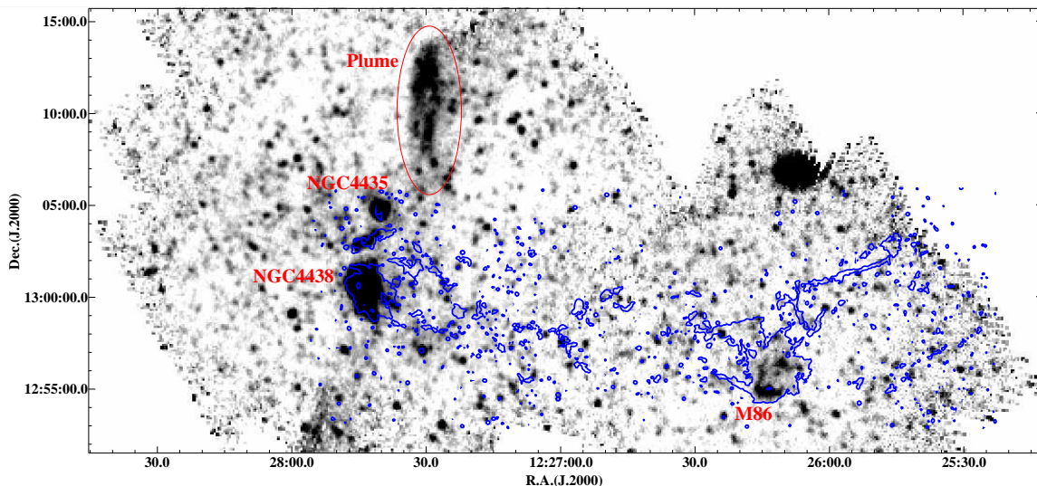
Fig. 1. The NGC4438/M86 region as seen by SPIRE. This mosaic is obtained by combining the 250\mu\text{m} maps centered on NGC4438 and M86 (Gomez et al. 2010). The blue contours show the extended \text{H}\alpha + [\text{NII}] filaments discovered by Kenney et al. (2008). Note that the intensity excess south of NGC4438 (near the edge of the frame) is just a residual of the baseline subtraction.
