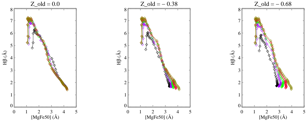
Figure 17. Composite models for different choices of the metallicity of the old component (indicated at the top of each panel) and solar metallicity of the young one represented by points in the ([MgFe50], H\beta) plane. Different colours refer to different values of the mass fraction of the young component in the composite model. The effects of age and fraction of the young component on the line-strength indices of the composite models are degenerate.
