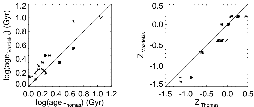
Figure 12. Comparison between the ages (left panel, in Gyr) and metallicities (right panel) obtained from our one-SSP approach using the models of Thomas et al. 2003 (horizontal axis, limitely to nearly-solar abundance ratios) and Vazdekis 1999 (vertical axis). The solid lines overplotted represent the 1:1 relation.
