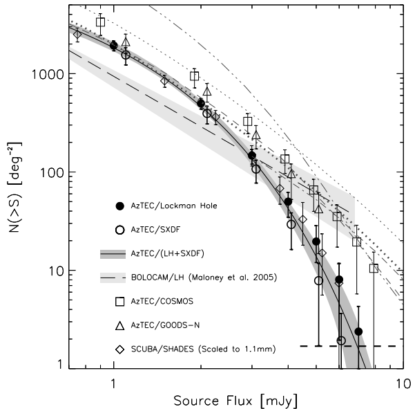
Figure 8. Integrated number counts for the AzTEC/LH and AzTEC/SXDF surveys with 68 per cent confidence intervals. Their combined constraint on the average blank-field number counts is shown as a continuous 68 per cent confidence region. A 3-parameter Schechter fit to the combined differential counts (Fig. 7) is shown as the solid curve. Results of other 1.1-mm surveys are plotted for comparison, with the AzTEC/GOODS-N and AzTEC/COSMOS results being recalculated using the AzTEC/SHADES prior and a 20 per cent null-threshold. The SCUBA/SHADES results (Coppin et al. 2006) are scaled to 1.1 mm using the combined fits of Section 4.3. Discrete integrated number counts data points are calculated at varying flux values (i.e. not shifted) for increased clarity. Model predictions are plotted as described in Fig. 7.
