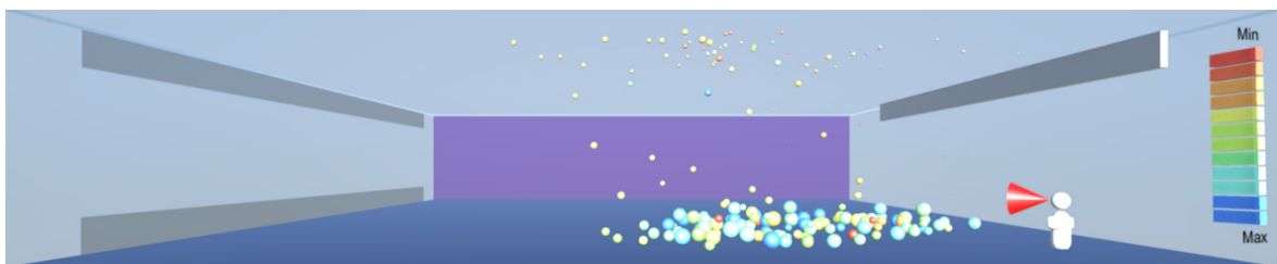
Figure 16. Uniform air velocity is started in the x direction.
