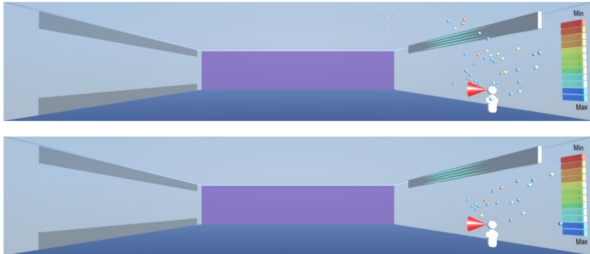
Figure 26. Overcoming the range limitation of ultraviolet radiation by driving the droplets with uniform air velocity towards the radiation source.
