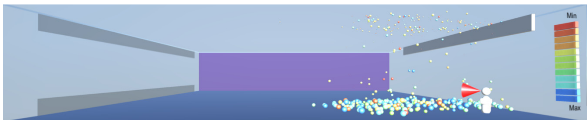
Figure 20. The combined droplets stratify so that larger particles settle near the floor and smaller particles rise towards the ceiling.
