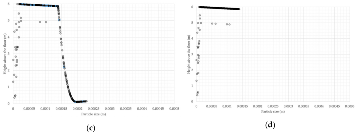
Figure 23. Particle size distribution during size reduction due to evaporation: (a) start; (b) 20% size reduction; (c) 50% size reduction; (d) 70% size reduction.
