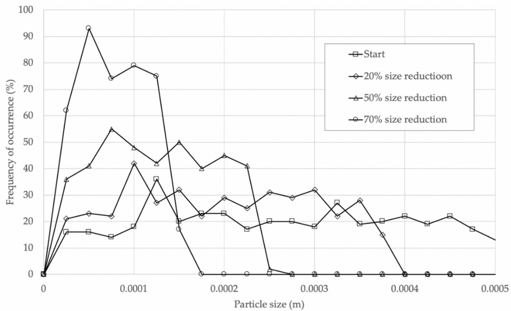
Figure 24. Distribution of particle sizes during evaporation.
