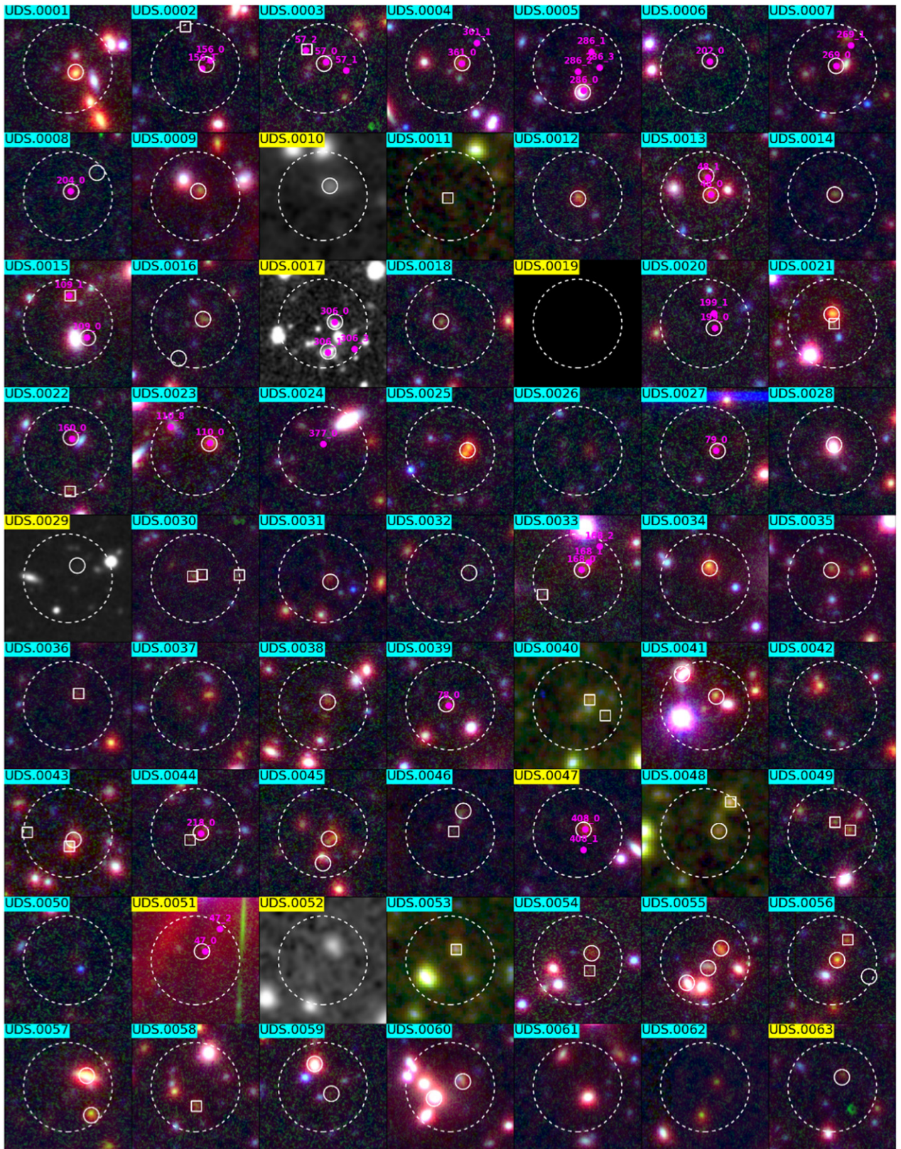
Figure 16. False-color \text{Ch1} - K - z ( r - g - b ) thumbnails (Ch2 - Ch1 - K if z band is not available) for the MAIN SCUBA-2 sources. If less than three photometric bands are available, we show in gray scale the image of the shortest among the three wavebands available. The size of each box is 25'' \times 25'' , and the large dashed circles show the counterpart searching area with a radius of 8'' . The filled squares and circles mark the counterpart candidates identified through the OIRTC technique and radio imaging, respectively. We only show circles if sources are identified by both radio and OIRTC. The magenta points are ALMA-detected SMGs with the ID numbers adopted from Simpson et al. (2015b). The background color for each ID number shows the Class of each source, with cyan, yellow, and brown marking Class = 1, 2, and 3, respectively (matched to the color scheme adopted in Figure 2). (An extended version of this figure is available.)
