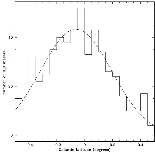
Figure 12. Galactic latitude distribution of H 2 O masers detected in HOPS. The number of water masers is shown by the histogram and a fitted Gaussian to the distribution is shown as the dashed line. The fitted Gaussian has a peak at -0.062^\circ and FWHM of 0.60^\circ .
