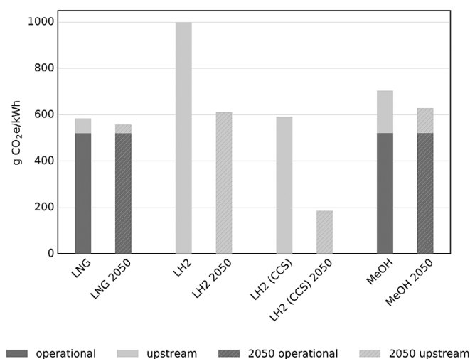
Fig. 6. Impact of temporal assumptions on life-cycle emissions summarised in Table 3, measured in g CO 2 e per kWh shaft output.
