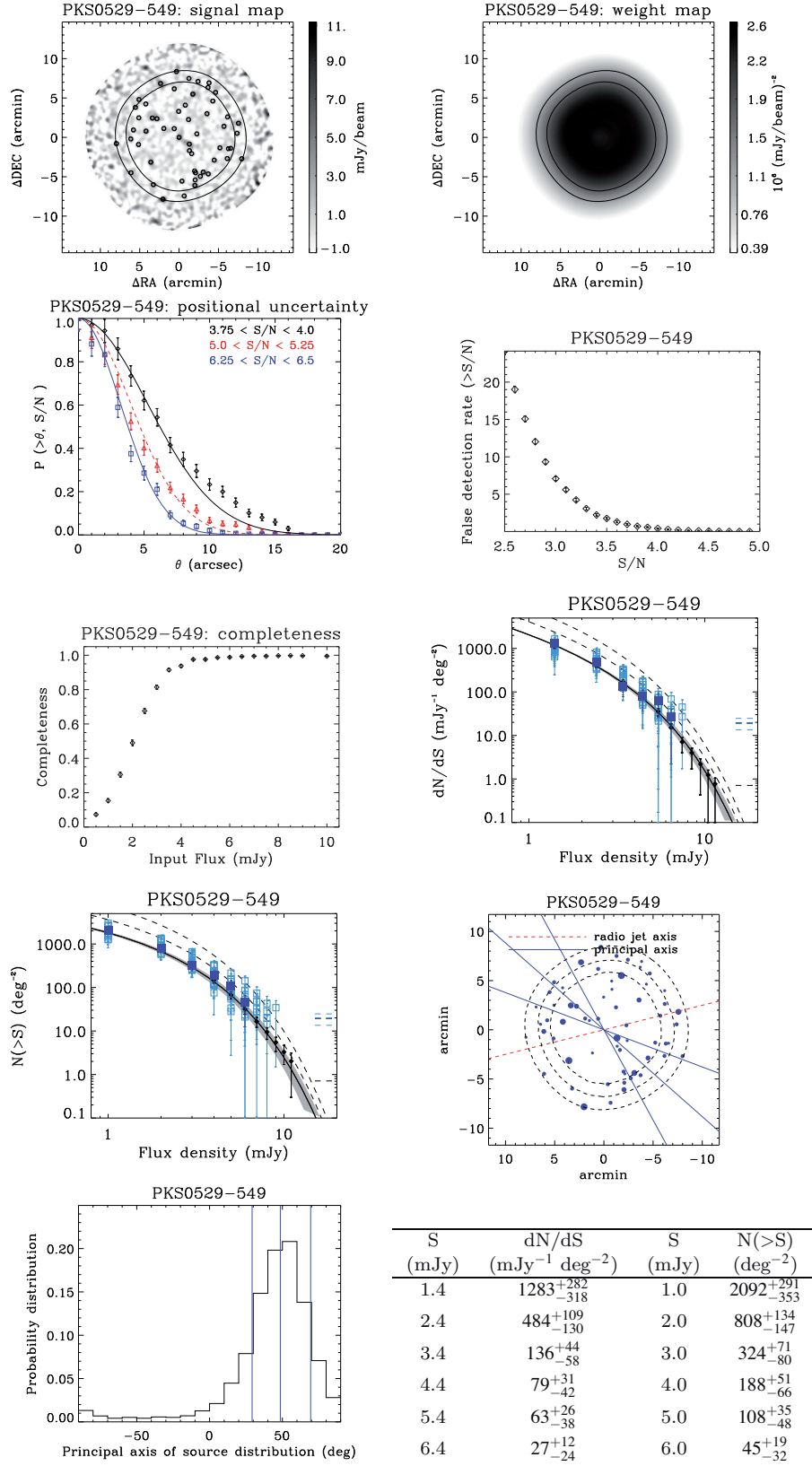
Figure A8. PKS0529-549 products.
