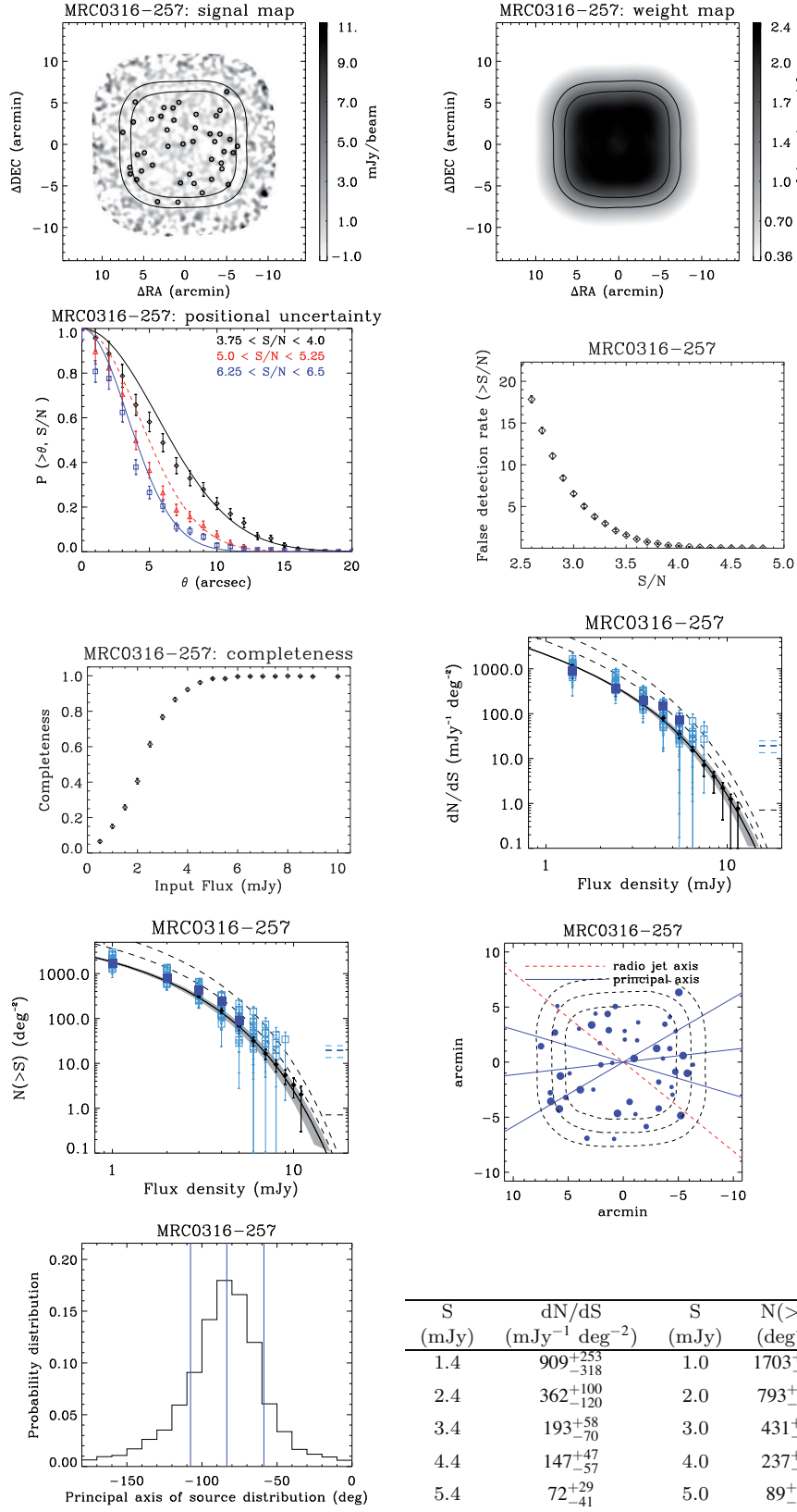
Figure A7. MRC0316-257 products.
