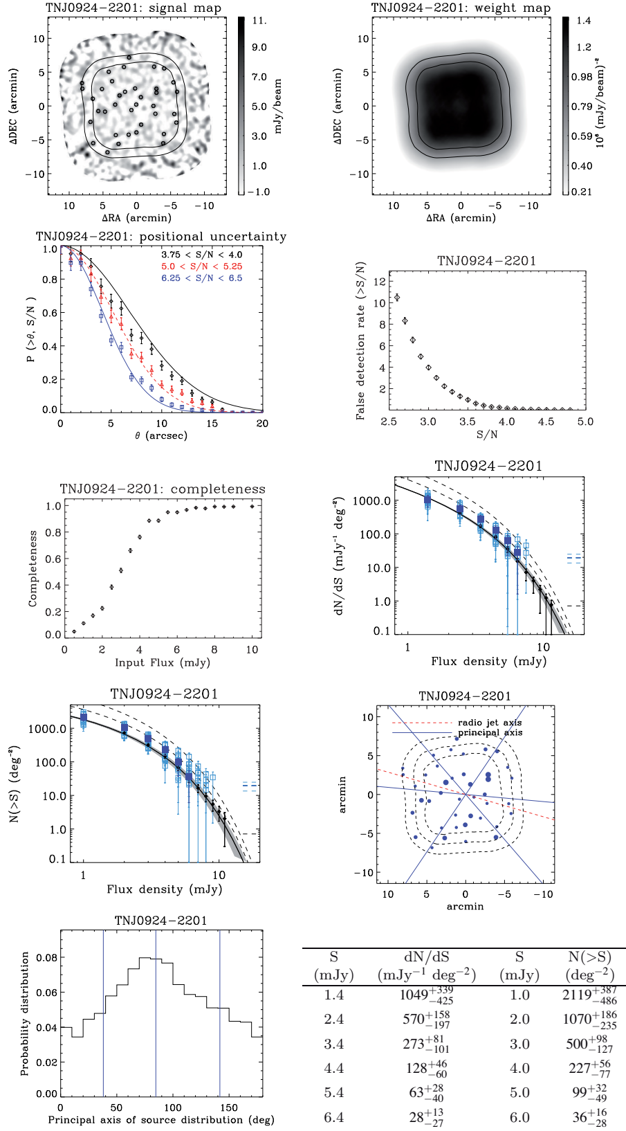
Figure A2. TNJ0924-2201 products.
