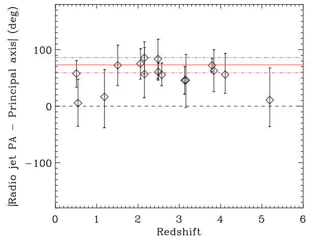
Figure 14. Angular difference (absolute value) between the RG jet and the principal axis of the surrounding source distribution for the 16 ACES RG fields, plotted against redshift. In most cases, the radio jet direction and the principal axis are separated more than 45 deg, although the error bars are quite large. A similar analysis using all fields is performed in Section 6.3. The result is plotted as solid and dotted–dashed horizontal lines.
