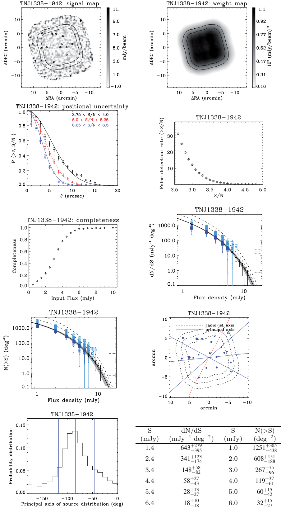
Figure A3. TNJ1338-1942 products.
