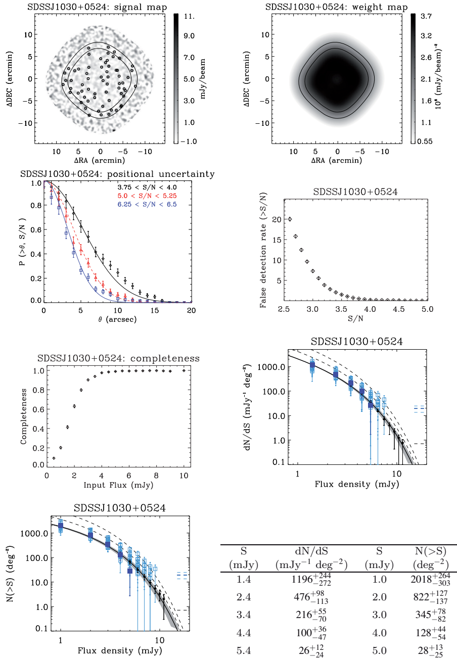
Figure A1. SDSSJ1030+0524 products.
