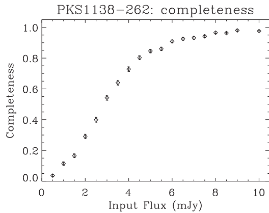
Figure 4. Completeness estimation for AzTEC sources in the ACES protocluster field towards PKS1138–262. The data points and 68 per cent confidence binomial error bars show the completeness estimated by inserting sources of known flux density one at a time into the real signal map. From the image, it can be seen that for sources with flux densities >4 mJy the completeness is >60 per cent. According to noise properties of the PKS1138–262 map, sources with S/N > 3 have flux densities >2.1 mJy.
