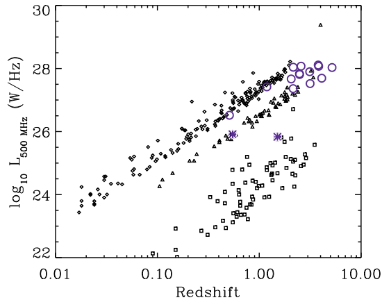
Figure 1. Radio luminosity–redshift ( L_{500\text{MHz}}-z ) plane for radio surveys 3CRR (diamonds; Laing, Riley & Longair 1983), 6CE (triangles; Eales 1985; Rawlings, Eales & Lacy 2001), and LBDS (squares, Lynx and Hercules fields only; Rigby, Snellen & Best 2007), which have successively deeper flux-density limits. These radio luminosities were calculated using a typical spectral index of 0.8 (de Zotti et al. 2010). Open circles denote ACES RGs whose synchrotron self-absorption frequency appears to be at <500 MHz (rest frame). Asterisks denote the 2 GPS sources we include in our sample. ACES AGN luminosities were estimated by fitting a straight line or a parabola to their spectra, depending on the number of data points available.
