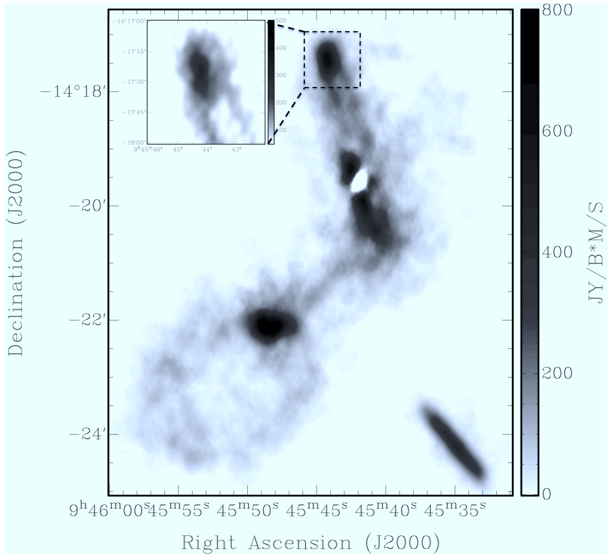
Figure 8.7: Spatial distribution of the integrated HI flux in Arp 245 (Natural weights, 11''.66 \times 7''.92 resolution). A robust-weight map ( 7''.17 \times 4''.76 resolution) of the spatial distribution of the integrated HI in the TDG Arp 245N is also displayed in the top left corner of the figure. Note the two “branches” in the north tail. They correspond to different parts of the tidal tail along the line-of-sight. Thanks to the high spatial resolution of the data, we are able to disentangle them.
