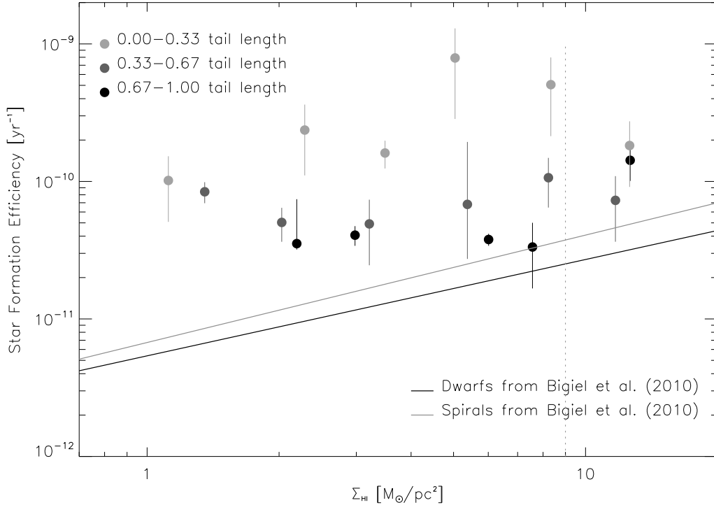
Figure 9.14: SFE-HI relation, per bin of \Sigma_{HI} and distances to the central galaxy. The SFE is defined as \Sigma_{SFR}/\Sigma_{HI} . Filled circles correspond to the median SFE (corrected for extinction) and mean \Sigma_{HI} within each bin. The error bars represent the statistical dispersion within each bin. When the statistical dispersion is greater than the median value, the lower error bar corresponds to [median - min value]. When the bins contain only one value, the statistical dispersion is taken to be half of the SFE. The solid lines are power-law fits to the distributions of spirals and dwarfs of Bigiel et al. (2010). In both cases, the slope is \sim 0.7 . Estimates of the SFE take into account the contribution of helium (factor of 1.34).
