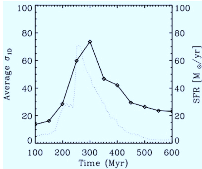
Figure 7.1: Evolution of the SFR and the velocity dispersion of the gas in a simulation of a galaxy merger (Bournaud et al., in prep.).
