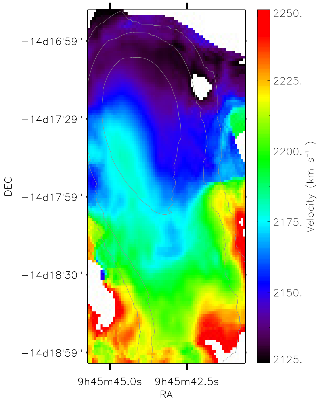
Figure 8.10: (a) Spatial distribution of the integrated H I velocity in Arp 245. Note the overall velocity gradient along the tidal tails. The rotation of the South West companion can be clearly seen. (b) Spatial distribution of the H I velocity around the TDG Arp 245N, delimited by the dotted rectangle in panel (a). In both figures, density contours at 1.5 M_{\odot} \text{pc}^{-2} , 4.0 M_{\odot} \text{pc}^{-2} and 9.0 M_{\odot} \text{pc}^{-2} of a 30'' resolution map have been overlaid in grey.
