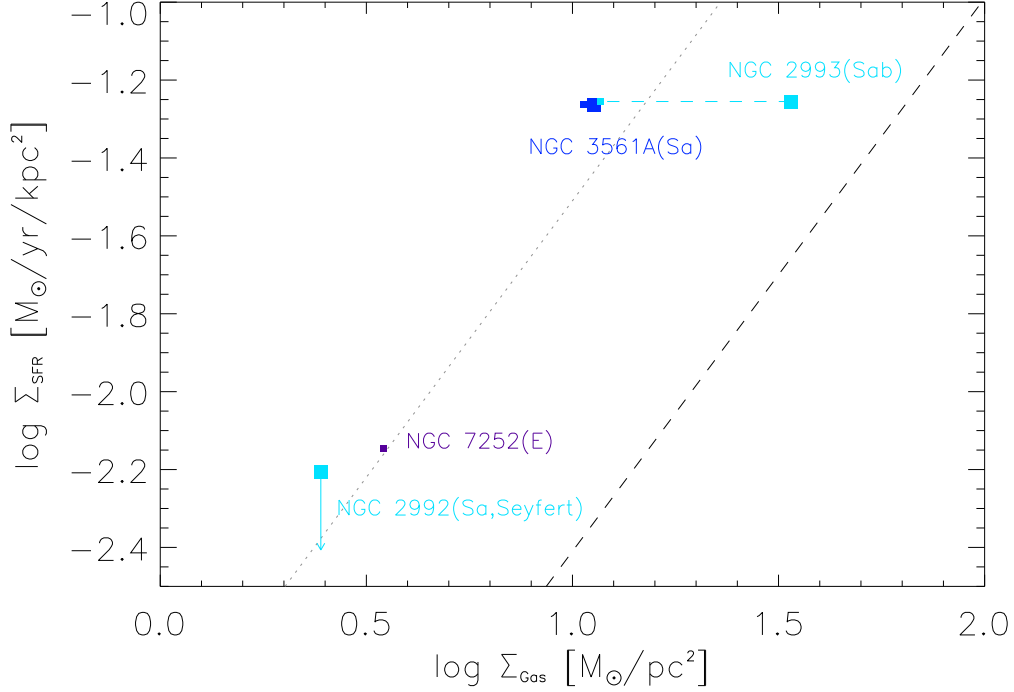
Figure 9.4: Location of the interacting systems on the SK-relation. The integrated values of the total gas, HI+H 2 plus helium contribution (large squares), the molecular gas, H 2 plus helium contribution (small squares), and SFR within R_{25} are plotted. The dashed line shows the locus of regular star-forming galaxies, whereas the dotted line corresponds to the starburst sequence, as defined by Daddi et al. (2010b) .
