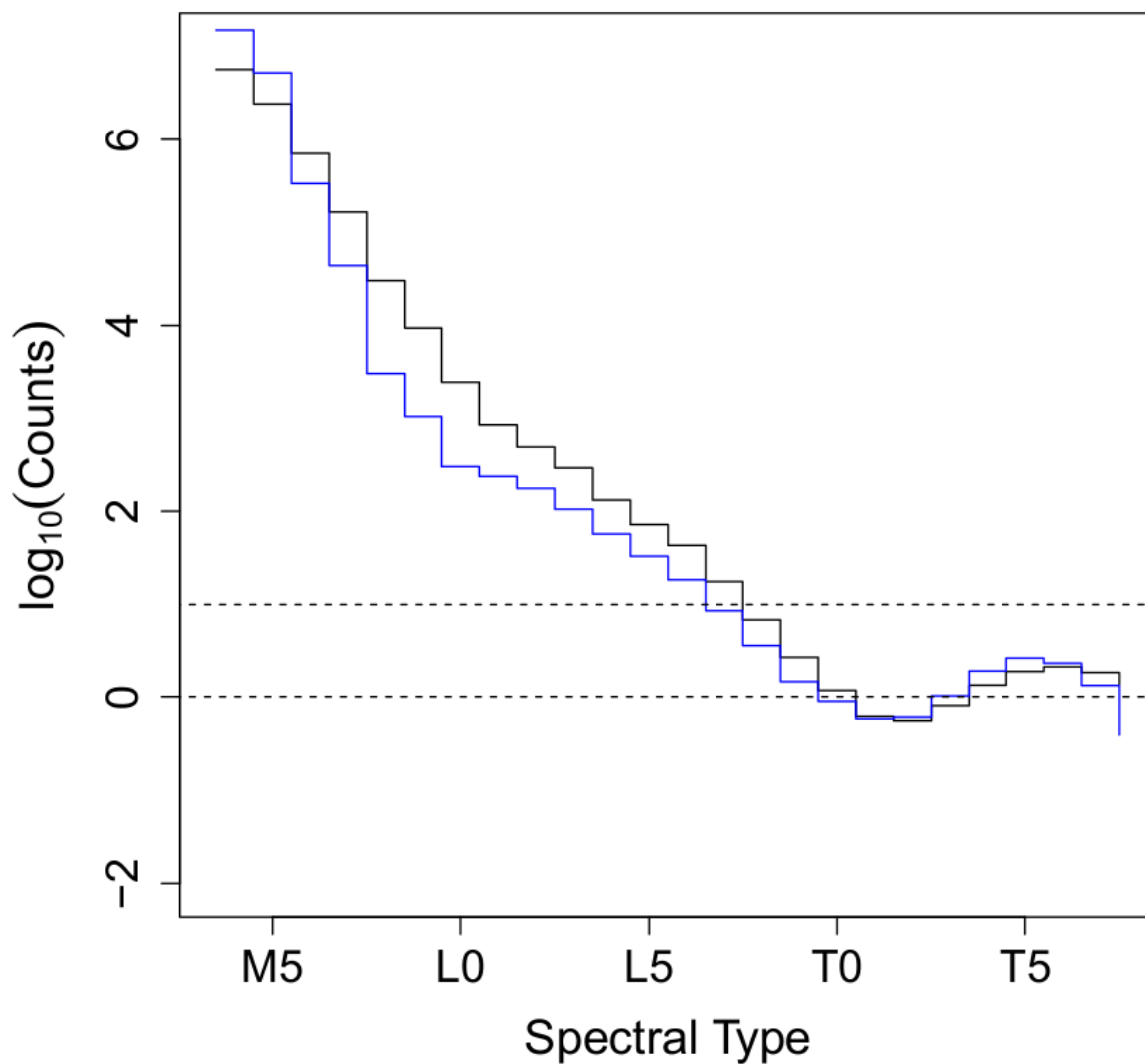
Figure 6.6: Figure from Sarro et al. (2013) showing the predicted number of counts per spectral type bin for Gaia, the black line represents the data from Caballero et al. (2008), where a spectral type and an I-band relationship is used. The blue line represents the data from the BT-Settl model (Allard et al., 2012). Dashed lines indicate 1 and 10 detection counts. For further details see Sarro et al. (2013).
