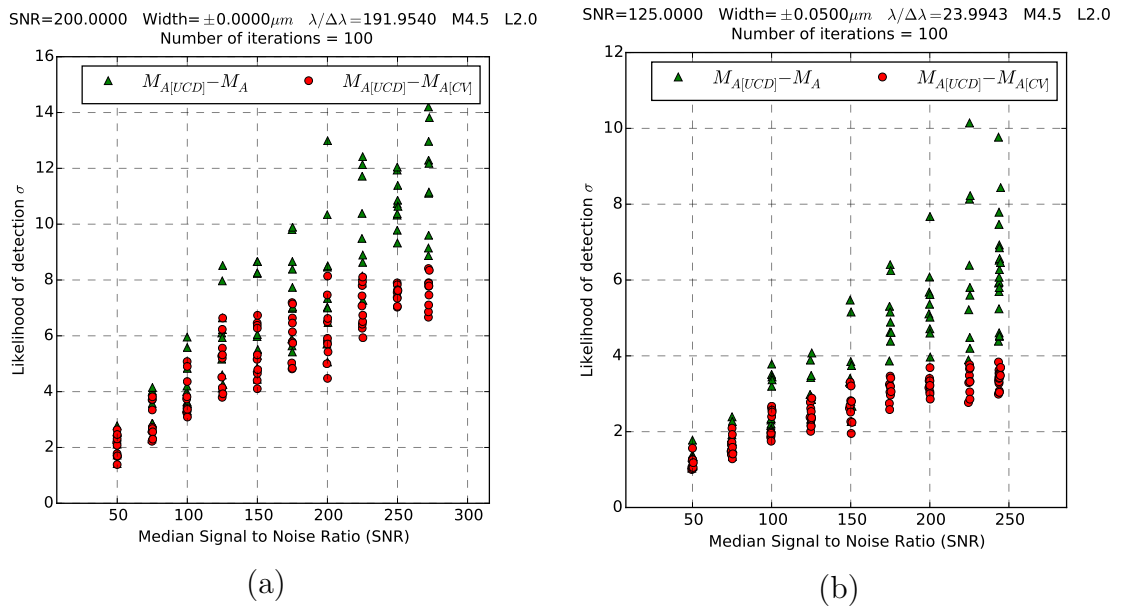
Figure. 4.20: How likelihood of detection changes across simulated SNR, for (a) ideal case (b) minimal case. Green triangles are the ideal case ( M_{A[UCD]}-M_A ) and red circles are the simulated colour-variants ( M_{A[UCD]}-M_{A[CV]} ). The spectral difference simulation process was repeated multiple times for each set of parameters (SNR, Width, resolution and primary/secondary spectral type) to minimise over-favourable noise and colour-variant situations.
