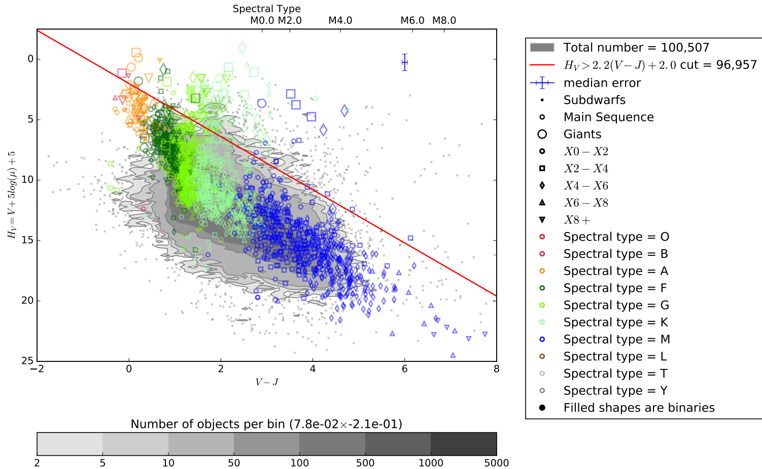
Figure. 2.5: The reduced proper motion cuts applied to a small area of sky ( \alpha = 9^h20^m0.0^s, \delta = +30^\circ0^m0.0^s to \alpha = 10^h0^m0.0^s, \delta = +40^\circ0^m0.0^s ) to show the size of the reduced proper motion cut. Spectral type is calculated using Equation 2.2. This shows that the vast majority of sources are kept using this cut but the brightest slow moving sources are rejected as possible giant stars or background galaxies. Over plotted on my distribution is a sample from the Gliese and 2MASS Cross Identifications Catalogue by Stauffer et al. (2010) to show that this cut truly selects dwarf stars and the giant stars are clearly seen as rejected. Difference shapes represent the different spectral subtypes, different sizes represent sub-dwarfs, main sequence and giant stars, colours represent different spectral classes.
