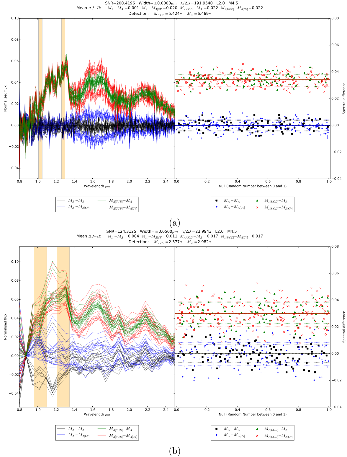
Figure. 4.19: (a) Spectral difference plot, left panel is the spectral subtractions ( M_{A-A} , M_{A[UCD]-A} , M_{A-A[CV]} , and M_{A[UCD]-A[CV]} ) for various noise-variants and colour-variants. Right panels shows the calculated spectral difference for each distribution (Equation 4.29). The parameters of SNR, width of the spectral band, resolution, L dwarf spectral type and M dwarf spectral type are shown above each figure. Mean colours were calculated for the four distributions and likelihoods were calculated as in Equation 4.30. (b) Parameters were chosen as the minimum required to achieve a \sim 2\sigma detection while giving the shortest possible exposure time (lower SNR).
