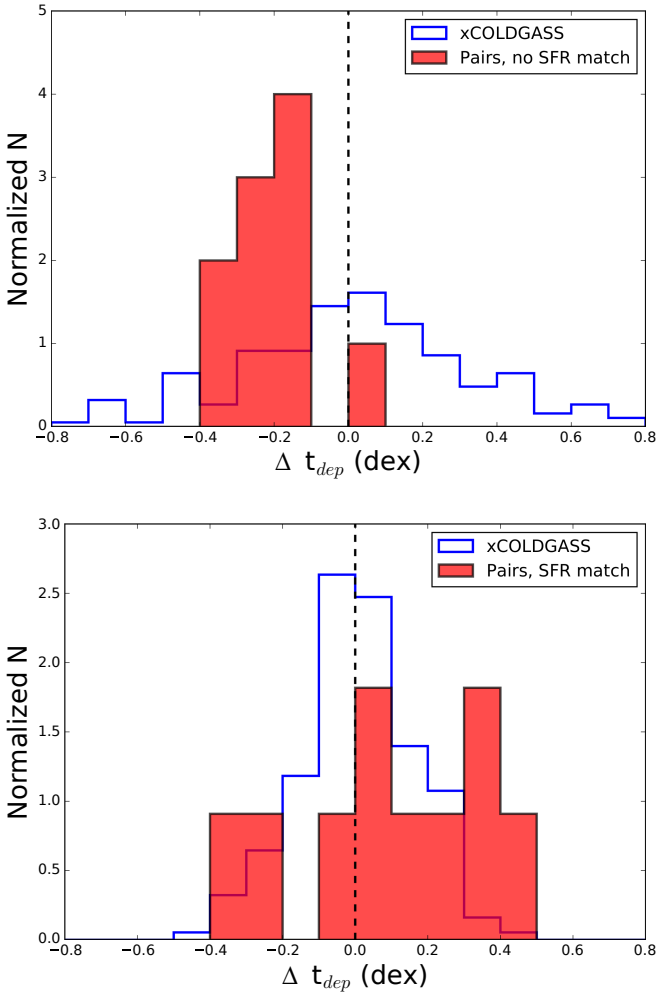
Figure 6. Molecular gas depletion time offset distribution of galaxy pairs (red filled histogram) and xCOLDGASS sources (blue empty histogram).
