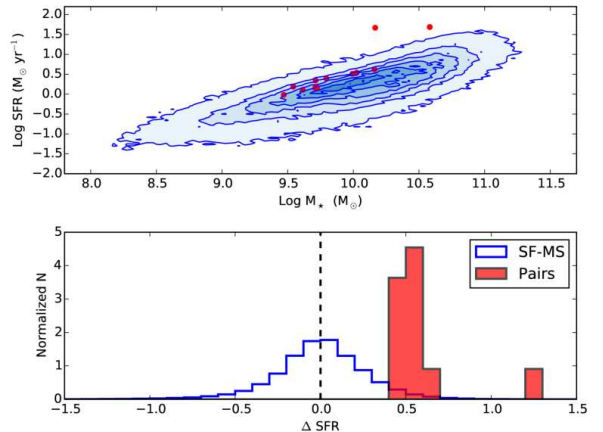
Figure 1. Top panel: Comparison between the main-sequence of SDSS star-forming galaxies (blue contours, as classified by Kauffmann et al. 2003) and our sample of 11 galaxies in pairs (filled red circles). Stellar masses and total SFRs of both samples are taken from Mendel et al. (2014) and Brinchmann et al. (2004), respectively. Bottom panel: Distribution of the SFR offset of galaxies in pairs compared to the main sequence, which reveals enhanced star formation activity in our sample of 11 galaxy pairs. The procedure used to produce this plot is fully described in Ellison et al. (2016) and is summarized in Section 2.
