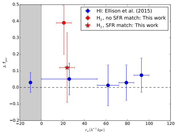
Figure 7. Distribution of the mean neutral gas fraction offset ( \Delta f_{gas} ) as a function of projected separation. The blue circles are the pairs and post-merger galaxies from Ellison et al. (2015), whereas the red symbols represent the mean H_2 fraction offsets of the 11 galaxy pairs of this paper (red points are slightly offset on the x-axis for clarity). The method employed to calculate the H_2 fraction offset is identical to that described in section 4.4.
