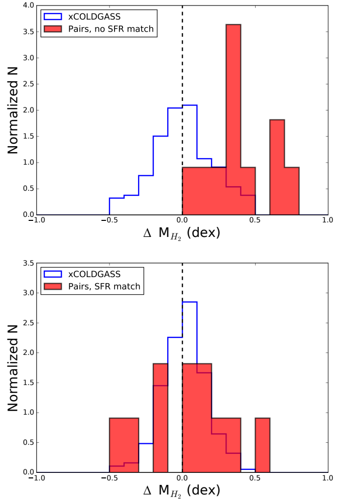
Figure 5. Distribution of molecular gas mass offset. Our sample of galaxy pairs is represented by the filled red histogram, whereas the xCOLDGASS sample distribution is plotted as a blue histogram.
