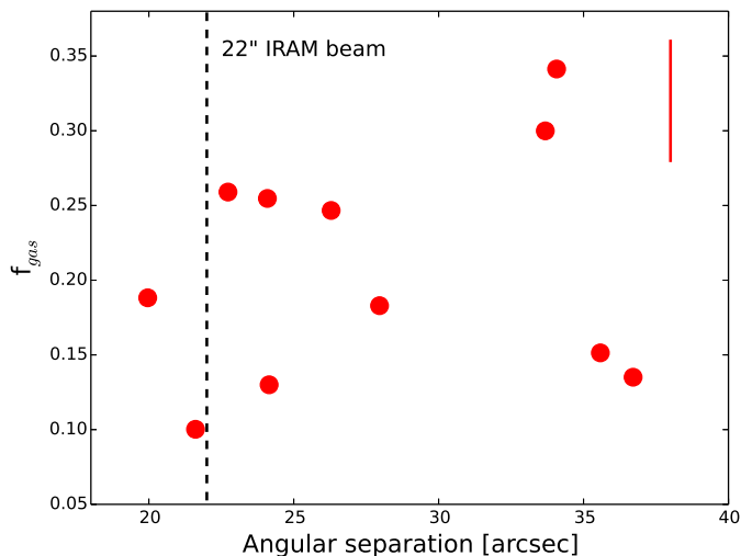
Figure 9. Molecular gas fraction vs angular separation between the two component galaxies comprising each pair in our sample. The black dashed line indicates the FWHM of the IRAM 30m beam at 3 mm. The red vertical bar represents the average error on gas fraction of our sample. The majority of the sources lie above this limit, and together with the lack of correlation between the plotted quantities, suggests that our CO measurements do not suffer from contamination from gas emission of the pair companion.
