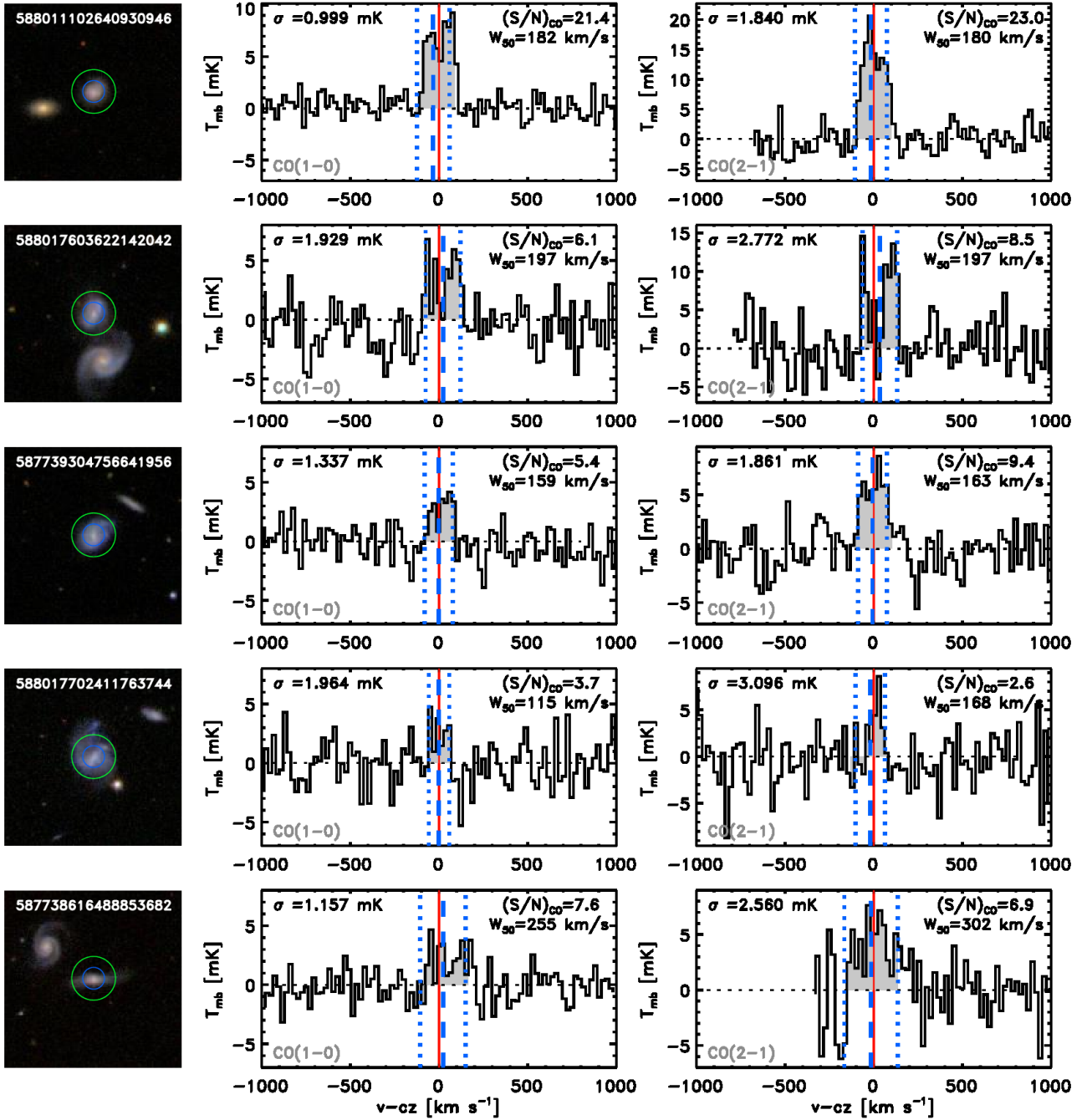
Figure 2. SDSS cutout images of the 5 galaxy pairs in our sample and their corresponding CO(1-0) (left) and CO(2-1) spectra (right). The green and blue circles in the images represent the FWHM size of the IRAM 30-m beam of 22 and 11 arcsec, respectively. In each spectrum the red dashed line represents the systemic redshift of the source, as determined from the SDSS spectrum. The dashed blue line is the central velocity of the CO line, while the blue dotted line delimits W_{50\text{CO}} , i.e. the linewidth of the CO emission measured at half intensity.
