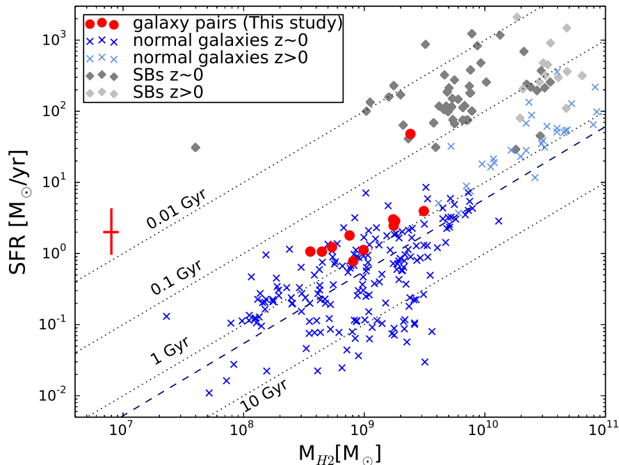
Figure 8. SFR plotted as a function of the molecular gas mass M_{H_2} . Our 11 galaxies in pairs are represented as red circles, while normal star-forming galaxies and starbursts are blue crosses and grey diamonds respectively. For both literature samples the dark symbols are local/low-redshift galaxies. The red cross reproduces the average error on M_{H_2} and SFR of our sample. For reference we show lines of constant gas depletion time. The dashed blue line is the best fit to the normal galaxies; with galaxy pairs lying above this sequence (with an average offset \leq 1\sigma ) as a result of their enhanced SFE.
