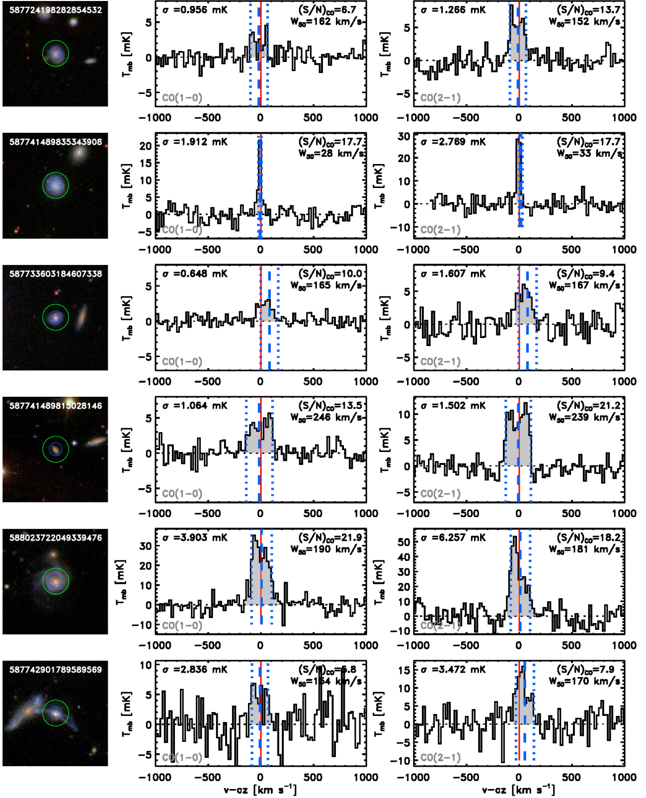
Figure 3. SDSS cutout images of the remaining 6 galaxy pairs in our sample and their corresponding CO(1-0) (left) and CO(2-1) spectra (right). Details as in Figure 2.
