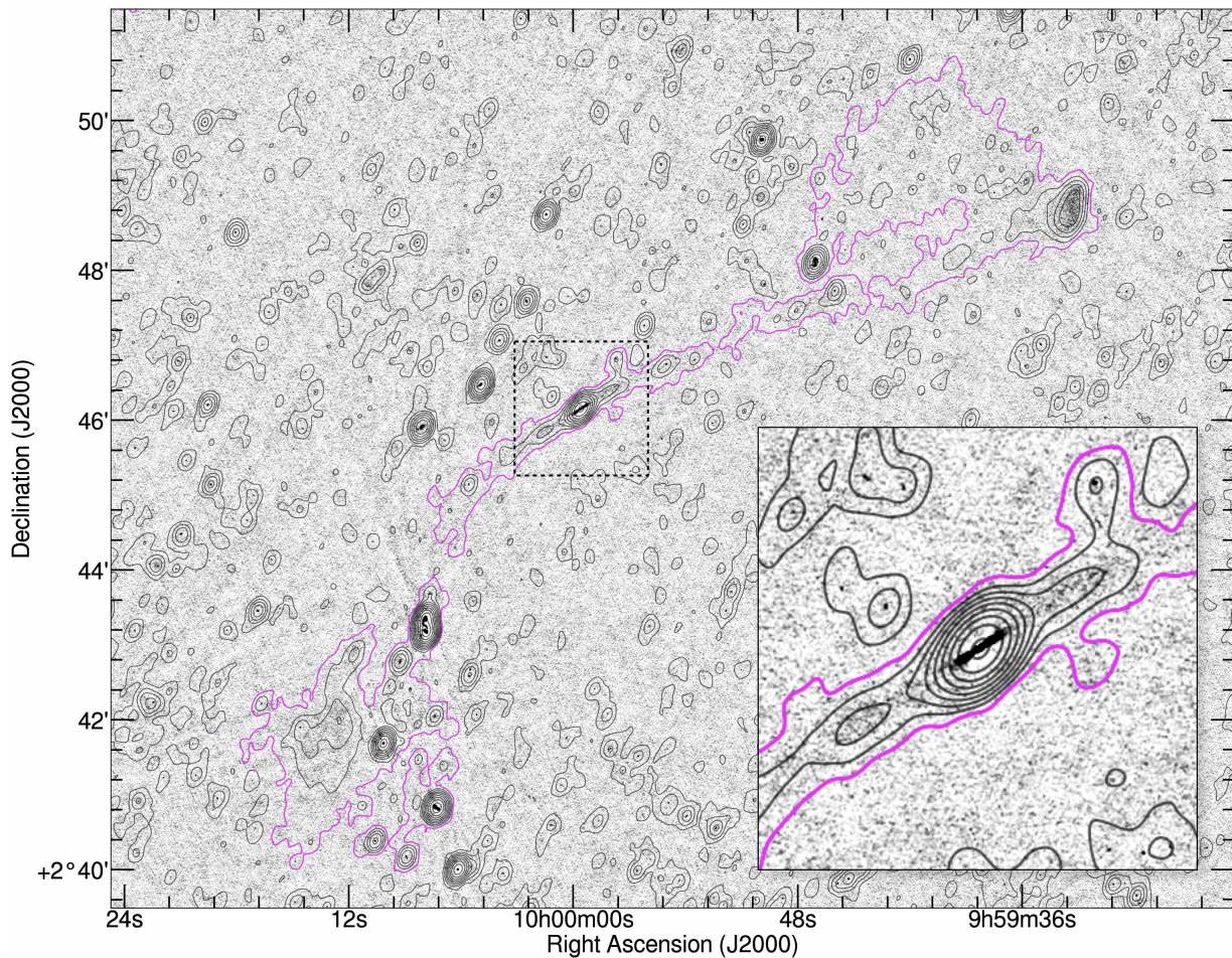
Figure 3. GRG1 as seen in the VLA-3GHz data (background map) and in the MIGHTEE data (black contours). Contour levels are as in Figure 2 and the lowest contour level is again shown in magenta. The hot-spot in the northern lobe is seen faintly at 3 GHz. The inset shows an enlargement of the core region, where a double-lobed/jetted structure can be seen in the VLA-3GHz image.
