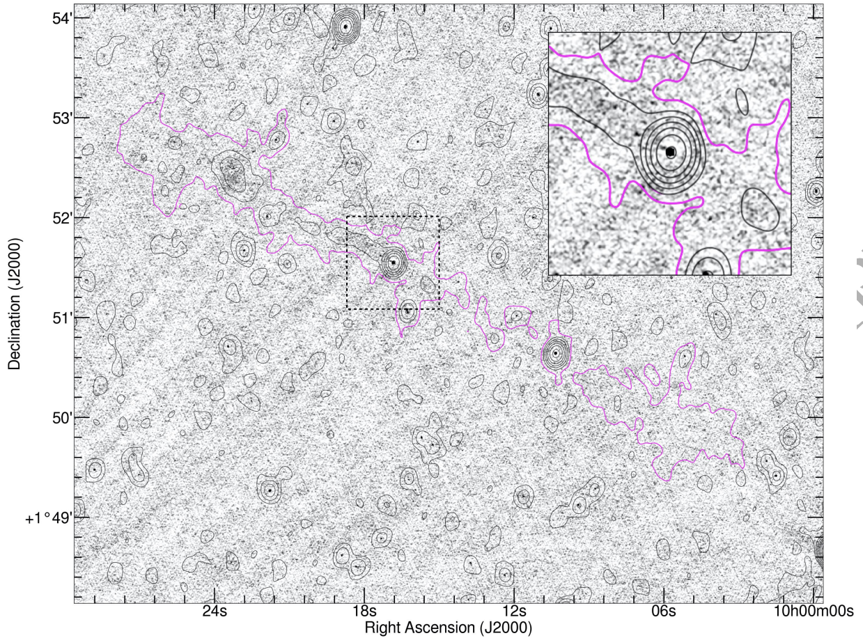
Figure 7. GRG2 as seen in the VLA-3 GHz data (background map) and in the MIGHTEE data (black contours). Contour levels as in Figure 2. At 3 GHz a compact core is seen and diffuse emission in the northern hot-spot is faintly visible.
