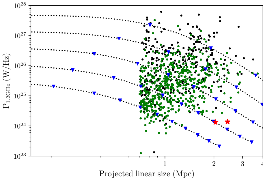
Figure 8. The position in the 1.2 GHz power-size (P-D) diagram of almost all known GRGs. Objects in the compilation catalogue of Dabhade et al. (2020b) are shown as green ( z < 0.5 ) and black ( z \geq 0.5 ) points. GRG1 and GRG2 are shown as red stars and are located in a previously unoccupied part of this diagram. For comparison, dotted lines show evolutionary tracks as determined by Hardcastle et al. (2019) for radio galaxies with jet powers of (bottom to top) 10^{37} , 10^{37.5} , 10^{38} , 10^{38.5} and 10^{39} W. The tracks show a lifetime of up to 1 Gyr with blue triangles marking each hundred Myr. GRG1 and GRG2 are consistent with the evolution of a \sim 10^{37.5} W jet after \sim 700 Myr.
