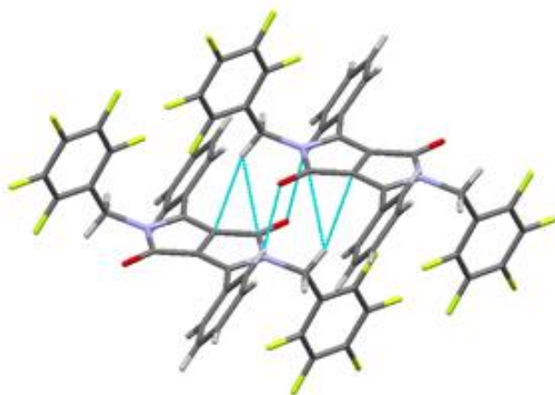
Figure 6. Capped stick representation of \pi - \pi stacking dimer pair V of HHFBDDPP , with illustrated close interatomic contacts.
