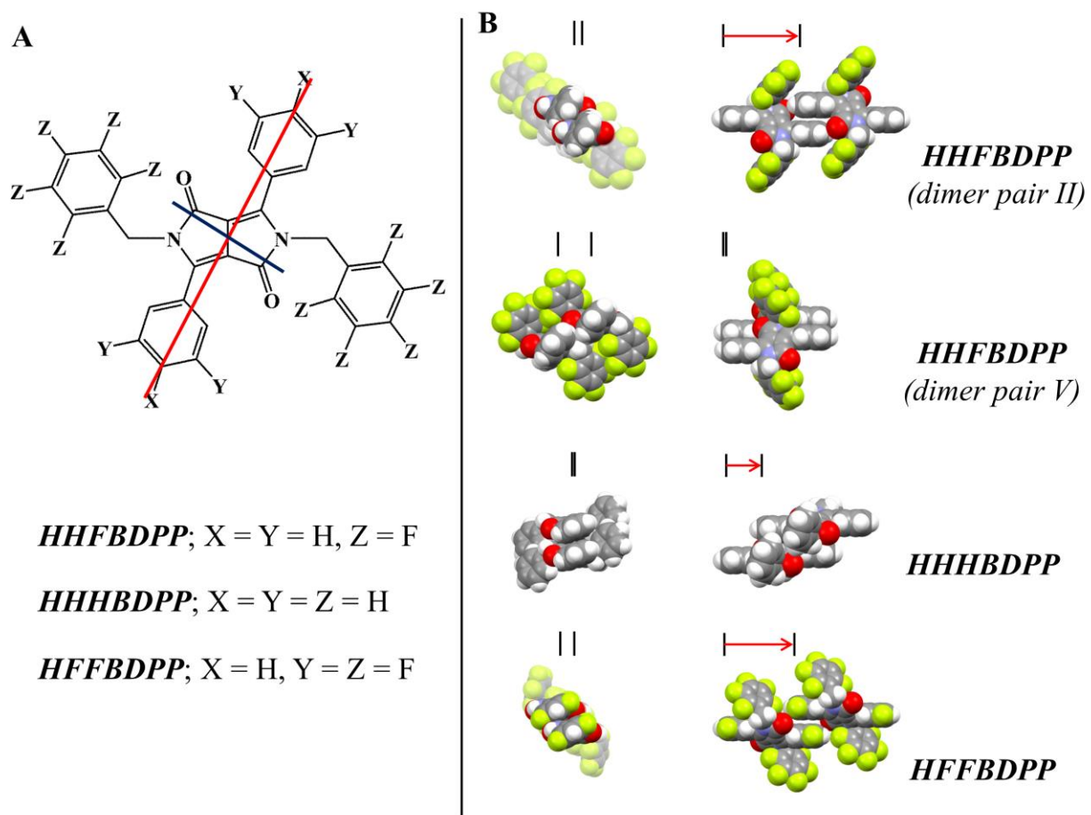
Figure 1. A Illustration of long and short molecular axes in DPP-based architectures. B Long and short molecular axis view of \pi - \pi dimer pair II and V of HHFBDPP and analogous systems, HHHBDPP and HFFBDPP for comparison. Phenyl-DPP cores in short molecular axis views of HHFBDPP and HFFBDPP are highlighted for ease of visualisation.
