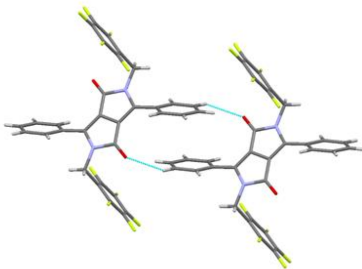
Figure 4. Capped stick representation of \pi - \pi stacking dimer pair II of HFFBDPP , with illustrated close interatomic contacts.
