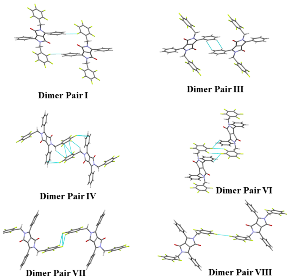
Figure 7. Capped stick representations of nearest neighbour dimer pairs I, III, IV, VI, VII and VIII of HHFBDDPP , with illustrated close interatomic contacts.
