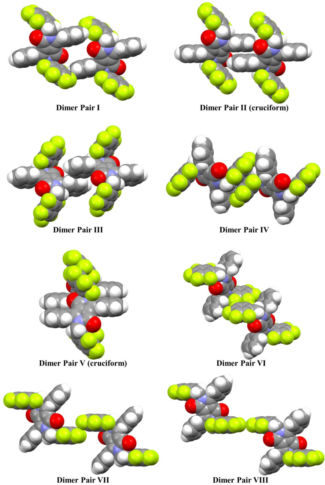
Figure 3. Space filled representation of all the nearest neighbour dimer pairs of HHFBDPP .
