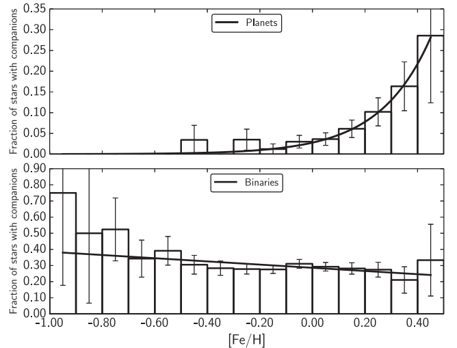
Figure 10. The metallicity distribution of exoplanet (upper panel) and binary (lower panel) companions. The best-fitting model distributions are also shown in the plots, where a power law is used for the exoplanet sample, and a linear function is used to model the binary distribution.
