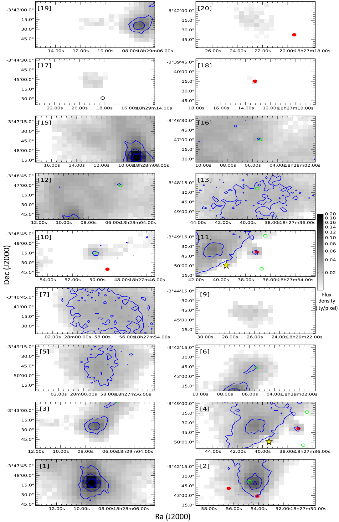
Figure 10. Comparison of flux emission from FELLWALKER objects at 450 \mu\text{m} (contours), 850 \mu\text{m} (greyscale) and the SGBS YSOs (markers). Numbers in square brackets correspond to the objects in Table 3. Maps show contours of 450 \mu\text{m} submillimetre flux at 5, 10, 20 and 30 \sigma ( \sigma = 0.016 Jy/pixel). Spitzer YSOs are indicated by hollow black circles (Class III), solid red circles (Class II) and green hollow circles (Class 0/I). The star indicates the location of the star MWC 297.
