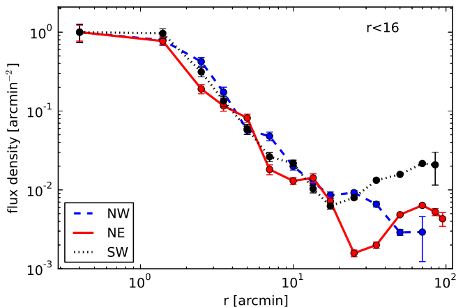
Fig. 12. Stellar density profiles for the north-west, north-east and south-west quadrants (respectively NW, NE and SW) of the VPHAS+ photometry, using stars with r < 16 . The profiles in the three quadrants were normalised to the flux in the innermost bin. The background level was not subtracted.
