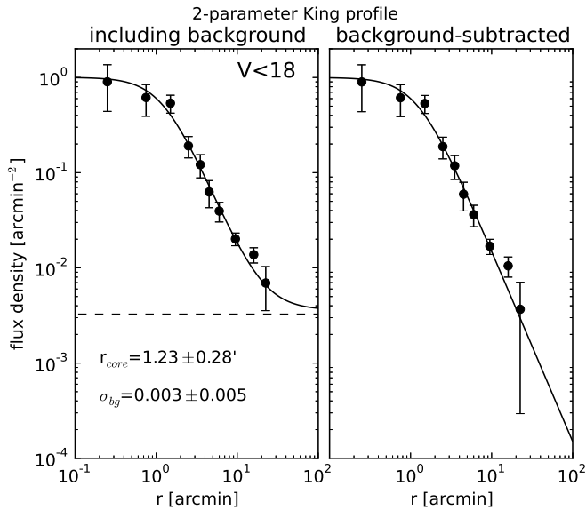
Fig. 11. Observed luminosity profile (black dots) for stars with V < 18 , fitted with a two-parameters King profile (continuous line), including background (left) and after subtracting the background (right). The flux density was normalised to the central luminosity so that \sigma_0 = 1 .
