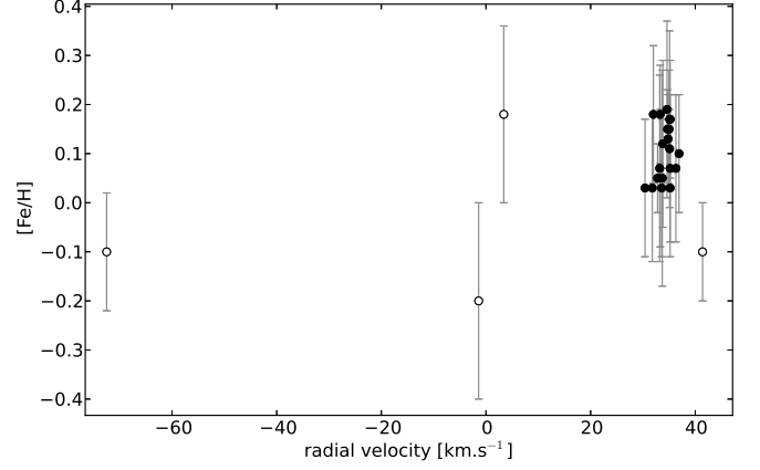
Fig. 7. Identification of the red clump cluster members from radial velocities and iron abundance. The error bars for the radial velocities are smaller than the symbols. The 21 filled circles correspond to the members, while the 4 open circles are the stars we consider non-members.
