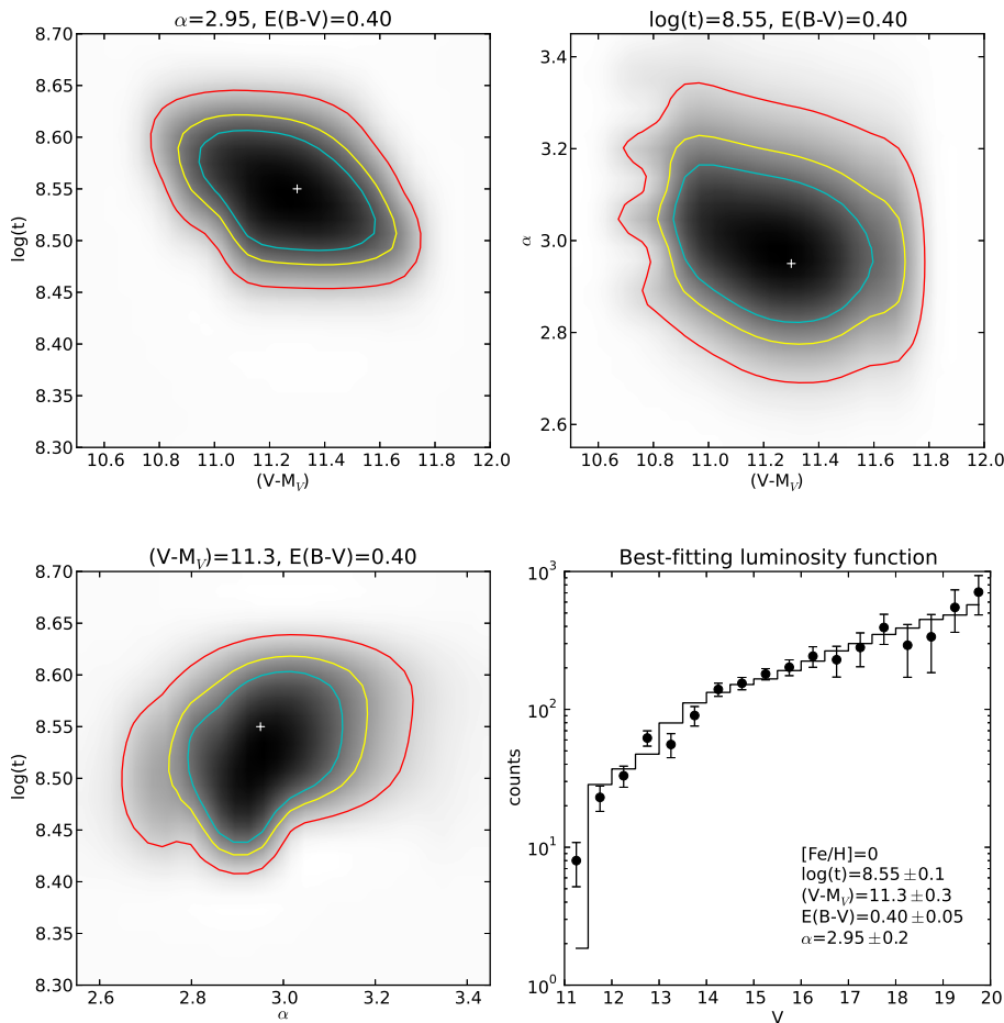
Fig. 18. Probability contours for the fit of the luminosity function. The cyan, yellow, and red lines show the 50%, 68% and 90% confidence regions, respectively. The white cross indicates the best-fitting solution. The bottom-right panel shows the observed LF (cleaned from the background) and the best-fitting theoretical one. The bins with V > 18 are shown but were not used in the fitting procedure.
