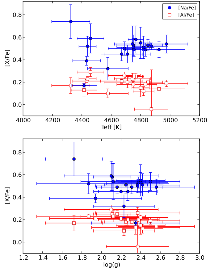
Fig. 20. Solar-scaled abundances of [\text{Na}/\text{Fe}] (blue filled dots) and [\text{Al}/\text{Fe}] (red open squares) for the 21 UVES member stars, as a function of T_{\text{eff}} and \log g .
