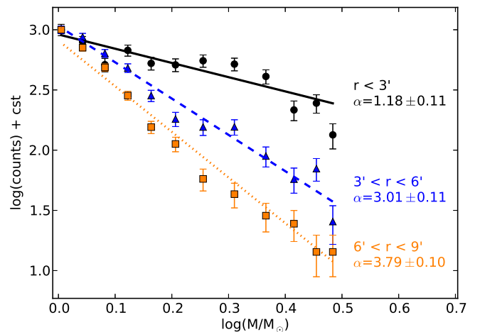
Fig. 19. Mass functions obtained in three different regions of the cluster, showing the flattening of the IMF in the center. The y-axis was shifted so that the observed number of stars in the lowest mass bin is the same for all three.
