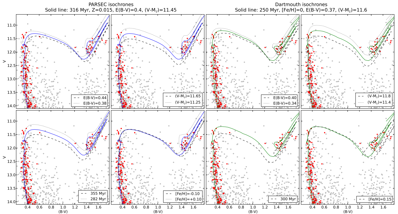
Fig. 15. The grey points are all the stars in our photometry, and the radial velocity members are marked in red. Left-hand side panels: The best-fitting PARSEC isochrone (solid blue line) corresponds to an age of 316 Myr, a solar metallicity, a reddening E(B - V) = 0.40 and a distance modulus (V - M_V) = 11.45 . The four panels show the change in the isochrone when modifying the extinction, distance modulus, age and metallicity with respect to the best-fitting isochrone. Right-hand side panels: same procedure with Dartmouth isochrones. The best-fitting isochrone is the solid green line. In all cases, the data are uncorrected for extinction (the isochrones are shifted along the extinction vector).
