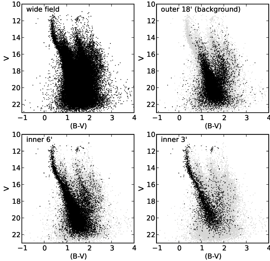
Fig. 3. Top-left: BV CMD of all 123 037 in our sample. Top-right: CMD of the outer 18', which we consider as our background field. Bottom-left and bottom-right: CMD of the inner 6' and 3'. In the latter three panels, the grey points correspond to the wide-field CMD.
