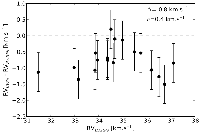
Fig. 6. Comparison between the radial velocity measurements from HARPS spectra and UVES spectra for 19 red giants.
