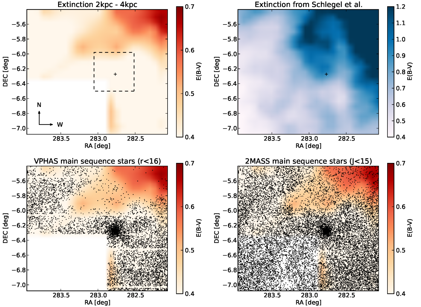
Fig. 9. Top-left: extinction map obtained from VPHAS+ photometry in the distance range 2-4 kpc. The cross indicates the center of the cluster. The dashed line shows the footprint of our BVI photometry. Bottom-left: same extinction map. The black points are cluster stars selected from the (r - i, r) VPHAS+ CMD, with r < 16 . The CCD gaps are visible as horizontal lines. Top-right: extinction map from Schlegel (1998) for this field. Bottom-right: same as bottom-left, but with 2MASS main-sequence stars ( J < 15 ).
