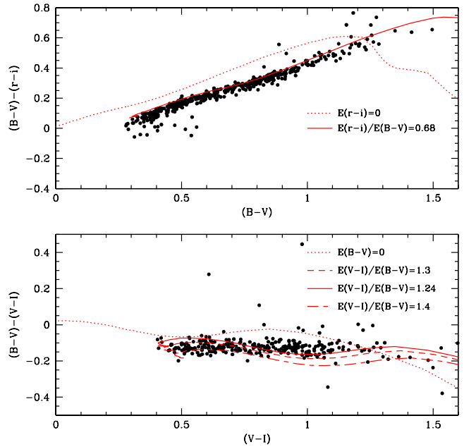
Fig. 8. Color-color diagrams on NGC 6705 GIRAFFE members main-sequence stars, compared with the relation expected from PARSEC isochrones for various extinction laws.
