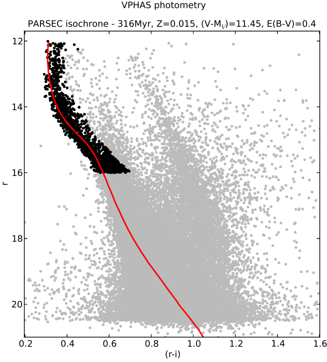
Fig. 4. VPHAS+ ri CMD of the central 12' of the cluster. The spatial distribution of the selected stars (black points) is shown in Fig. 9. The solid line corresponds to the PARSEC isochrone of best parameters, shifted for distance modulus and extinction (see Sect. 7 for detail). Stars brighter than r = 12 suffer from saturation and are not shown here.
