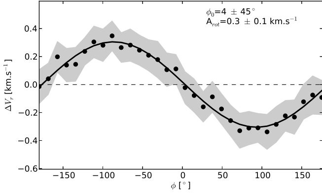
Fig. 14. Rotation curve obtained from the cluster members. The shaded region show the uncertainty estimated via bootstrapping. The best fitting sine corresponds to a position angle of the rotation axis \phi_0 = 4^\circ and an amplitude A_{rot} = 0.3 \text{ km s}^{-1} .
