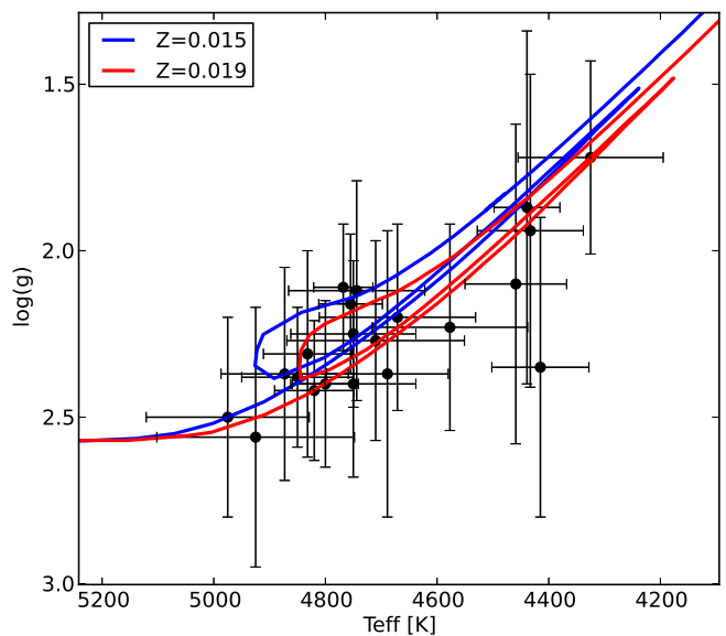
Fig. 17. Position of the 21 UVES members in the theoretical plane. The position of the red clump is well reproduced with a PARSEC isochrone of age \log t = 8.5 and Z = 0.015 ( [\text{Fe}/\text{H}] = 0 ) or Z = 0.019 ( [\text{Fe}/\text{H}] = 0.1 ).
