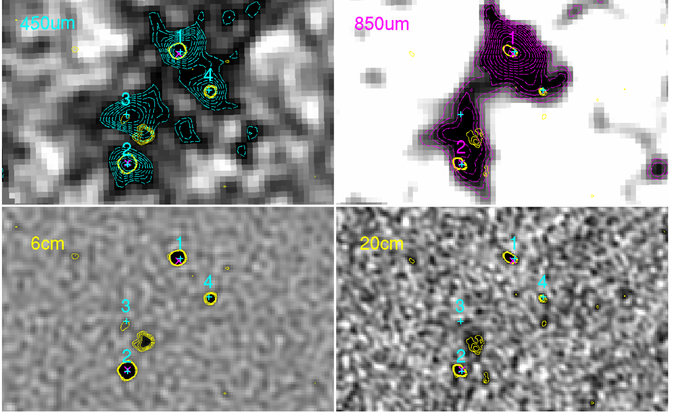
Figure 1. Finding charts of a 2.1' \times 1.3' region around the submm structure associated with RX J0941 (N is up and E to the left). The region around 850.3 (to the NW of RX J0941) is shown separately in Fig. 5. Top left: 450 \mu\text{m} SNR image with 2 to 6 \sigma contours (in steps of 0.5 \sigma , dashed cyan) and 6cm 2 to 5 \sigma contours (in steps of 1 \sigma , yellow), the numbers and crosses in cyan correspond to the 450 \mu\text{m} sources in Table 1. Top right: 850 \mu\text{m} SNR image with 2 to 8 \sigma contours (in steps of 0.5 \sigma , dashed magenta) and 20cm 2 to 5 \sigma contours (in steps of 1 \sigma , yellow), the numbers and “x” in magenta correspond to the 850 \mu\text{m} sources in Table 1 (the cyan crosses to the 450 \mu\text{m} sources in that Table). Bottom left: 6cm image and contours (as above) with source numbers and crosses as above (note that sources 1 and 2 are common to 450 \mu\text{m} and 850 \mu\text{m} ). Bottom right: 20cm image and contours (as above) with source numbers and markers as above. In greyscale, magenta appears slightly darker than cyan and the steeper yellow contours appear white.
