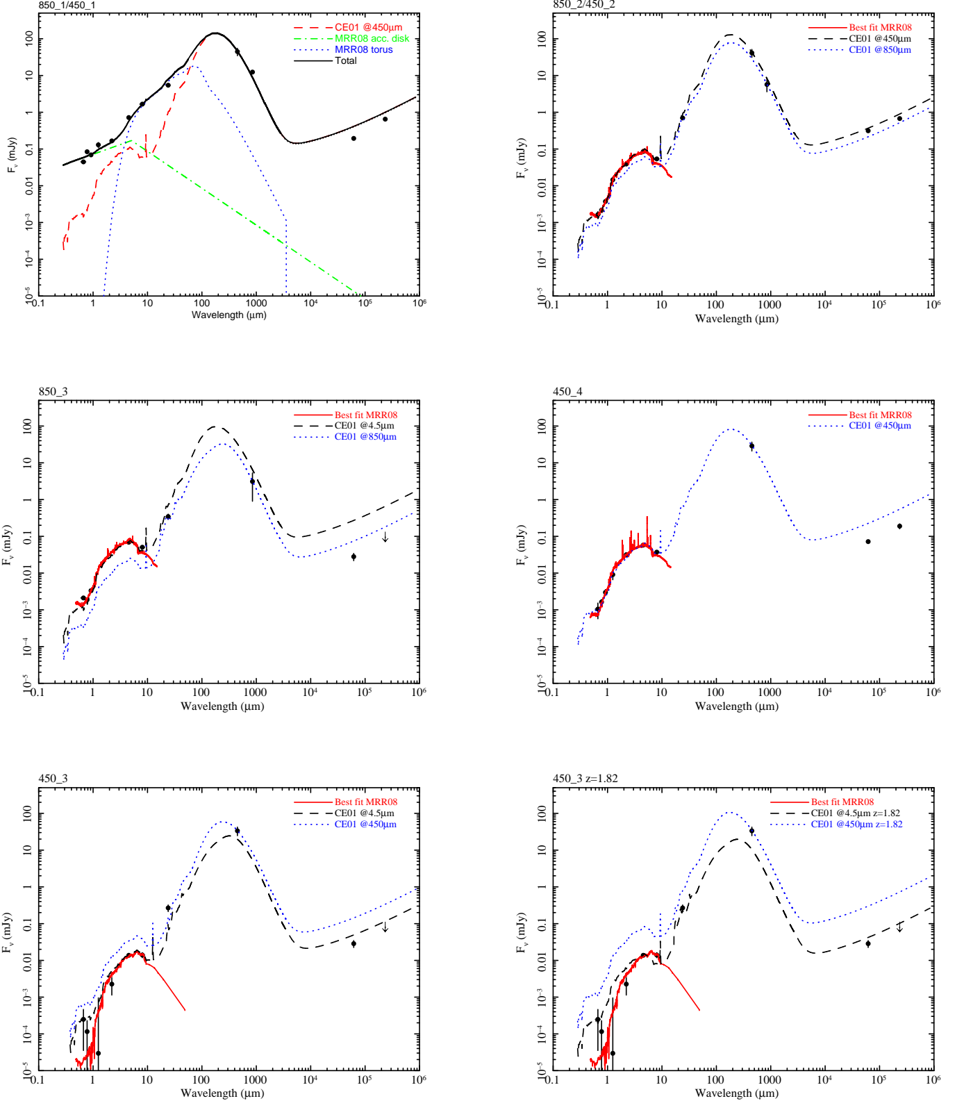
Figure 2. Spectral Energy Distribution in F_\nu in the observer’s frame for 850.1/450.1 (RX J0941, top left), 850.2/450.2 (top right), 850.3 (middle left), 450.4 (middle right), and 450.3 (with templates at the best photometric redshift -bottom left- and fixed at z = 1.82 -bottom right-). Observed points ( RiZJK , 4.5, 8, 24, 450 and 850 \mu\text{m} , and 6 and 20 cm) are shown as black dots and upper limits as down-pointing arrows. The meaning of each line is summarized in each panel and explained fully in Section 4.2.
