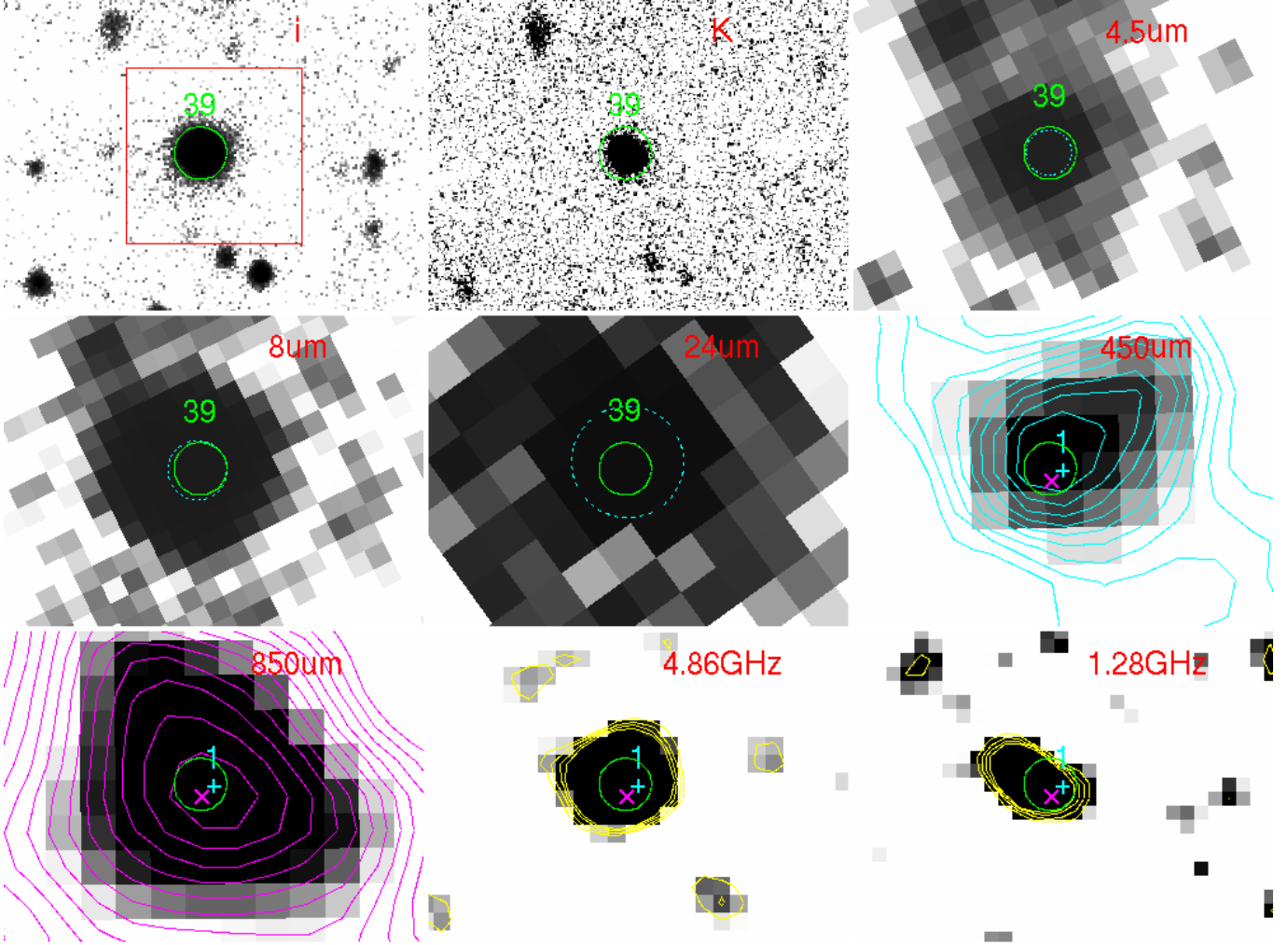
Figure 3. Finding charts for 850.1/450.1. From top-left to bottom-right: i (the size of the red box is 10'' \times 10'' ), K , 4.5 \mu\text{m} (dashed cyan circle is the positions of the 4.5 \mu\text{m} sources with radius equal to the flux extraction radius), 8 \mu\text{m} (dashed cyan circles mark 8 \mu\text{m} sources and extraction radii), 24 \mu\text{m} (dashed cyan circles mark 24 \mu\text{m} sources and extraction radii), 450 \mu\text{m} (with cyan contours starting at 2\sigma and increasing in steps of 0.5), 850 \mu\text{m} (with magenta contours, starting at 2\sigma and increasing in steps of 0.5), 4.86 \text{ GHz} (with yellow contours starting at 2\sigma and in intervals of 1), 1.28 \text{ GHz} (with yellow contours, same as previous). All finding charts have the same FOV and the solid circles indicate the optical/NIR source position and extraction radius (green corresponds to 1.5'' , red to smaller radii), only the sources mentioned in the text have been labelled. The labels have been omitted in the SCUBA and radio images for clarity, but we have labelled and marked instead with cyan “+” our positions for the 450 \mu\text{m} and with magenta “x” the positions of the 850 \mu\text{m} sources.
