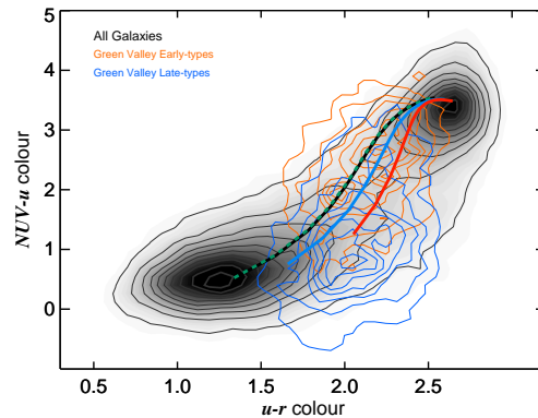
Figure A2. The NUV_{ur} colour diagram, similar to Figure 7, with the same Model tracks shown as on Figure A1. All models that are on the main sequence at the time of quenching (black, green, light blue) yield a short quenching. The red model, which is incompatible with the Main Sequence due to having a low SSFR at the quenching time, is somewhat offset, but still yields a short quenching time scale on the NUV_{ur} diagram. Together with Figure A1, this Figure illustrates the robustness of the NUV_{ur} diagram as a quenching time and that all reasonable star formation histories that end up on the main sequence are blue, and reasonable starting points for our quenching model.
