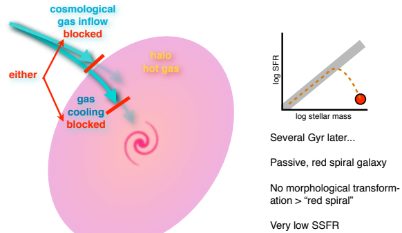
Figure 13. Diagram outlining the scenario presented here for star-formation quenching in late-type galaxies. Once the external supply of gas to the galaxy's reservoir is cut off, the galaxy will leave the main sequence, and the SFR will decay exponentially, with a long quenching time scale \tau_{\text{quench}} . While no longer on the main sequence, the galaxy nevertheless continues to convert gas to stars and thus to increase its stellar mass. Absent a major merger, this evolutionary pathway eventually produces a passive, red, late-type galaxy. We see radiation from black hole growth during stage (3), long after the quenching event actually took place.
