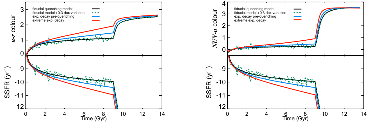
Figure A1. Evolution of u - r colour ( left ) and NUV - r colour ( right ) as a function of time for a set of four models. Below the colour evolution of each model, we show the specific star formation rate as a function of time. Model 1 (black line): fiducial model of constant SFR, followed by exponential decay, in this case with \tau_{\text{quench}} = 100 Myr. Model 2 (green dashed line): same as Model 1, but with random perturbations prior to quenching. Model 3 (light blue line): rather than a constant SFR, the pre-quenching star formation history is a gently exponentially declining SFR. This SFR builds up a more significant old stellar population by the time of quenching. The model is tuned to have an SSFR at the quenching time t_{\text{quench}} = 9 Gyr that is at the lower edge of the Main Sequence. Model 4 (red line): same as Model 3, but with a more strongly exponentially declining SFR prior to quenching. This Model has an SSFR \sim 1 dex below the Main Sequence at t_{\text{quench}} . Due to its low SSFR at t_{\text{quench}} , Model 4 is incompatible with the Main Sequence. The other models, do not show significant offsets from the fiducial quenching model as they all have the following salient features: at t_{\text{quench}} , they have blue cloud u - r and NUV - u colours, and after the quenching event, they become redder at essentially the same rate. Thus, all SFHs which place a galaxy on the main sequence at the point of quenching yield similar quenching timescale.
