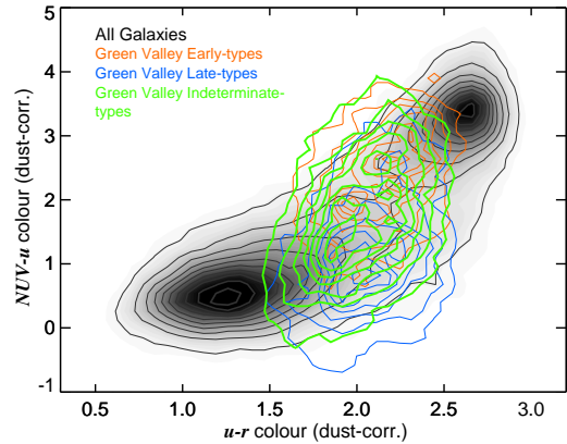
Figure 9. NUVur diagram, similar to the upper left panel in Figure 7 but showing the indeterminate-type galaxies as green contours, with early types as orange contours and late types as blue contours. The bulk of the green valley indeterminate-types overlap the green valley late-type locus, with somewhat redder colours, with a minority scattering to the early-type locus. This supports a picture where the indeterminate-types quenching slowly, similar to the late types, with the minority misclassified early types possibly quenching more rapidly.
