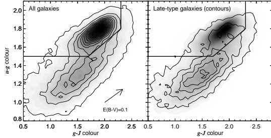
Figure 4. The ugJ colour-colour diagram for our sample, analogous to the UVJ diagram of Williams et al. (2009). The arrow indicates the shift due to dust for an E(B-V)=0.1 using a Calzetti et al. (2000) extinction law. In the left -hand panel, we show all galaxies and an adapted box separating passive red galaxies from dusty star-forming galaxies. The right -hand panel shows the (same) shading of the entire galaxy sample, with contours for late-type galaxies only; this shows that some of the red spirals are actually dust-reddened spirals, while others are passively evolving.
