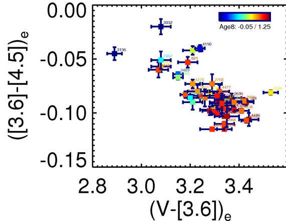
Figure 15. [3.6] - [4.5] colour vs. V - [3.6] (from Paper XIX, both in \text{mag arcsec}^{-2} ) within r_e .
