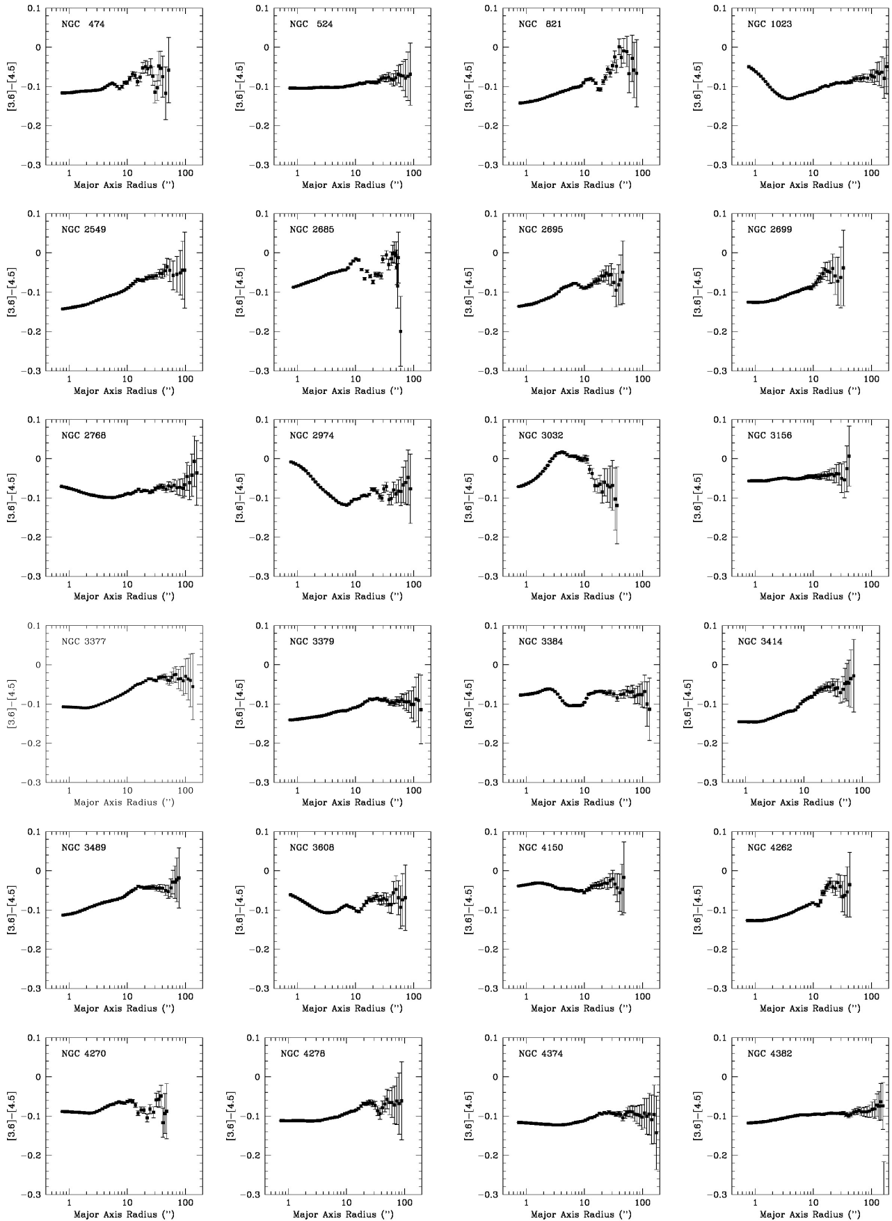
Figure 4. a) [3.6] - [4.5] colour profiles in \text{mag arcsec}^{-2} of the sample galaxies.
