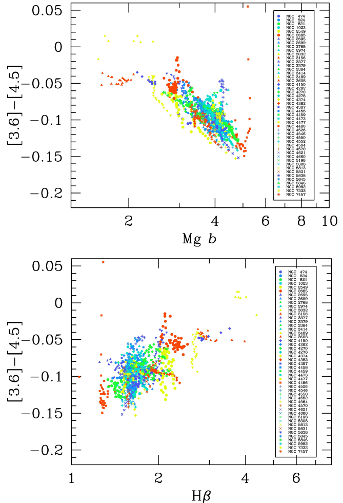
Figure 19. Local colour in mag arcsec ^{-2} plotted as a function of local line strength index Mg b (a) and H \beta (b) (both in \text{\AA} ). Line indices from Paper VI.
