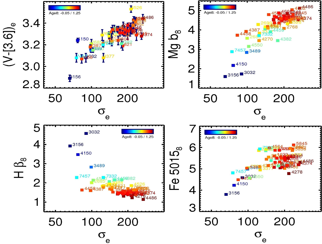
Figure 11. Various colour/line strength vs. velocity dispersion plots. In Fig. 11a (top-left) the V-[3.6] colour in \text{mag arcsec}^{-2} within r_e is plotted (from Paper XIX). All line strengths (in Fig. 11b,c and d) are equivalent widths in \text{\AA} and have been calculated within apertures of r_e/8 . The points are coloured according to age within r_e/8 .
