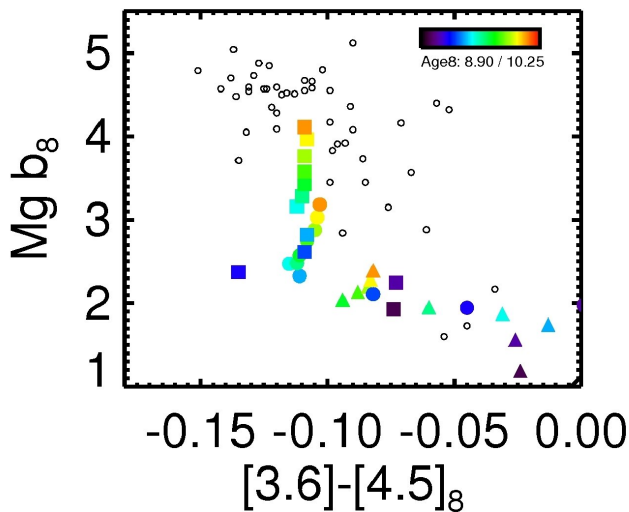
Figure 14. [3.6] - [4.5] colour - Mg\ b diagrams. The black open circles indicate the galaxy data presented in Section 4 using apertures of radius r_e (top) and r_e/8 (bottom). Coloured points indicate SSP models, composed of [3.6] - [4.5] colours from Marigo et al. (2008) and Mg\ b line indices from Bruzual & Charlot (2003). Models are given for solar metallicity Z=0.008 (filled triangles), Z=0.02 (filled circles) and Z=0.03 (filled squares). The models are coloured according to their age.
