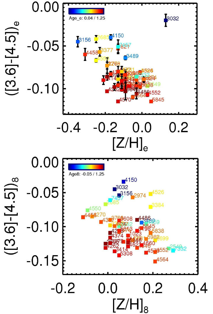
Figure 8. Relation between SSP-metallicity [Z/H] (Paper XVII) and the [3.6] - [4.5] colour inside r_e (Fig.8a) and r_e/8 (Fig.8b). Colouring of the points as in Fig.6.
