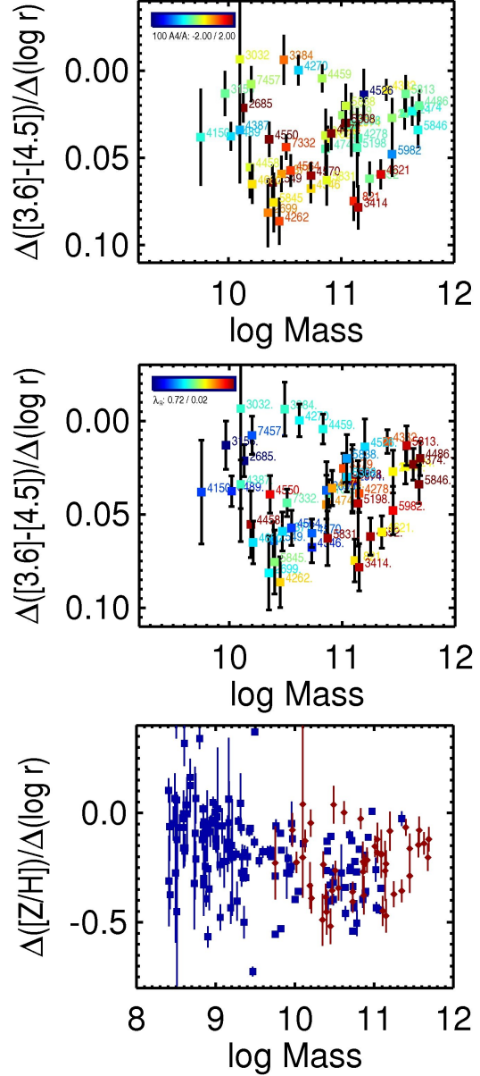
Figure 17. (a) and (b): [3.6] - [4.5] colour gradient as a function of galaxy mass. In Fig. 17a) the points have been coloured using the boxy/diskiness inside r_e (from Paper IX). In Fig. 17b) they have been coloured using their \lambda_R (Paper IX). (c) Colour gradient, converted to metallicity gradient, as a function of mass. Plotted here are the sample of this paper (red) and the Coma sample of den Brok et al. (2011, blue). In Fig.17(a) and (b) dynamical masses are plotted. In Fig.17(c) the stellar masses of den Brok et al. (2011) are used, all in solar units.
