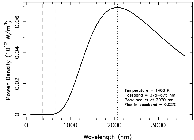
FIG. 9.— The predicted blackbody flux of HD 20782b, assuming a calculated temperature of \sim 1400 K. The passband boundaries of MOST are indicated by the vertical dashed lines. The blackbody calculation assumes zero Bond albedo and zero heat redistribution (hot dayside model) and thus represents a maximum flux scenario. Of the integrated flux, 0.02% falls within the MOST passband.
