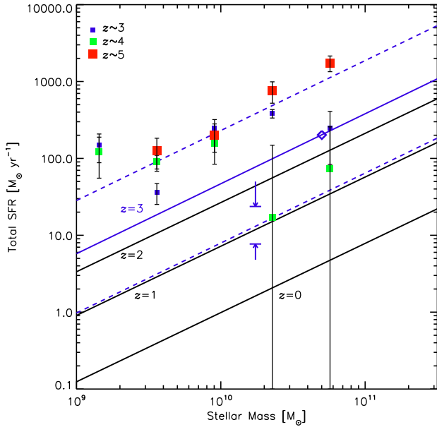
Figure 8. The “main sequence” of star-forming galaxies predicts increasing star formation activity with stellar mass, and the relation is known to evolve with redshift. The observed correlations are plotted at z = 0 (Noeske et al. 2007), z = 1 (Elbaz et al. 2007), z = 2 (Daddi et al. 2008), and z = 3 (from Magdis et al. 2010a, based on IRAC-detected LBGs). The blue dashed lines simply represent the extent of the 1\text{-}\sigma spread in the Magdis et al. 2010a data, to guide the eye to the likely range of values at z \sim 3 . This plot has been adapted from Davies et al. (2013) and their limits for typical z \sim 3 LBGs are shown as blue arrows, as well as their submm detection of IRAC-22.5 (high mass) sub-sample. All of the data points and correlations shown take into account the total (obscured-unobscured) SFRs. Similar to Fig. 6 (which only shows the trend for the obscured SFRs with stellar mass), our new data hint that the SFRs of LBGs at z \sim 3, 4 , and 5 scale with mass, with the most massive LBGs tending to have the highest overall SFRs.
