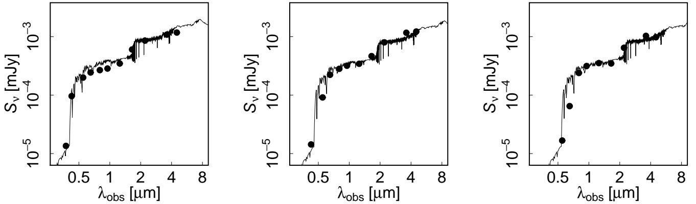
Figure 3. Best-fitting Bruzual (2007) model for z = 3 LBGs selected at 24\mu\text{m} from Magdis et al. (2010b), normalised to the observed K -band flux of each LBG sample at z = 3, 4, and 5 . This simple SED scaling provides an overall excellent description of the observed average photometry, with only a slight discrepancy in the UV emission at z = 4 and z = 5 , most likely due to increasing \text{Ly}\alpha forest absorption at z > 3 (see text).
