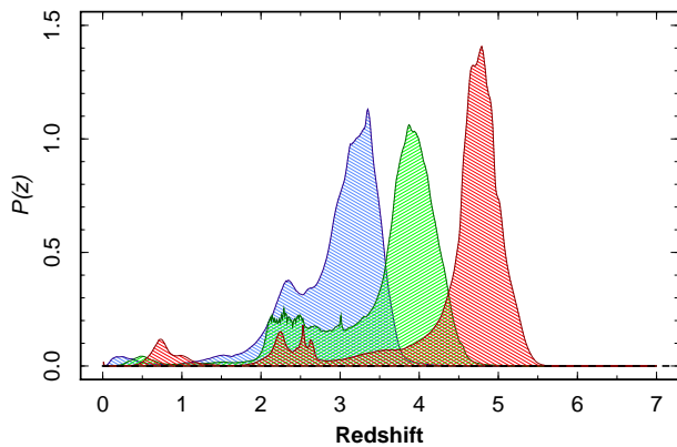
Figure 1. Stacked photometric redshift distributions from EAZY (see text) of the sources selected in our three LBG samples (all normalised to a common integral), clearly showing the three distinct peaks in redshift space, centred at z \sim 3, 4, and 5 .
