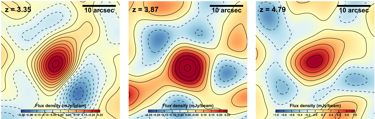
Figure 2. Thumbnail images of the stacked 850\ \mu\text{m} flux in the SCUBA-2 map, centred on the LBG positions in the z \sim 3, 4, and 5 sub-samples (the mean redshift of each LBG sub-sample is indicated on each image). The colour scale indicates the average flux density and the solid contours represent significance levels of 0, 1, 2, 3- \sigma ,..., and the dashed lines are the corresponding to negative deviations.
