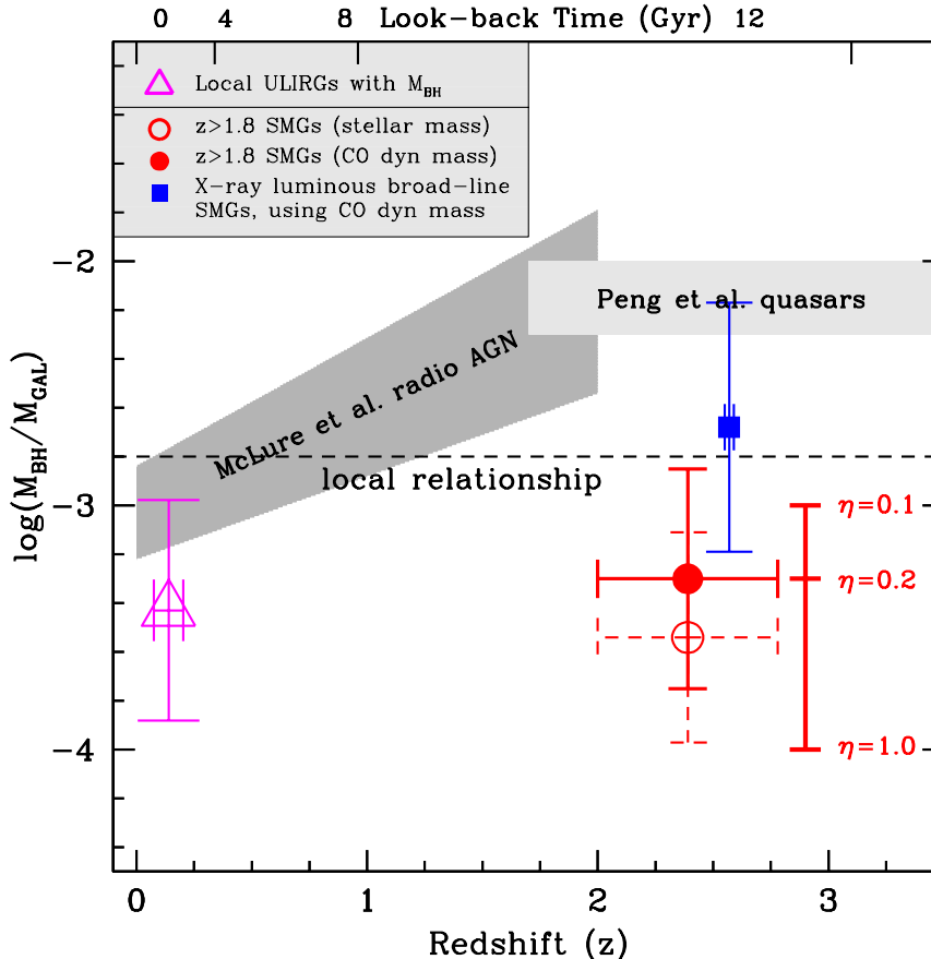
FIG. 7.— Black-hole–host-galaxy mass ratio versus redshift for the z > 1.8 X-ray obscured SMGs, X-ray luminous broad-line SMGs, and the obscured ULIRGs with broad Pa \alpha emission. The z > 1.8 X-ray obscured SMGs are plotted using the stellar mass and the CO dynamical mass constraints. The dashed line indicates the local black hole–spheroid mass relationship from Häring & Rix (2004), the dark-shaded region shows the radio galaxy constraints from McLure et al. (2006), and the light-shaded region indicates the constraints for z \approx 2 quasars from Peng et al. (2006). The error bars correspond to 1\sigma uncertainties. The X-ray obscured SMGs lie marginally below the local relationship (factor \approx 3 – 5 ), as also found for the nearby obscured ULIRGs, and they lie a factor \approx 10 below that found for z \approx 2 radio galaxies and quasar population. This suggests that SMGs are identified at an earlier stage in the evolution of quasars and massive galaxies. The X-ray luminous broad-line SMGs are statistically consistent with the local relationship, assuming the CO dynamical mass constraints from the SMGs and the average Eddington ratio of \eta = 0.6 . We discuss the overall constraints in §5.
