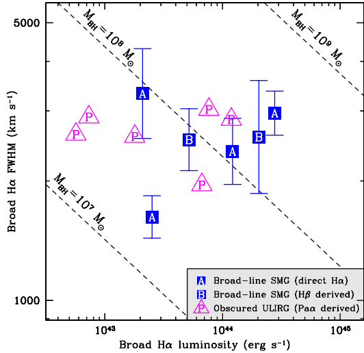
FIG. 1.— H\alpha properties of the broad-line SMGs and obscured ULIRGs. Sources indicated with letters have had their H\alpha properties determined from their extinction-corrected H\alpha emission (“A”), derived from their H\beta properties for an intrinsic H\alpha/H\beta ratio of 3.1 (“B”; see §3.1), or derived from their Pa\alpha properties for an intrinsic H\alpha/Pa\alpha ratio of 8.6 (“P”; see §4.1). The dashed lines show the relationship between the black-hole mass ( M_{BH} ) and the broad H\alpha emission-line properties on the basis of the virial black-hole mass estimator of Greene & Ho (2005). Taken at face value the data suggest that broad-line SMGs have a range of black-hole masses with a mean of \log(M_{BH}/M_{\odot}) \approx 8.0 ; the obscured ULIRGs have a mean black-hole mass of \log(M_{BH}/M_{\odot}) \approx 7.8 . However, if it is assumed that the BLR gas in the broad-line SMGs is distributed in a disk that is seen close to pole on (rather than the BLR gas being isotropically distributed and in random motion) then the average black-hole mass will be \approx 2.7 times larger, on the basis of the model described in the text (see §3.2).
