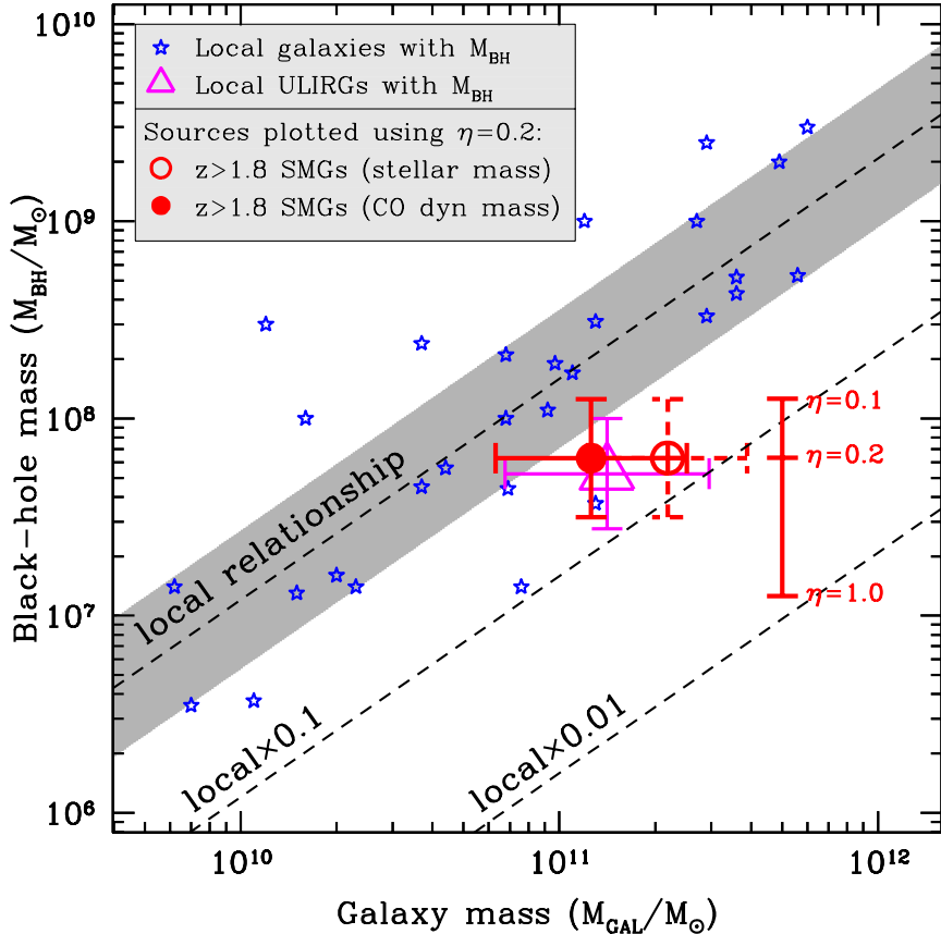
FIG. 4.— Black-hole versus galaxy mass. We plot the estimated average properties of the X-ray obscured SMGs for different host-galaxy mass measurements (CO dynamics; Greve et al. 2005; stellar masses; Borys et al. 2005), assuming \eta = 0.2 . We also plot the average properties of the obscured ULIRGs with broad Pa \alpha emission (see §4.1) and show the properties of well-studied nearby galaxies (taken from Häring & Rix 2004). The error bars correspond to 1\sigma uncertainties on the average properties. The shaded region indicates the black hole–spheroid mass relationship from Häring & Rix (2004) and the dashed lines indicate different ratios of this relationship. The solid bar indicates the black-hole mass constraints for the X-ray obscured SMGs for different Eddington ratios. For \eta = 0.2 , the SMGs lie \approx 3 – 5 times below this relationship, depending upon whether the average CO dynamical mass or stellar mass constraints are used; these results are qualitatively consistent with those found for the nearby obscured ULIRGs.
