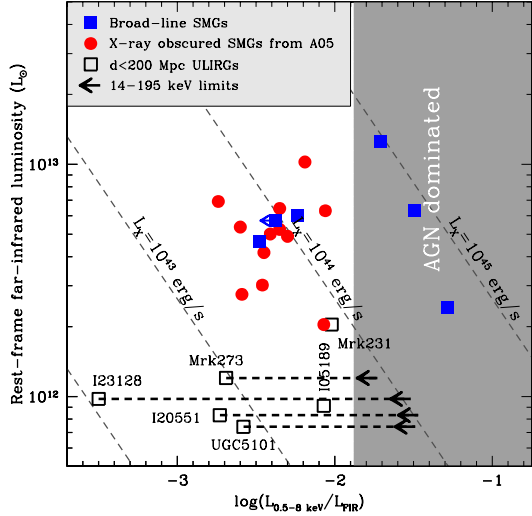
FIG. 3.— Rest-frame far-IR luminosity versus X-ray-to-far-IR luminosity ratio for the X-ray obscured SMGs, the broad-line SMGs, and the d < 200 Mpc ULIRGs; the X-ray luminosities are corrected for absorption, where necessary. The arrows indicate the 14–195 keV limits for the d < 200 Mpc ULIRGs from Swift -BAT (Markwardt et al. 2005); both Mrk 231 and I05189-2524 are detected at high X-ray energies (20–50 keV) using BeppoSAX -PDS (Dadina 2007). The far-IR luminosities for the X-ray obscured SMG and the broad-line SMGs are calculated from the radio luminosity assuming the radio-to-far-IR relationship (the former are taken from Alexander et al. 2005b), and the far-IR luminosities for the d < 200 Mpc ULIRGs are taken from Sanders et al. (2003). The diagonal dashed lines indicate different X-ray luminosities and the shaded region shows where AGN-dominated sources will lie on the basis of the Elvis et al. (1994) spectral energy distribution (taken from Fig. 8 of Alexander et al. 2005b). The three lower-luminosity broad-line SMGs lie in the same location of the L_X – L_{\text{FIR}} plane as the X-ray obscured SMGs, however, the other three broad-line SMGs have X-ray luminosities \approx 10 times higher than the broad-line SMGs and are not typical of the SMG population (these X-ray luminous broad-line SMGs are probably AGN dominated systems).
