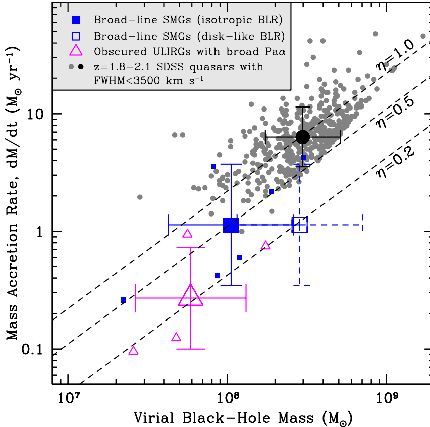
FIG. 2.— Mass accretion rate versus black-hole mass of the broad-line SMG sample, a sample of nearby ULIRGs hosting obscured AGNs but with detected broad Pa \alpha emission, and z = 1.8 – 2.1 SDSS quasars with comparatively narrow emission lines ( \text{FWHM} < 3500 \text{ km s}^{-1} ; data taken from McLure & Dunlop 2004). The error bars correspond to 1\sigma uncertainties on the average properties. The dashed lines indicate Eddington ratios ( \eta = L_{\text{bol}}/L_{\text{Edd}} ; i.e., the fraction of the Eddington limit) of \eta = 0.2 , \eta = 0.5 , and \eta = 1.0 . The average Eddington ratio of the broad-line SMGs is \eta \approx 0.5 , assuming that the BLR gas is isotropically distributed and in random motion, or \eta \approx 0.2 , assuming that the BLR gas is distributed in a disk that is observed close to pole on (see §3.2); this is compared to the average for the SDSS quasars with comparatively narrow emission lines ( \eta \approx 1.0 for BLR gas in random motion). The average Eddington ratio of the nearby ULIRGs hosting obscured AGNs, where inclination-angle effects will not be as important, is \eta \approx 0.2 (see §4.1).
