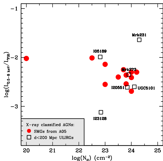
FIG. 6.— Unabsorbed 0.5–8.0 keV-to-far-IR luminosity ratio versus X-ray derived column densities for the z > 1.8 X-ray obscured SMGs from Alexander et al. (2005b) and the six d < 200 Mpc ULIRGs hosting obscured AGN activity (see §4.2). The far-IR luminosities for the X-ray obscured SMGs are from Alexander et al. (2005b) and are calculated using the radio-to-far-IR relationship, and the far-IR luminosities for the d < 200 Mpc ULIRGs are taken from Sanders et al. (2003). The column density and X-ray-to-far-IR luminosity ratio distributions of both populations are similar.
