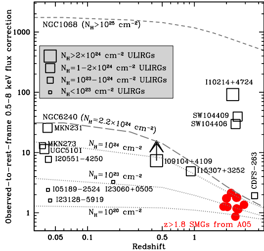
FIG. 5.— X-ray flux absorption corrections versus redshift for X-ray obscured AGNs in ULIRGs at low and high redshift (taken from Brandt et al. 1997; Franceschini et al. 2000, 2003; Severgnini et al. 2001; Imanishi et al. 2003; Ptak et al. 2003; Braito et al. 2004; Alexander et al. 2005c; Balestra et al. 2005; Mainieri et al. 2005; Polletta et al. 2006) and the z > 1.8 X-ray obscured SMGs studied in Alexander et al. (2005b). The corrections that would need to be made for two nearby Compton-thick AGN NGC 1068 (dashed curve; using Matt et al. 1997 model) and NGC 6240 (long dashed curve; using Vignati et al. 1999 model) are shown in addition to the models adopted by Alexander et al. (2005b) for lower amounts of obscuration (dotted curves); the assumed column densities are indicated. The X-ray derived column densities for the ULIRGs are indicated using different symbol sizes. The negative K -corrections for AGNs in the X-ray band mean that the absorption corrections are not large for high-redshift objects unless they are heavily Compton thick (i.e., N_{\text{H}} \gg 10^{24} \text{ cm}^{-2} ). The good agreement between the absorption corrections used in Alexander et al. (2005b) and those of obscured ULIRGs in the literature indicate that the intrinsic X-ray luminosities of the X-ray obscured SMGs are unlikely to be significantly underestimated.
