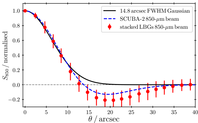
Figure 3. Light profile of the z \approx 3 850- \mu\text{m} stack (red points), compared with the SCUBA-2 850- \mu\text{m} beam (dashed blue line) of Geach et al. (2017) and a 14.8 arcsec FWHM Gaussian (black solid curve). The stacked profile is consistent with the beam and therefore any contribution from clustering of associated sources must be on scales below 15'' if present at all.
