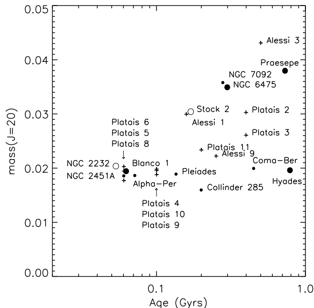
Figure 2. The J=20 mass limit for open clusters from Dias et al. (2002). Small filled circles have [M/H] = -0.1 – -0.1 , and larger circles have [M/H] = \pm 0.1 – \pm 0.2 (filled circles are metal rich and open metal poor). Clusters with unknown [M/H] are shown as plus signs. Where points are congested, cluster names for several plus signs have been grouped together, with an arrow indicating the location of the group.
