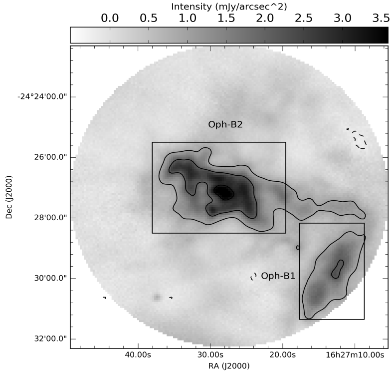
Figure 1. The 850\mu\text{m} dust emission map of Oph-B clump obtained using SCUBA-2 on the JCMT. The two sub-clumps, B1 and B2, are labeled with boxes. Contours are of 850\mu\text{m} emission (greyscale) and the contour levels are drawn with (0.6, 1.8, 2.9, 4.1) \text{mJy}/\text{arcsec}^2 .
