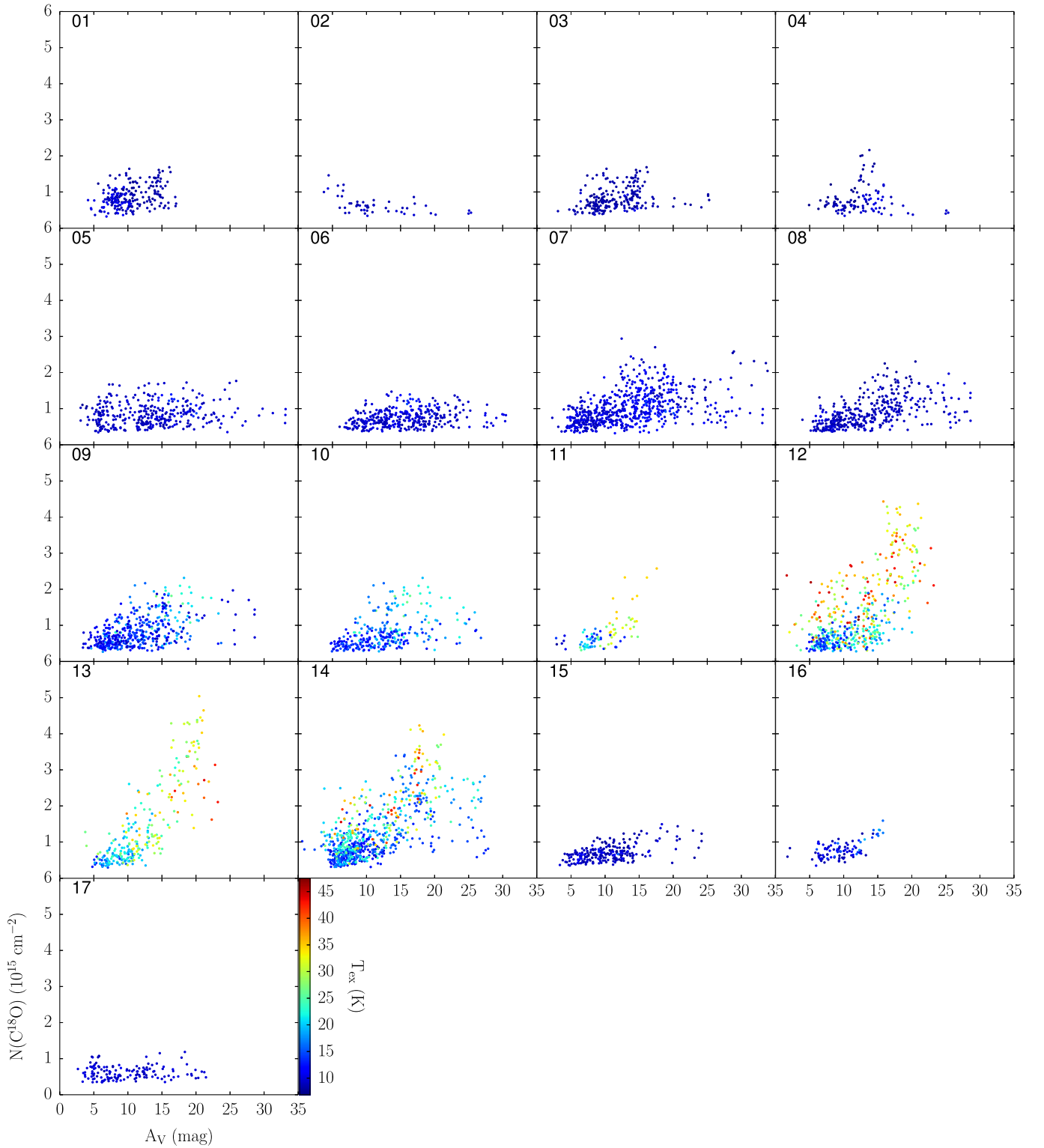
Figure 7. Pixel-by-pixel comparison between C^{18}O column density and A_V within each tile. A 2\sigma_{W,18} cut is applied to the integrated intensity in the N(C^{18}O) calculation. The magnitude of the error is the same as in Figure 5(b). The axes have the same horizontal and vertical scales for all tiles; otherwise, the same as Figure 6.
