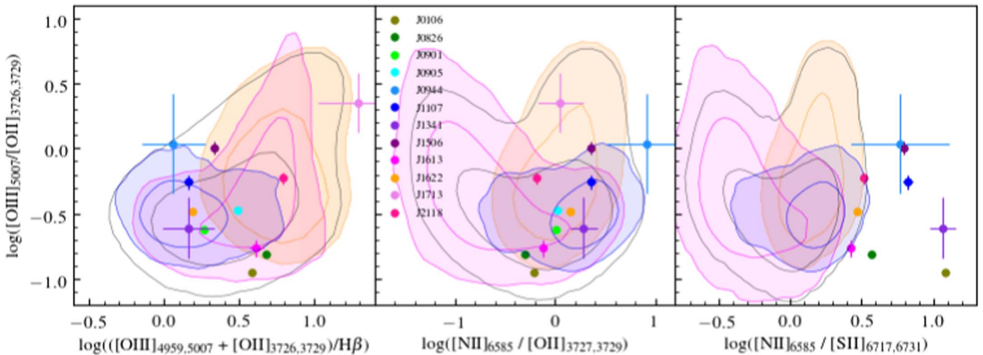
Figure 8. The ionization-sensitive ratio O32 ( [\text{O III}]\lambda 5007/[\text{O II}]\lambda\lambda 3726,3729 ), plotted against abundance-sensitive diagnostics for our sample and the SDSS DR8 comparison sample. Light gray contours enclose 80% and 99% of the SDSS galaxies, while blue and magenta contours enclose 80% and 99% of the high ( M_* > 10^{10.52} M_\odot ) and low ( M_* < 10^{9.25} M_\odot ) mass star-forming SDSS galaxies, respectively. The yellow contours illustrate the location of 80%, and 99% of the SDSS AGN-host galaxies. Left panel: R23 ratio ( ([\text{O III}]\lambda\lambda 4959,5007 + [\text{O II}]\lambda\lambda 3726,3729)/\text{H}\beta ; Pagel et al. 1979). Central panel: N2O2 ratio ( [\text{N II}]\lambda 6585/[\text{O II}]\lambda\lambda 3726,3729 ; Evans & Dopita 1985, 1986; Dopita et al. 2000). Right panel: N2S2 ratio ( [\text{N II}]\lambda 6585/[\text{S II}]\lambda\lambda 6717,6731 ; Dopita et al. 2013).
