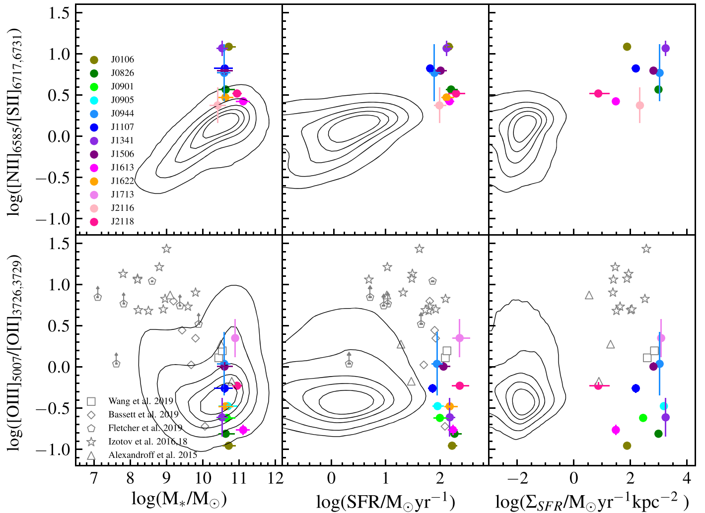
Figure 9. Top panels: total [N II] \lambda 6585 –[S II] \lambda\lambda 6717,6731 flux ratio compared to stellar mass (left), star formation rate (central), and star formation rate surface density (right). Bottom panels: total [O III] \lambda 5007 –[O II] \lambda\lambda 3726,3729 flux ratio compared to stellar mass (left), star formation rate (central), and star formation rate surface density (right). The gray contours represent SDSS DR8 data with contours at 25%, 50%, 75%, 90%, and 99%. Black empty symbols are Lyman continuum leaking galaxies: z \sim 0.3 [S II]-weak galaxies (squares; Wang et al. 2019), low-redshift Green Pea galaxies (stars; Izotov et al. 2016a, 2016b, 2018a, 2018b), low-redshift Lyman Break Analogs (triangles; Alexandroff et al. 2015, z \sim 3 star-forming galaxies (diamonds; Bassett et al. 2019), and z > 3 LACES galaxies (pentagons; Fletcher et al. 2019). Five targets from Fletcher et al. (2019) are not detected in [O II], the O32 values are 3\sigma lower limits.
