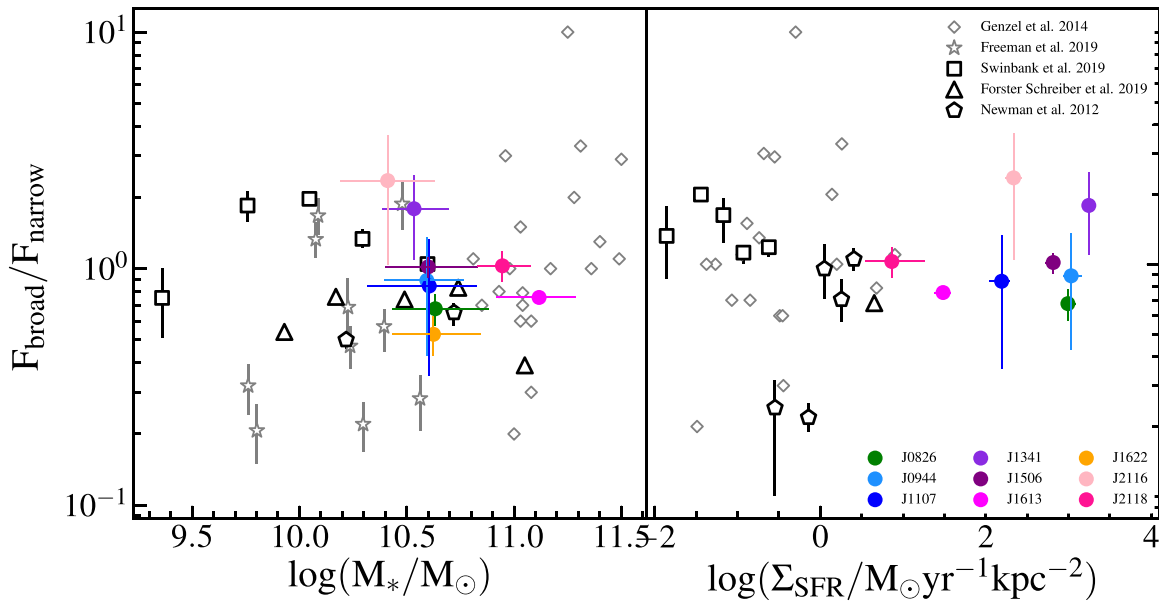
Figure 10. Broad-to-narrow H \alpha flux ratio as a function of stellar mass (left panel), and star formation surface density (right panel) for our galaxies and some relevant star-forming galaxy samples. Stars are 10 star-forming galaxies at z \sim 2 from the MOSDEF survey (Freeman et al. 2019). Squares are the galaxy average values of 529 star-forming galaxies at z \sim 1 from KMOS observations (Swinbank et al. 2019). Diamonds are 20 z = 1 - 2 galaxies from Genzel et al. (2014). Pentagons are stacks of 27 z \sim 2 star-forming galaxies from the SINS and zC-SINF surveys (Newman et al. 2012). Triangles are stacks of 78 (left panel) and 33 (right panel) star-forming galaxies at 0.6 < z < 2.7 from the KMOS3D survey (Förster Schreiber et al. 2019).
