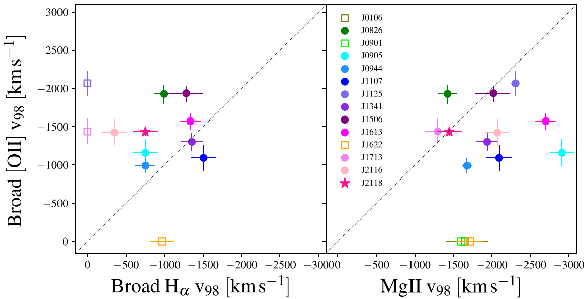
Figure 4. Broad [O II] emission line kinematics compared to broad H\alpha emission line (left), and Mg II absorption line (right) ones as represented by the maximum measured velocity v_{98} . Errors on v_{98} due to uncertainties in the fits are estimated varying the best-fit parameters in a range of \pm 1\sigma and measuring the resulting change in v_{98} . The dotted lines represent the one-to-one relation. The galaxies that have no broad [O II] or H\alpha emission lines detected are shown as empty squares. For J0905 v_{98} is derived from the H\beta broad emission line instead of the H\alpha . For J2118 v_{98} is derived from the Fe II \lambda 2586 absorption line profile instead of the Mg II \lambda 2796 , since Mg II absorption is not detected for this galaxy. Most of the objects in our sample exhibit broad [O II] maximum velocities comparable to those derived from the broad H\alpha and Mg II absorption lines.
