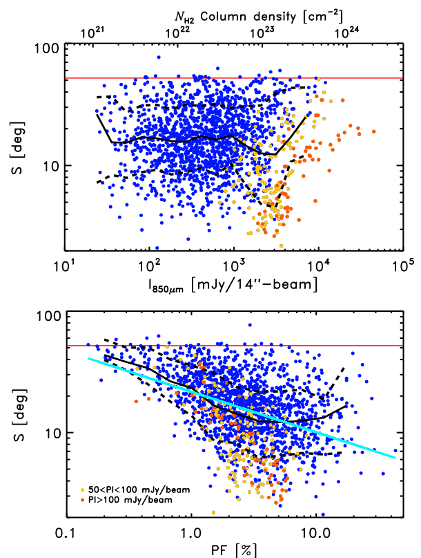
Fig. 9. Scatter plot of S (dispersion function of \chi_{B_{\text{pos}}} ) as a function of I ( top ) and PF ( bottom ) for data points with SNR(I) > 25 and SNR(PI) > 3 (c.f., Fig. 7). The data points with 50 < PI < 100 mJy/beam and PI > 100 mJy/beam are shown in yellow and red, respectively. The black solid curves show the median \log(S) per bin of \log(I) and \log(PF) in the top and bottom panels, respectively. The lower and the upper dashed black lines are the 16% and 84% percentiles of the distributions, respectively. The red horizontal line at S = 52^\circ shows the value that S would take for a B-field dominated by turbulence. In the bottom panel, the cyan solid line is a linear fit to the distribution.
