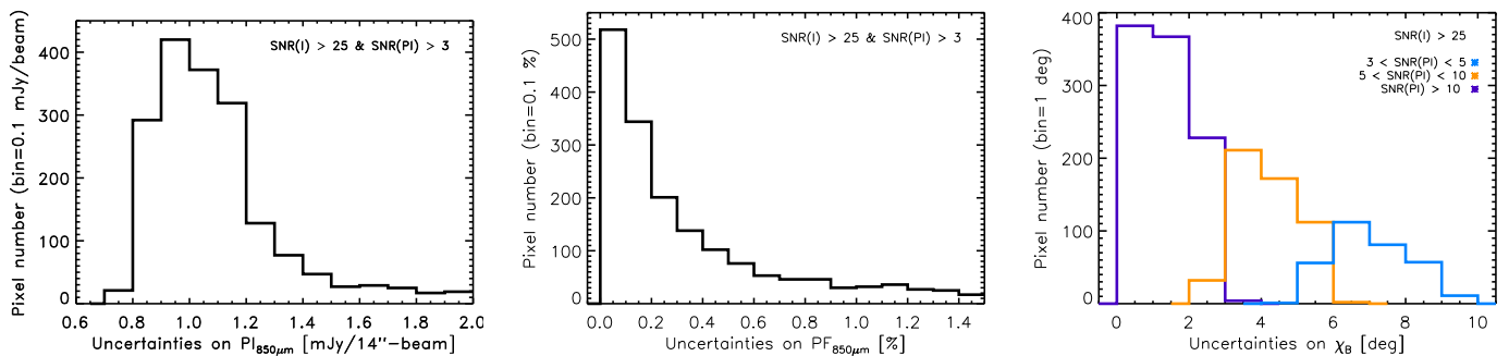
Fig. A.5. Distributions of the uncertainties on PI (left), PF (middle), and \chi_{B_{\text{POS}}} (right) for SNR(I) > 25 and SNR(PI) > 3 corresponding to the maps shown in Fig. A.1. On the right hand side plot the different colors are as follow: blue for 3 < SNR(PI) < 5 , orange for 5 < SNR(PI) < 10 , and purple for SNR(PI) > 10 .
