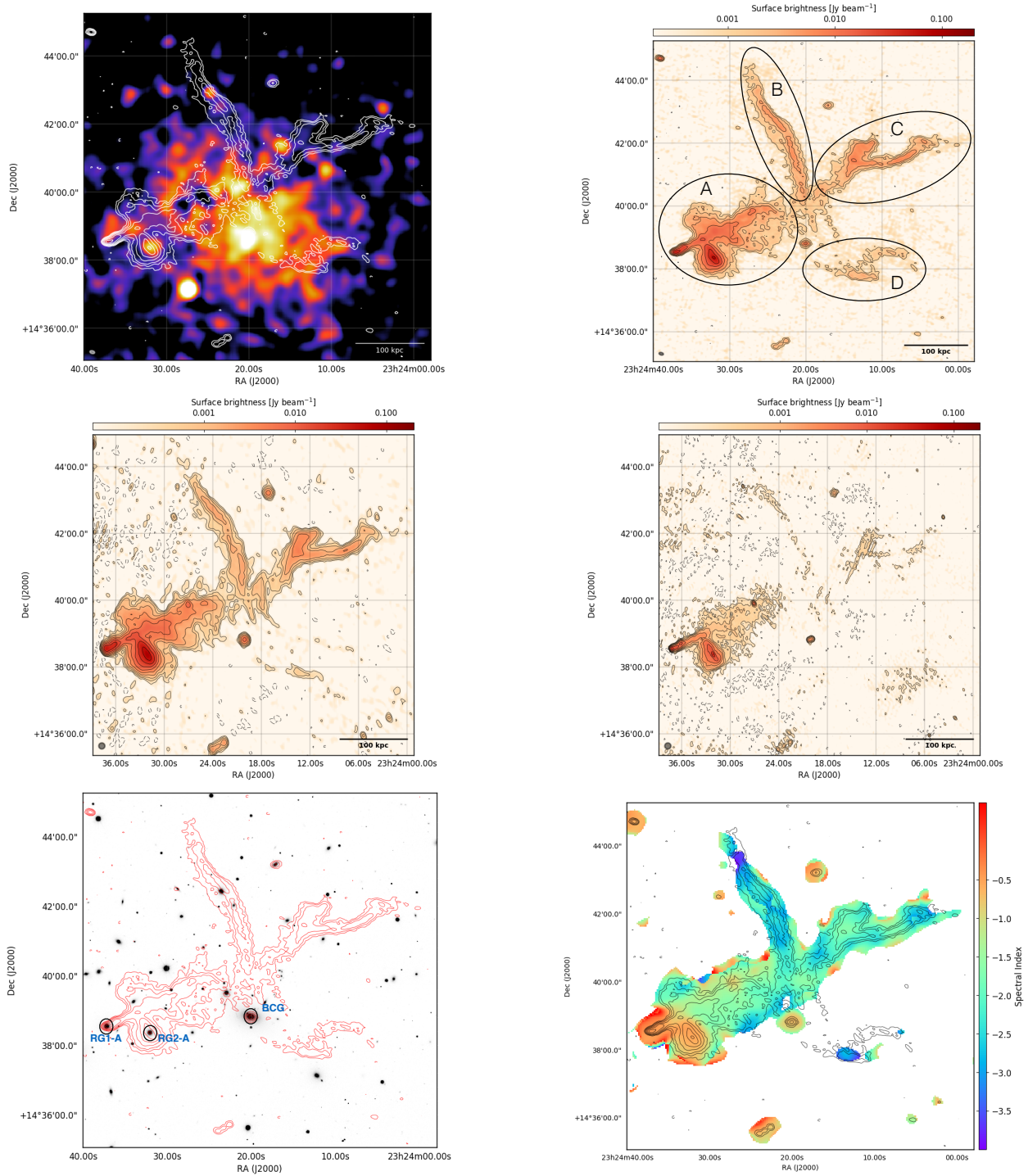
Fig. 1. Top left panel: Full-resolution LOFAR image contours (white; as shown in the right panel ) of Abell 2593, overlaid on an exposure-corrected Chandra image in the 0.5–2.0 keV energy band with a total integration time of 7ks. Top right panel: The 150 MHz LOFAR image ( 9'' \times 6'' ) where the black contours and dashed lines show the (1, 2, 4, \dots) \times 5 \times \sigma_{\text{LOFAR}150} and -3 \times \sigma_{\text{LOFAR}150} levels respectively, where \sigma_{\text{LOFAR}150} = 219 \mu\text{Jy}/\text{beam} . Middle left panel: The 325 MHz GMRT image ( 11'' \times 7'' ) where the black contours and dashed lines show the (1, 2, 4, \dots) \times 5 \times \sigma_{\text{GMRT}325} and -3 \times \sigma_{\text{GMRT}325} levels respectively, where \sigma_{\text{GMRT}325} = 66 \mu\text{Jy}/\text{beam} . Middle right panel: The 610 MHz GMRT image ( 5'' \times 4'' ) where the black contours and dashed lines show the (1, 2, 4, \dots) \times 5 \times \sigma_{\text{GMRT}610} and -3 \times \sigma_{\text{GMRT}610} levels respectively, where \sigma_{\text{GMRT}610} = 38 \mu\text{Jy}/\text{beam} . Bottom left panel: LOFAR 150 MHz contours as shown in the top left panel in red overlaid on an SDSS r-band image of Abell 2593. The marked galaxies (RG1-A and RG2-A) are the possible counterparts for the radio emission of regions A and C. The BCG mark indicates the brightest cluster galaxy. Bottom right panel: The LOFAR 150 MHz contours as shown in the top right panel overlaid on the high resolution ( 20'' \times 20'' ) spectral index map of Abell 2593.
