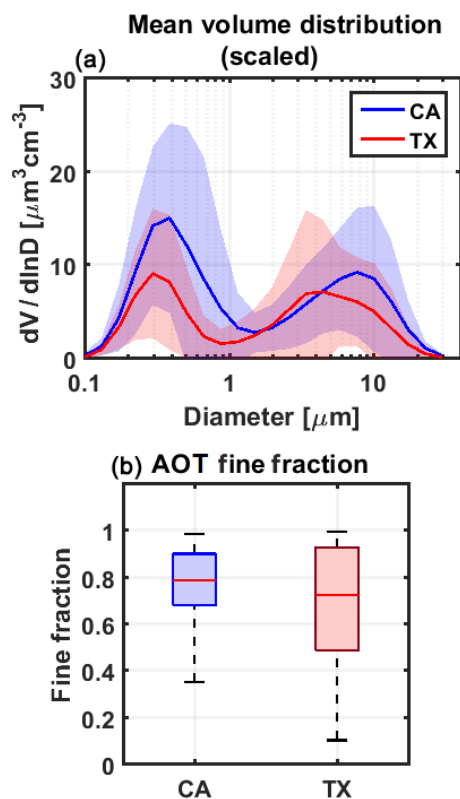
Figure 11. (a) Mean volume distribution retrieved from AERONET/DRAGON sun photometer measurements, scaled to a maximum aerosol layer height of 1 km for CA and 3 km for Texas. (b) Statistics for the AERONET/DRAGON aerosol optical depth fine fraction.
