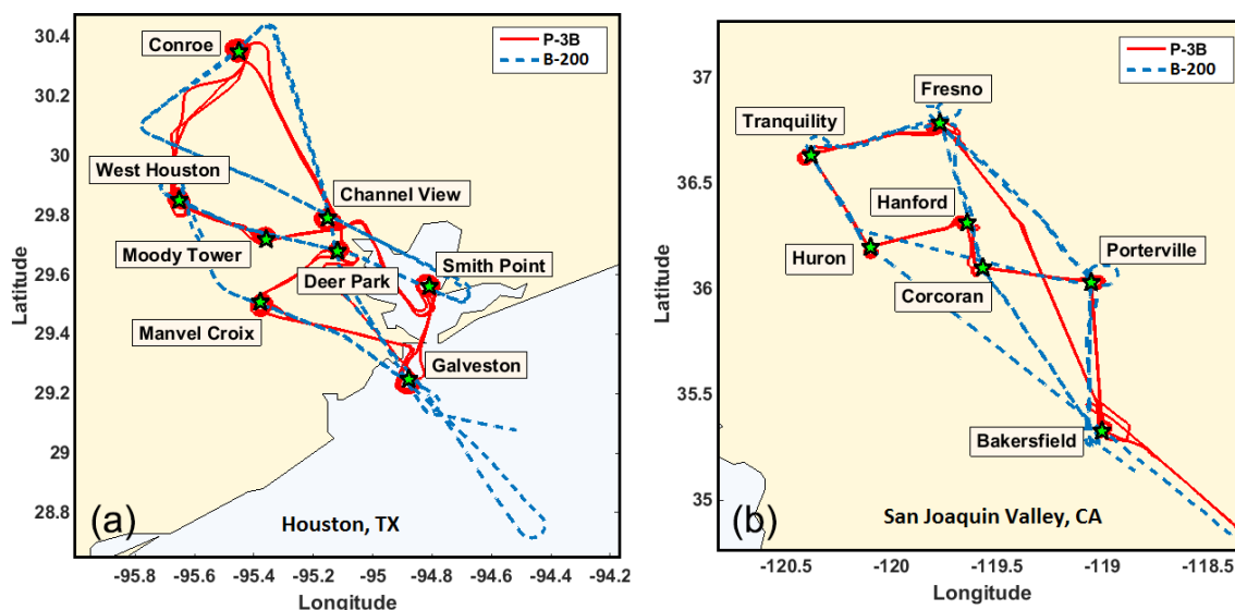
Figure 1. Map of the flight tracks for DISCOVER-AQ field campaign (DAQ) California (b) and DAQ Texas (a). The green stars mark the location of the ground stations over which the P3B (red solid line) spiraled. The HSRL-2 instrument onboard the King Air (blue dashed line) flew over the same ground stations.
