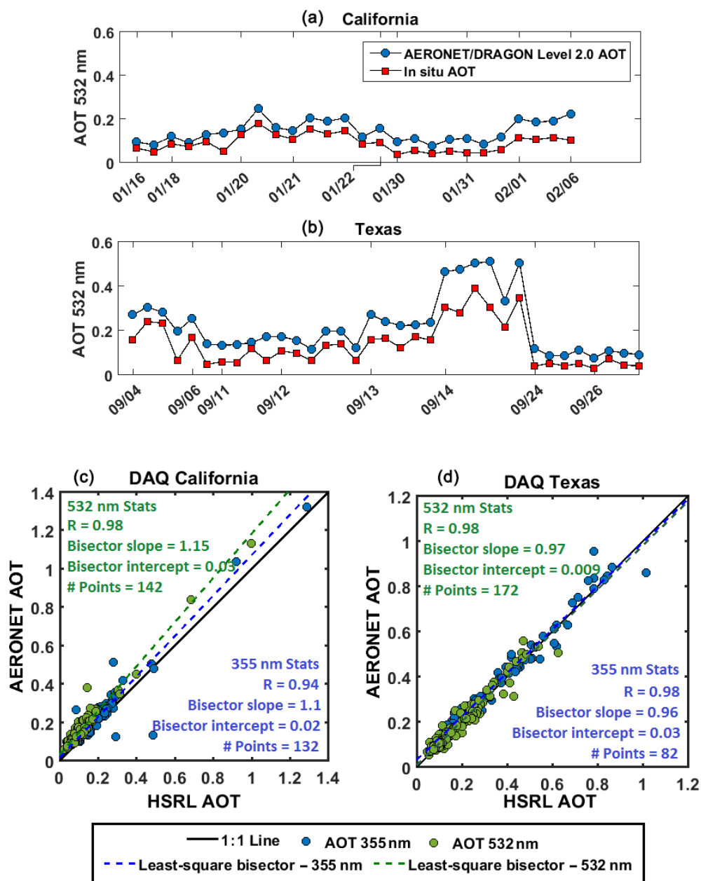
Figure 10. (a, b) AERONET and in situ aerosol optical thickness (AOT) measurements during DAQ CA (a) and TX (b). In situ values were obtained by vertical integration of the ambient extinction profile. (c, d) Comparison of AOT measurements at 355 and 532 nm measured with HSRL-2 and AERONET/DRAGON sun photometers during DAQ California (c) and DAQ Texas (d). Measurements from AERONET were calculated from level 2.0 measurements of AOT at 340 and 500 nm, corrected to 355 and 532 nm using Ångström exponents calculated between 340 and 440 nm, and 440 and 675 nm, respectively. Only measurements obtained within a radius of 2.5 km and 10 min from each other were considered.
