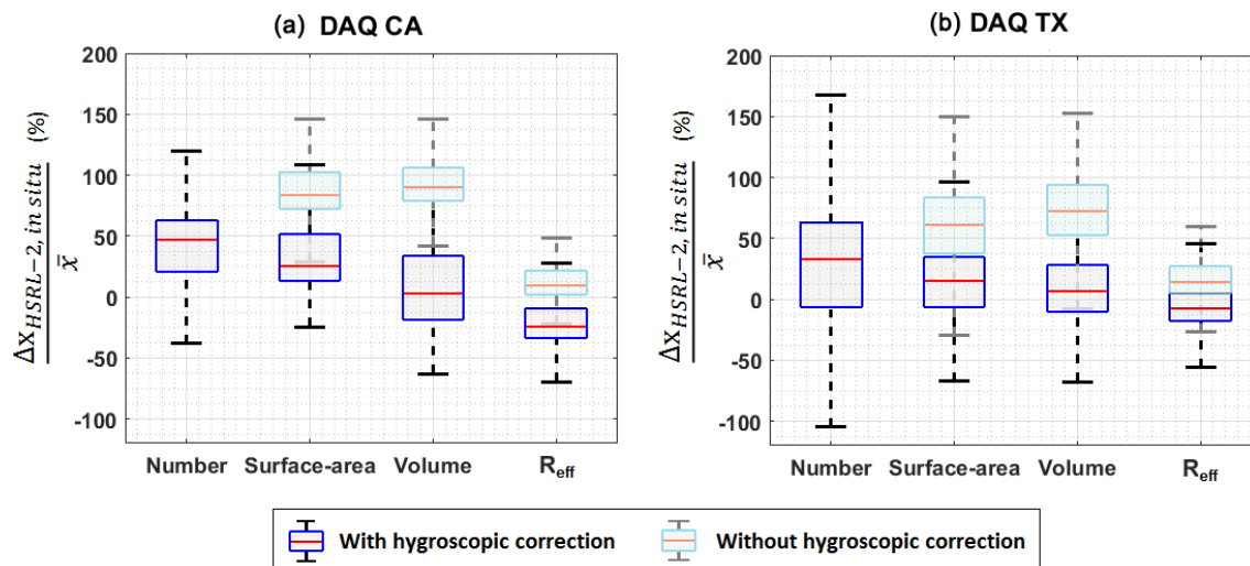
Figure 7. Statistics of the comparison between the HSRL-2 retrievals and the in situ measurements of number, surface-area, and volume concentrations, and effective radii for DAQ CA (a) and DAQ TX (b) with and without the hygroscopic correction applied to the in situ measurements (fine-mode only). The box plots represent the distribution of the biases observed between the HSRL-2 retrievals and the in situ measurements for each parameter. The relative bias was calculated as the ratio of the difference between HSRL-2 retrievals and the in situ measurements ( \Delta x ) to the average between the HSRL-2 retrievals and the in situ measurements ( \bar{x} ). The red line represents the median value, the boxes edges represent the 25th and 75th percentiles ( q_1 , q_3 , respectively), and the whiskers represent the outlier boundaries ( q_1 - 1.5 \times \text{IQR} ) and ( q_3 + 1.5 \times \text{IQR} ), where \text{IQR} = q_3 - q_1 .
