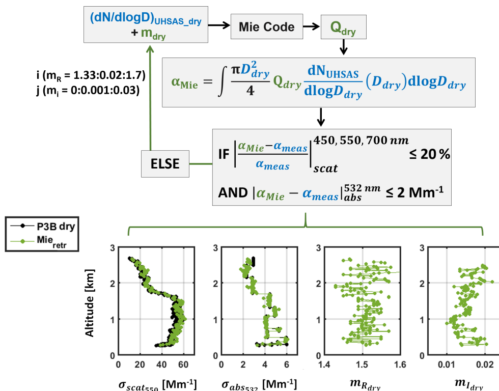
Figure 2. Diagram representation of part I in which the dry complex refractive index pairs ( m_{Rdry} , m_{Idry} ) are retrieved from the in situ measurements. UHSAS measurements of size distributions are obtained for particles with D < 1 \mu\text{m} while the scattering and absorption measurements were obtained for particles with D < 5 \mu\text{m} . The blue terms in the block diagram refer to measured quantities. Q_{dry} refers to the scattering or absorption efficiencies calculated with the Mie code. The profiles shown at the bottom of this figure were obtained over Channel View, Houston, TX on 11 September 2013 between 21:06 and 21:15 UTC, during DAQ TX. The plots show the comparison between the in situ measurements (“P3B dry” in black) and the retrieved (“Mie retr ”) dry scattering at 550 nm ( \sigma_{scat550} ), and absorption at 532 nm ( \sigma_{abs532} ) obtained with the complex refractive index retrieved in this step.
