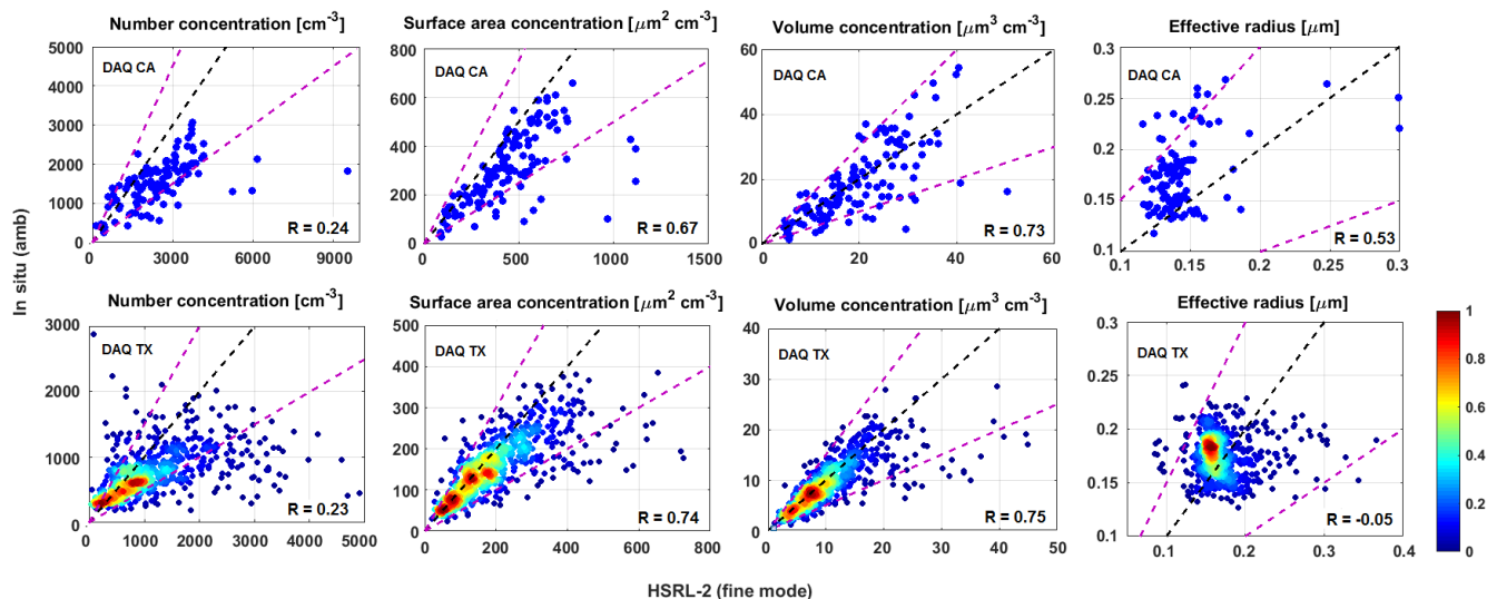
Figure 6. Comparison of number, surface-area and volume concentrations, and effective radius (fine mode only) for all coincident points between HSRL-2 ( x axis) and in situ (corrected for ambient RH; y axis) obtained during DAQ CA and TX. The black dashed lines represent 1 : 1 and the magenta dashed lines represent \pm 50\% . R values correspond to correlation coefficients. There are 126 points in the DAQ CA plots and 630 data points in the DAQ TX plots. For the latter, due to the large number of overlapping points, the scatter plot is color-coded by the density of points. The colorbar is normalized to 1.
