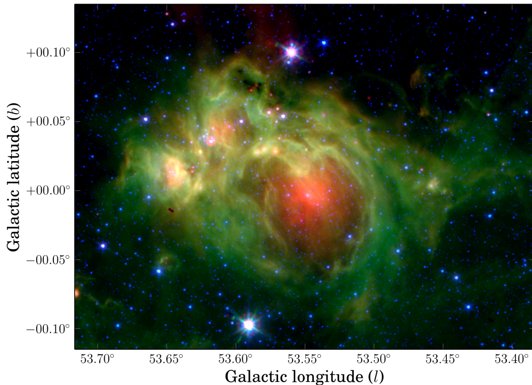
Figure 19. Star-forming region Sh 2-82 as seen in the mid-infrared by the Spitzer Space Telescope. The mosaic is composed of the 24 \mu\text{m} (red), 8.0 \mu\text{m} (green) and 4.5 \mu\text{m} (blue) bands. The image reveals a bubble-shaped structure which surrounds the HII region that is seen in the IPHAS mosaic which spans the same region (Fig. 18). This structure has previously been labelled as N115 in the catalogue of Churchwell et al. (2006), and could be a possible site of triggered star formation (Thompson et al. 2012; Kendrew et al. 2012).
