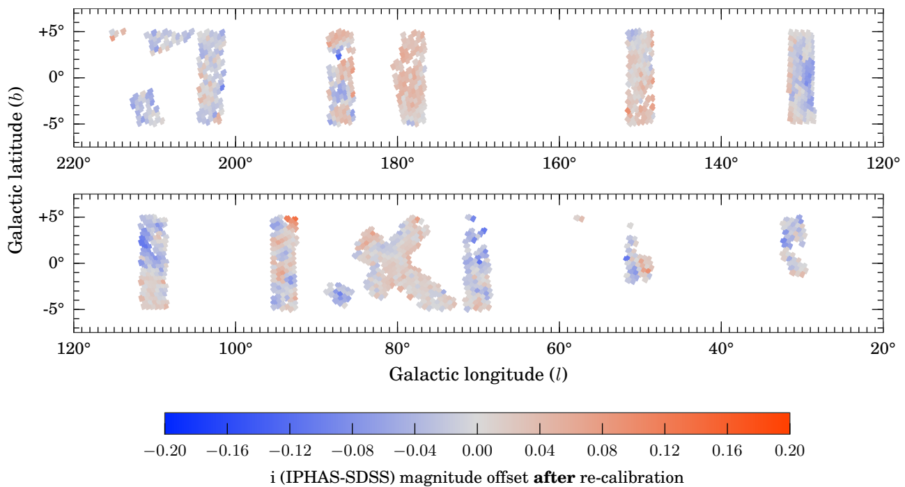
Figure 10. Same as Fig. 9 for the i -band.
