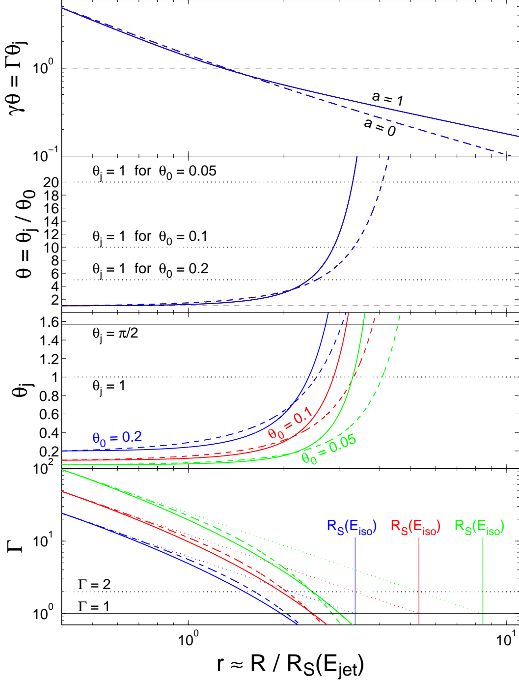
Fig. 3.— Similar to Fig. 2 but only for a uniform external density ( k = 0 ) and for three different values of the initial jet half-opening angle: \theta_0 = 0.05 ( green ), \theta_0 = 0.1 ( red ) and \theta_0 = 0.2 ( blue ). The old ( a = 0 ) and new ( a = 1 ) recipes for the jet lateral expansion are shown by dashed and solid lines, respectively. In the top two panels the lines for different \theta_0 and the same a values coincide (see text for details). The values of R_S(E_{\text{iso}}) are indicated in the bottom panel for reference.
