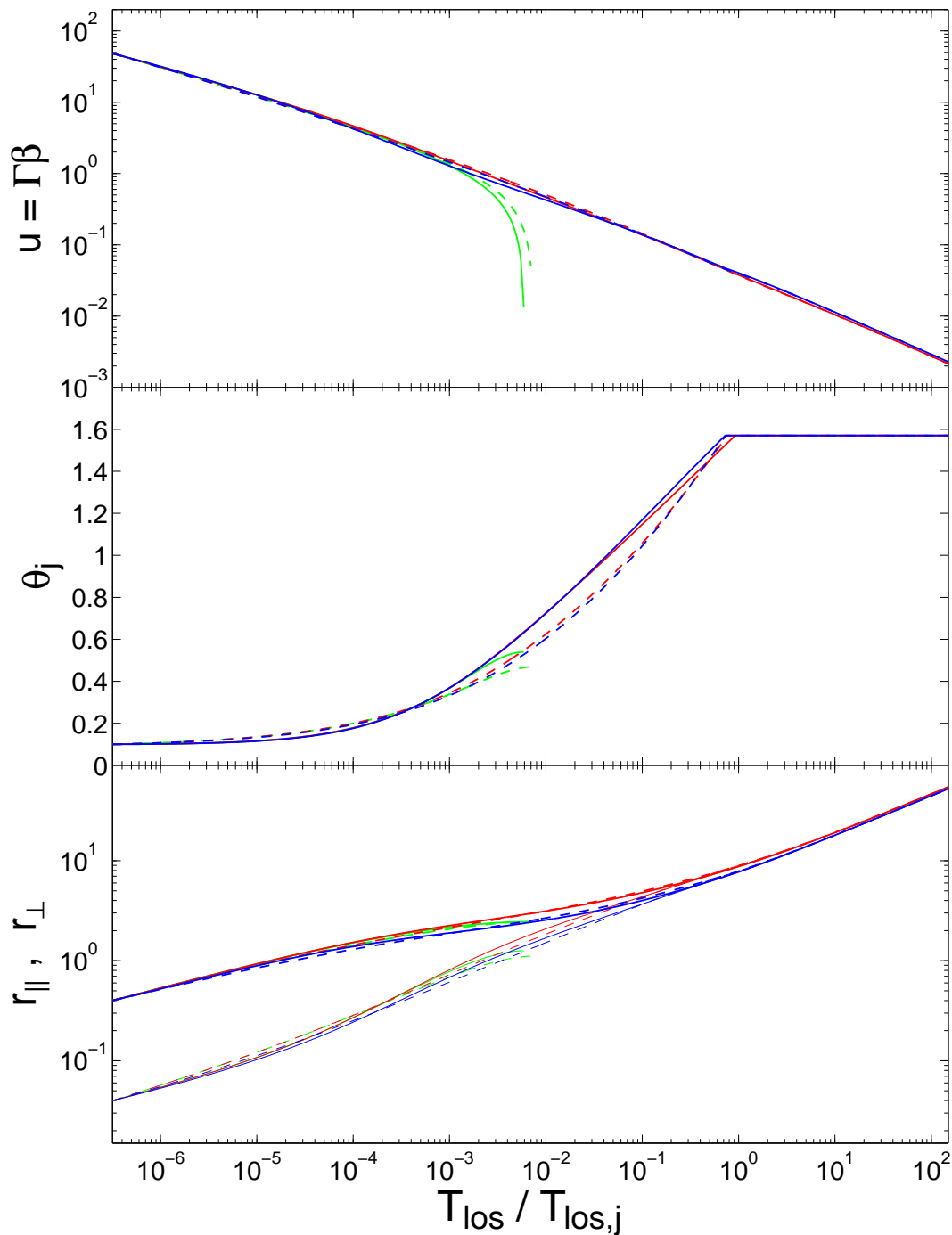
Fig. 10.— Similar to Fig. 9 but as a function of the observed time, T_{\text{los}} , at which photons from the front of the jet reach an observer located along its symmetry axis, normalized by its value at the jet break time T_{\text{los},j} .
