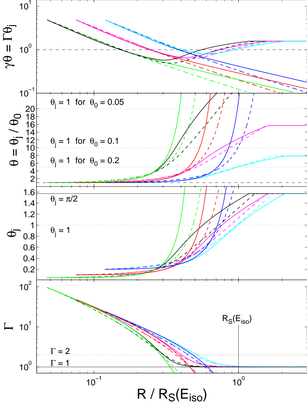
Fig. 7.— Similar to Fig. 6 but shown (1) only for our relativistic model ( green, red, and blue lines for \theta_0 = 0.05, 0.1, and 0.2, respectively) and trumpet model ( black, magenta, and cyan lines for \theta_0 = 0.05, 0.1, and 0.2, respectively), (2) for both the old recipe ( a = 0 ; dashed lines ) and our new recipe ( a = 1 ; solid lines ) for the jet lateral expansion, and (3) as a function of the jet radius R normalized by R_S(E_{\text{iso}}) = R_j \theta_0^{-2/(3-k)} instead of of [(3-k)/2]^{-1/(3-k)} R_j = [(3-k)/4]^{-1/(3-k)} R_S(E_{\text{jet}}).
