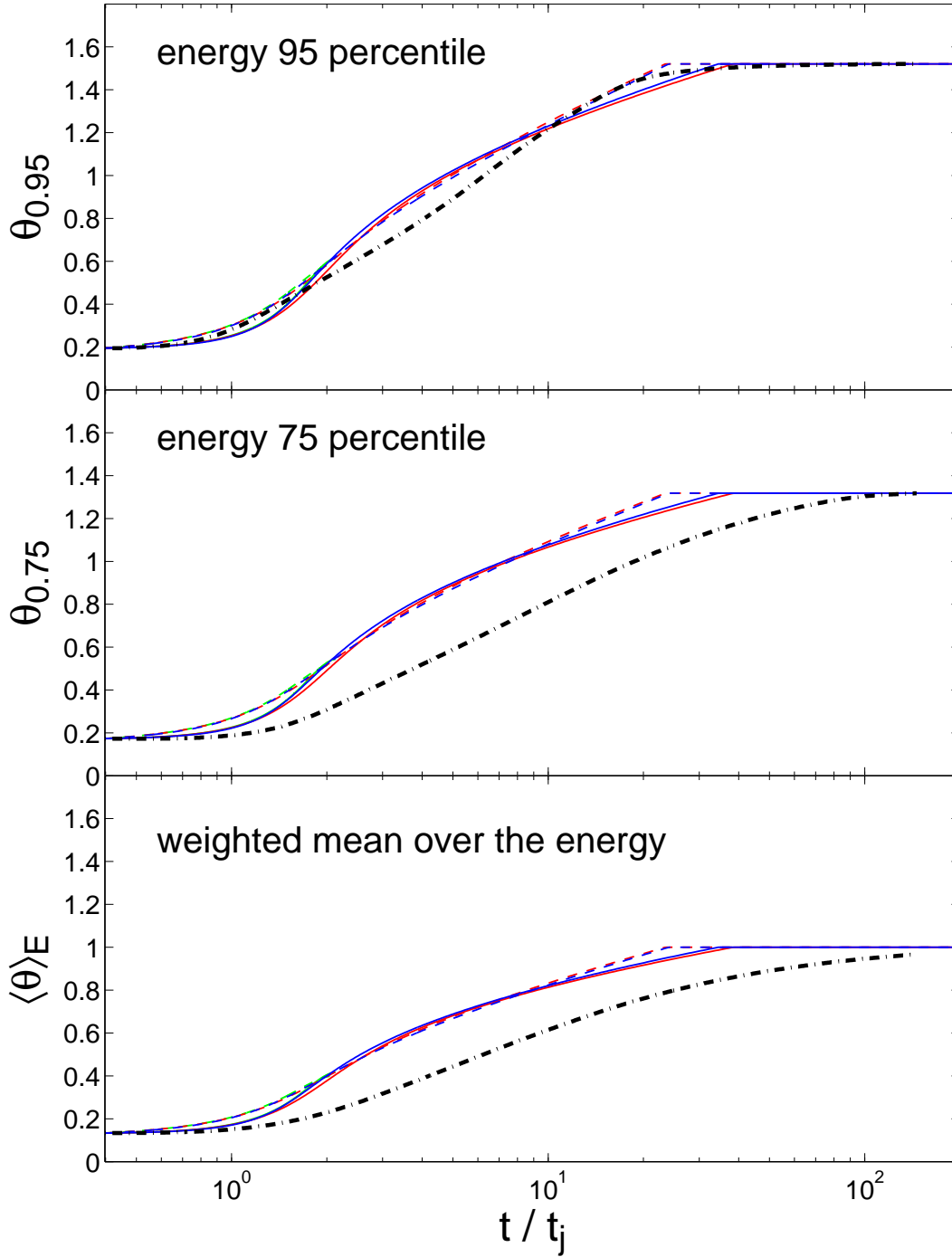
Fig. 12.— Similar to Fig. 11 but for three different ways of quantifying the jet half-opening angle, \theta_j . The top panel and middle panel show two different energy percentiles, \theta_{0.95} and \theta_{0.75} , respectively, i.e. the values of \theta up to which 95% and 75% of the energy is contained. The bottom panel shows the weighted mean over the energy, \langle \theta \rangle_E .
