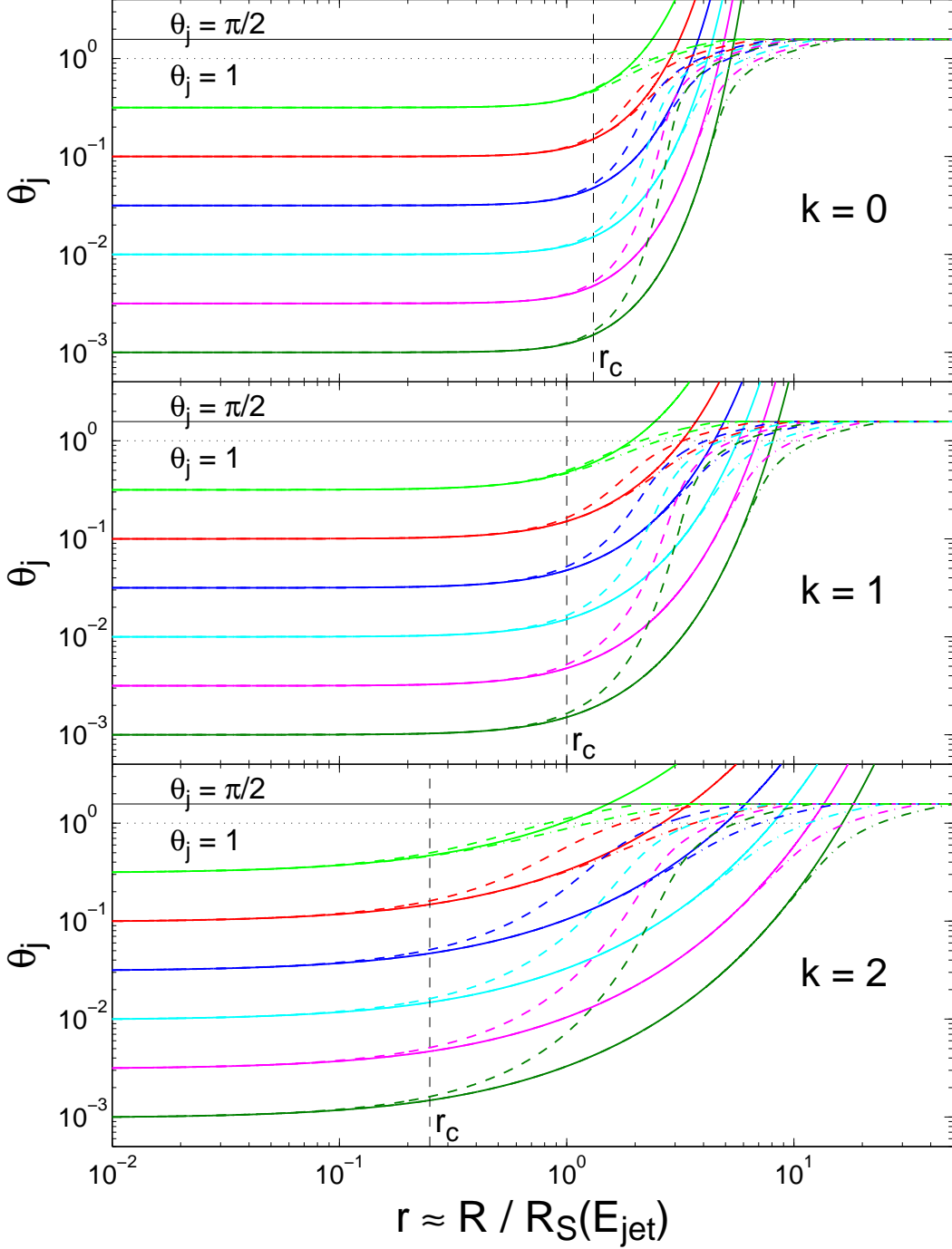
Fig. 8.— Comparison between our relativistic ( solid lines ), trumpet ( dot-dashed lines ) and conical ( dashed lines ) models in terms of the evolution of the jet half-opening angle \theta_j with the normalized radius r , for k = 0, 1, 2 ( top to bottom panels ), where all models use our new recipe for the lateral spreading of the jet ( a = 1 ). Results are shown for \log_{10}(\theta_0) = -3, -2.5, \dots, -0.5 ( using different colors ) while the values of \theta_0 = 1, \pi/2 and the critical radius r_c (given by Eq. [20], where the lateral spreading is expected to become significant) are shown for reference.
