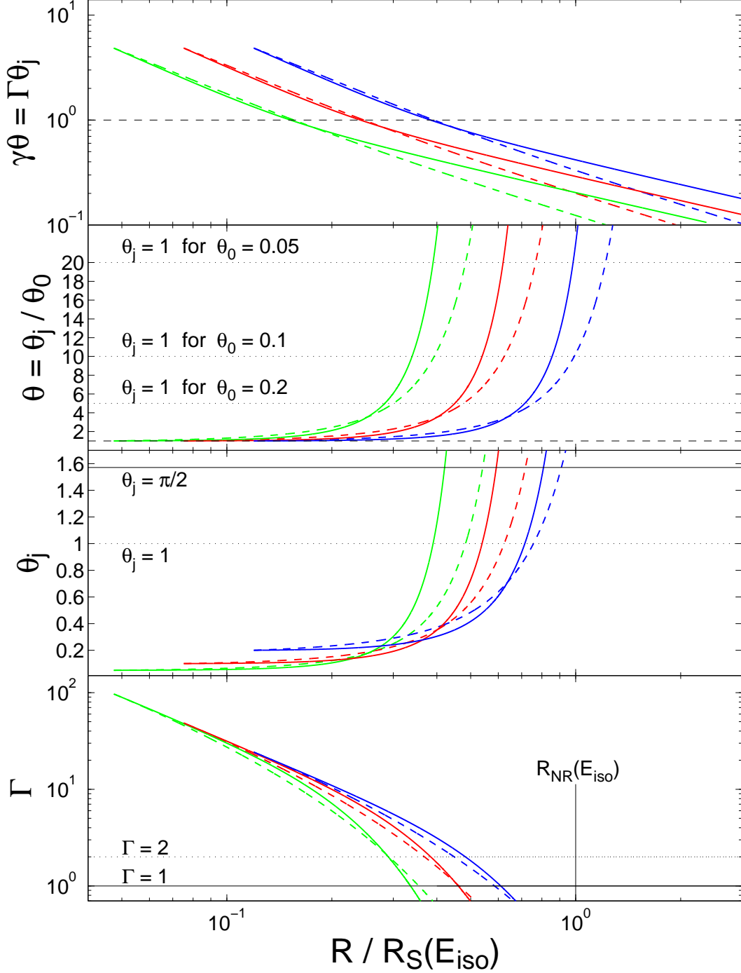
Fig. 4.— Similar to Fig. 3 but shown as a function of the jet radius R normalized by R_S(E_{\text{iso}}) = R_j \theta_0^{-2/(3-k)} instead of of [(3-k)/2]^{-1/(3-k)} R_j = [(3-k)/4]^{-1/(3-k)} R_S(E_{\text{jet}}) , where E_{\text{iso}} \approx E_{\text{jet}} 2/\theta_0^2 is the isotropic equivalent energy in the jet, while E_{\text{jet}} is its true energy.
