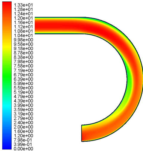
6c). RSM. Cells: 2.8 Million.
