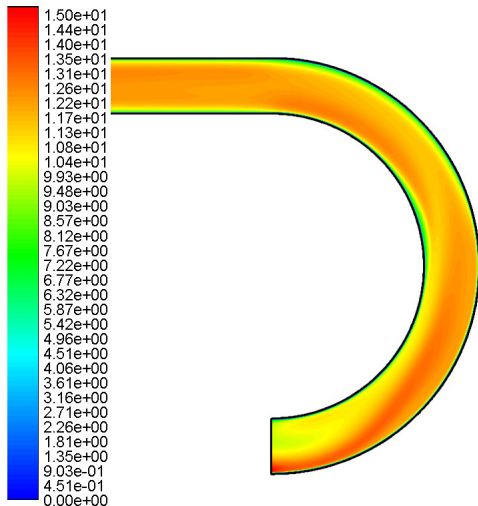
6e). k-\epsilon RNG. Cells: 2.8
