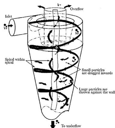
Figure 1. Schematic showing hydrocyclone flow and operation.
