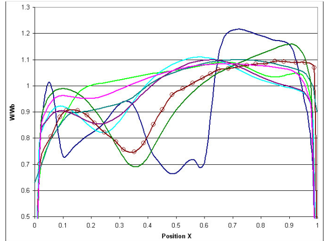
2b). Rake 2Y/D=0.25 on 90^\circ Plane
