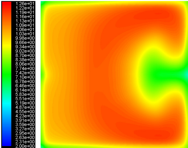
Run 1.4 5c). RSM. Cells: 2.8 Million. t=n/a
