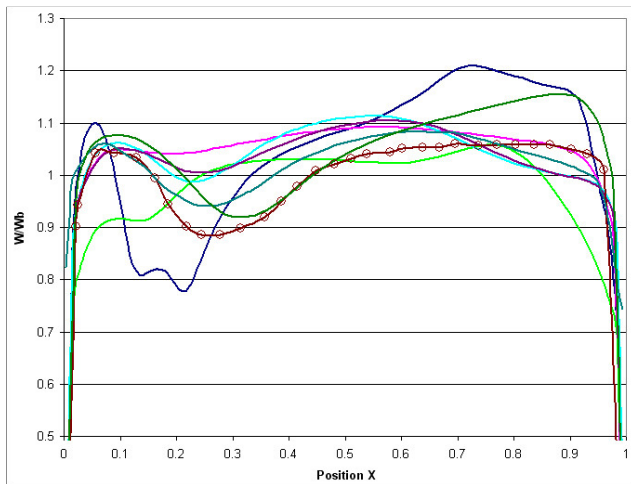
2c). Rake 2Y/D=0.5 on 90^\circ Plane
