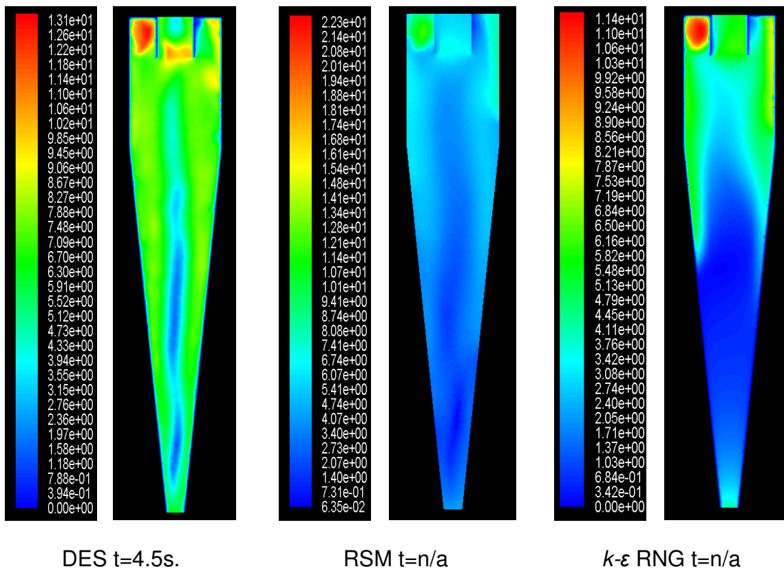
Figure 8. Contours of velocity magnitude for 10m/s Inlet with an 80/20 ratio for overflow/underflow outlets.
