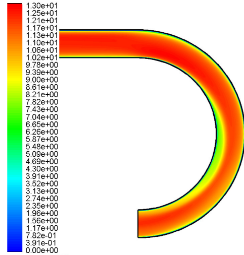
6f). k-\epsilon RNG. Cells: 0.5 Million.
