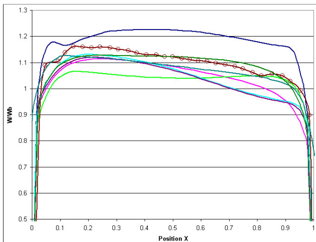
2e). Rake 2Y/D=0.875 on 90^\circ Plane
