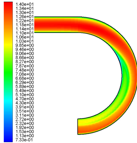
6b). DES. Cells: 0.5 Million
