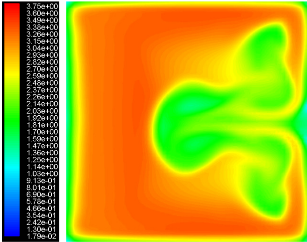
Run No 1.1 5a). DES. Cells: 2.8 Million. t=4.5s
