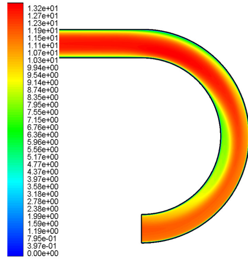
6d). RSM. Cells: 0.5 Million
