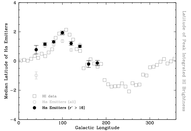
Figure 5. The median latitude as a function of longitude for all H\alpha emitters (open circles) and faint H\alpha emitters ( r' > 16 ; solid circles), compared to the peak latitude of integrated H I brightness (open squares; measured from Fig. 3 in Freudenreich et al. 1994). The signature of the Galactic warp is obvious in the H I data, and probably also be present in the H\alpha data.
