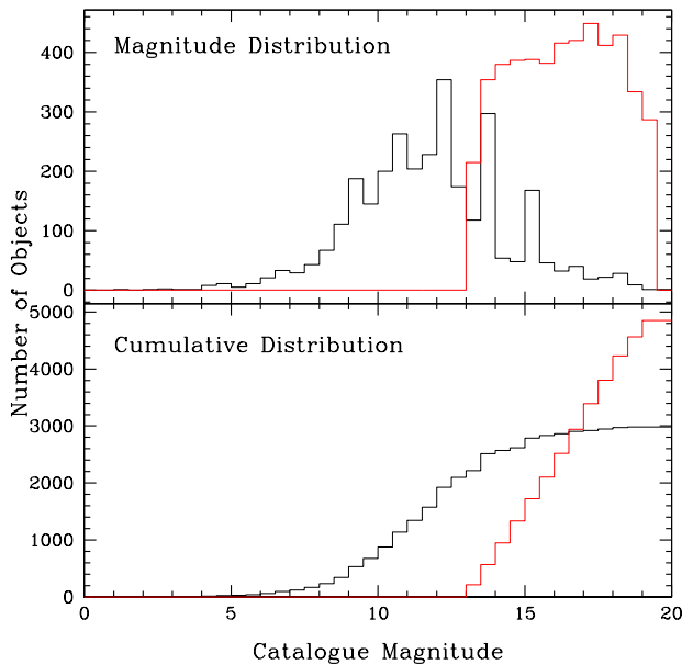
Figure 10. The magnitude distribution of the IPHAS catalogue of H\alpha emitters (red line) compared to the magnitude distribution of objects in the KW99 catalogue (black line). The IPHAS magnitudes shown correspond to the r' band, and the majority of the KW99 magnitudes correspond roughly to V band (based on either photoelectric, photographic or photovisual measurements). The top panel shows the magnitude distribution, and the bottom panel shows the cumulative distribution. All IPHAS emitters are shown here, including those flagged with 'c' in Table 1.
