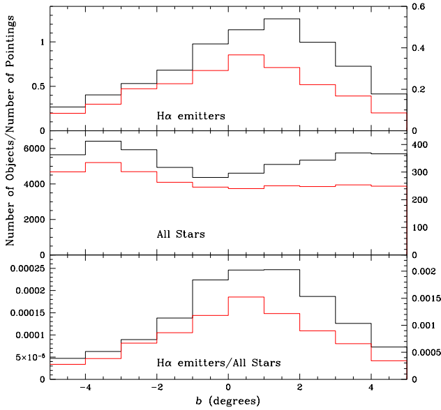
Figure 4. The distribution of H\alpha emitters in Galactic latitude. The black histograms (corresponding to the left vertical scales) show the distributions of objects irrespective of r' band magnitude. The red histograms (corresponding to the right vertical scales) show the distribution of the bright objects only ( r' \leq 15 ). The top panels show the distributions of H\alpha emitters (divided by the number of pointings in each spatial bin). The middle panels show the corresponding distributions of all stars. The bottom panels show the ratios of emitter and all-star distributions.
