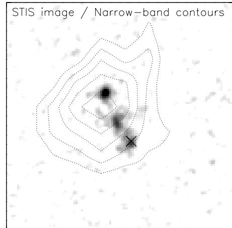
Fig. 1. A 3 \times 3 \text{ arcsec}^2 section of the STIS/CL image around the host galaxy of GRB 011211 (Jakobsson et al. 2003b). North is up and East is to the left. The GRB went off in the faint, southern part of the object (position marked with a cross). The contours show the Ly \alpha emission based on our narrow band observations. The Ly \alpha emission weighted centroid of the galaxy is close to the northern knot seen in the STIS image.
