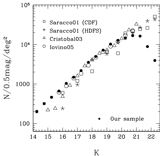
Figure 12. K -band number counts from six hours of UKIDSS DXS/UDS SV observations of a single tile in the ELAIS N1 field. Results from the literature are shown for comparison. Note that the UKIDSS number counts include both stars and galaxies.
