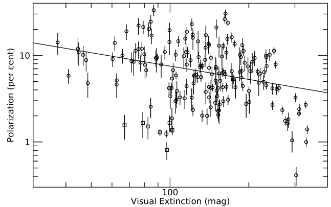
Figure 3. Relationship between the de-biased polarization fraction P and the visual extinction A_V in Perseus B1. Each point represents one of the polarization vectors from the left panel of Figure 1 that also have Herschel -derived opacity measurements. The visual extinction A_V is derived from the 300 \mu\text{m} \tau_{300} opacity map from Chen et al. (2016) assuming a reddening factor R_V = 3.1 . The figure covers a range of extinction A_V from 30 mag to 400 mag. The vertical lines show the uncertainties for the polarization fraction P . The 8 polarization vectors found towards B1-c are identified with squares. The solid line is the power-law fit (with index \beta \sim -0.5 ) between the polarization fraction P and the visual extinction A_V ( P \propto A_V^\beta , see Section 3.2).
