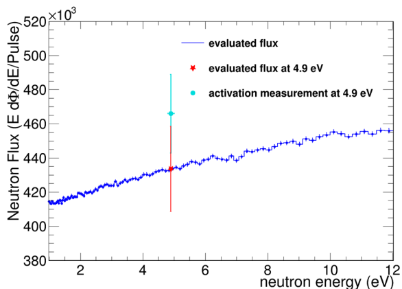
Fig. 9. Comparison of the activation measurement (cyan dot) with the value of the evaluated flux (red dot) at 4.9 eV. Results are in agreement within overall uncertainties of 5%.
