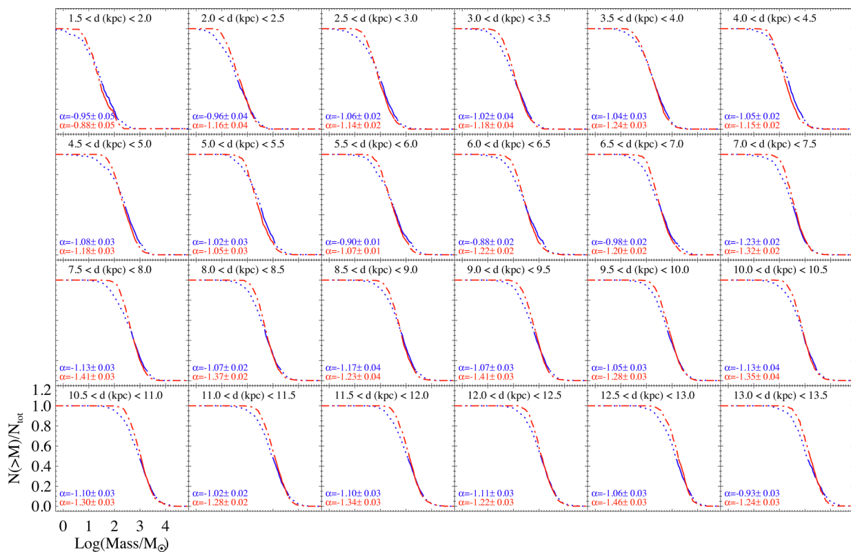
Figure 10. CClumpPMFs for pre-stellar (red dot–dashed line) and protostellar (blue dotted line) sources, obtained in the same distance ranges as used for Fig. 9. The power-law (linear in bi-logarithmic scale) portion is highlighted with solid lines, and the corresponding slope is reported in the panel with the same colour coding.
