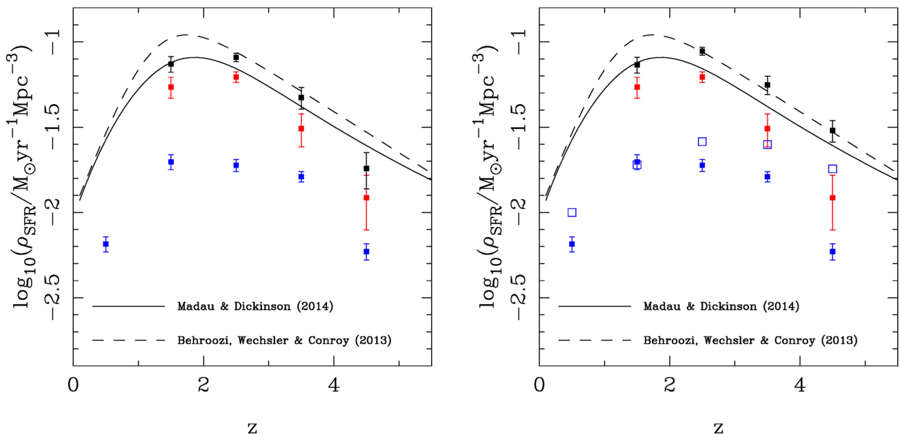
Figure 14. The cosmic evolution of comoving SFR density, \rho_{\text{SFR}} . In the left-hand panel, we plot our new ALMA-derived estimates of \rho_{\text{SFR}} (observed) (red points), estimated values of \rho_{\text{SFR}} (visible) produced by summing the raw UV-derived SFR of the galaxies in the HUDF (blue points) and the values of \rho_{\text{SFR}} (total) that result from adding these two contributions at each redshift (black points). The solid and dashed curves show two recent parametric descriptions of the evolution of \rho_{\text{SFR}} as derived from the literature by Madau & Dickinson (2014) and Behroozi, Wechsler & Conroy (2013), respectively (scaled to the IMF of Chabrier 2003). In the right-hand panel, we show the impact of including a more complete census of \rho_{\text{SFR}} (visible), based on the luminosity-weighted integral of the evolving UV galaxy luminosity function, down to M_{\text{UV}} = -15 (Parsa et al. 2016; Bouwens et al. 2015). In this panel, the values of \rho_{\text{SFR}} (observed) are unchanged, but the black points indicating \rho_{\text{SFR}} (total) now include the more complete (and, at high redshift, higher) census of \rho_{\text{SFR}} (visible), as shown by the open blue squares. At z \simeq 2 the agreement with the parametric fit provided by Behroozi et al. (2013) is excellent, and our results indicate that there is a transition from \rho_{\text{SFR}} (visible)/ \rho_{\text{SFR}} (observed) > 1 , to \rho_{\text{SFR}} (visible)/ \rho_{\text{SFR}} (observed) < 1 at z \simeq 4 .
