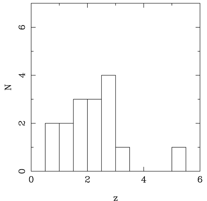
Figure 5. The redshift distribution of the 16 ALMA-detected galaxies in the HUDF. The redshift information consists of 13 spectroscopic redshifts, and three accurate ( \delta z \simeq 0.1 ) photometric redshifts, as listed in Table 2.
