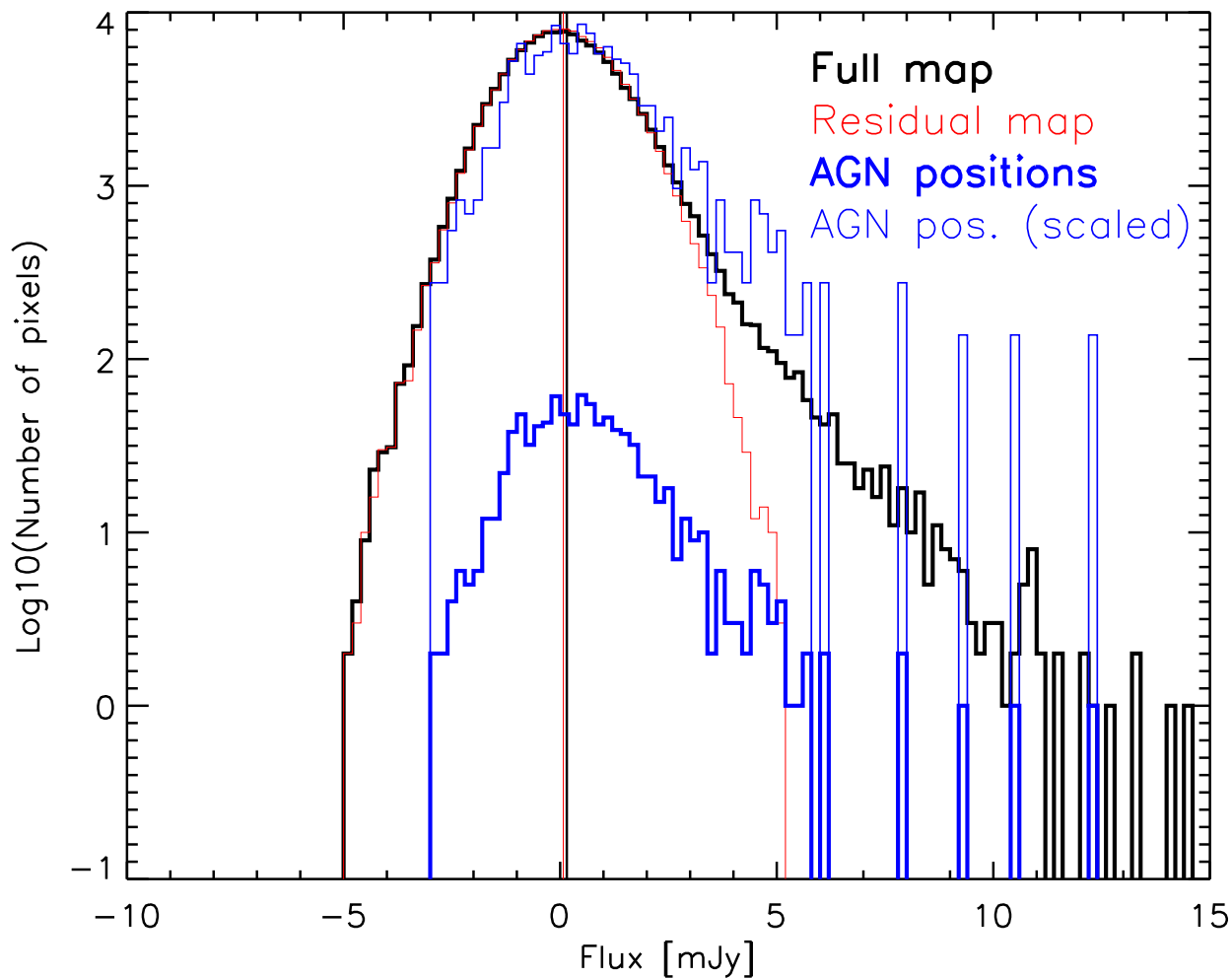
Fig. 1.— Pixel flux histograms for the roughly 80% of the LABOCA 870\mu\text{m} map of the ECDFS with RMS less or equal 1.5 times the minimum noise of 1.07\text{mJy} . The black thick histogram represents the full map, the red thin histogram the residual map after subtraction of detected sources (Weiß et al. 2009). Vertical lines indicate the mean flux of this region in the respective map. The blue thick histogram shows the flux distribution at the positions of the combined sample of 895 CDFS and ECDFS AGN. The blue thin histogram shows for easy comparison this AGN histogram scaled to the number of map pixels.
