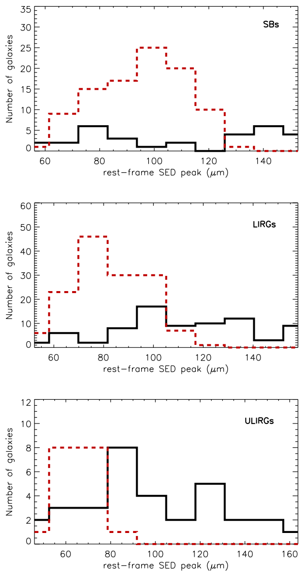
Figure 6. The distribution in SED peak for the 3 main luminosity classes (SBs, LIRGs and ULIRGs). The dotted red line represents the local sample and the solid black line represents the 70 μm sample . Although there is overlap in the distributions, a significant fraction of high redshift LIRGs and ULIRGs peak at longer wavelengths than the local galaxies of the same luminosity.
