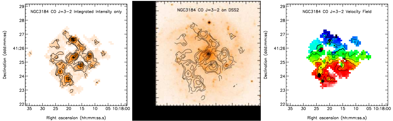
Figure C7. CO J=3-2 images for NGC 3184. (a) CO J=3-2 integrated intensity image. Contour levels are (0.5, 1, 2, 4) \text{K km s}^{-1} ( T_{MB} ). (b) CO J=3-2 integrated intensity contours overlaid on an optical image from the Digitized Sky Survey. (c) Velocity field as traced by the CO J=3-2 first moment map. Contour levels are (532, 546, 560, 574, 588, 602, 616, 630) \text{km s}^{-1} . The velocity dispersion map has been published in Wilson et al. (2011).
